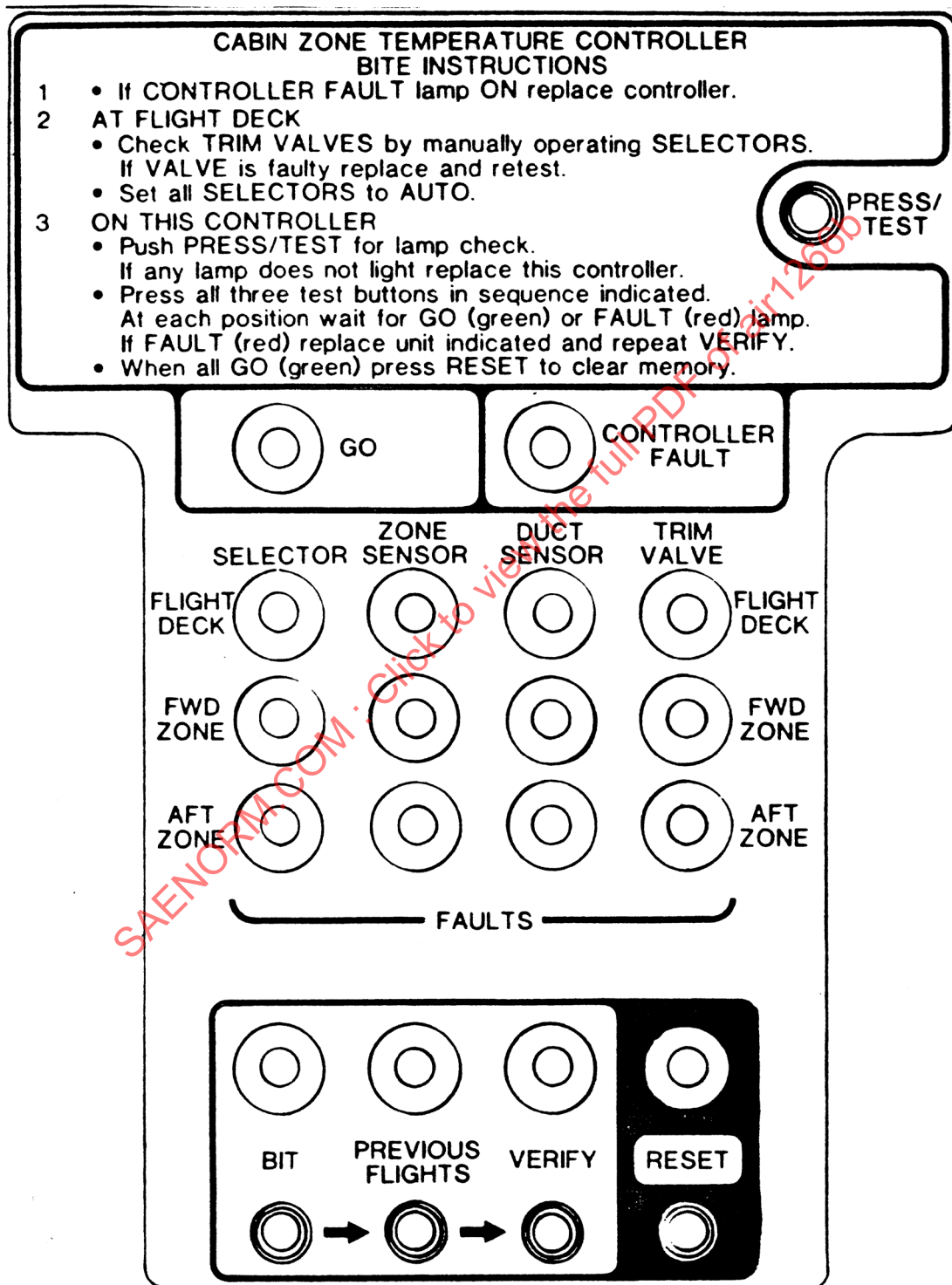
Figure 4 - Temperature controller BIT instructions
