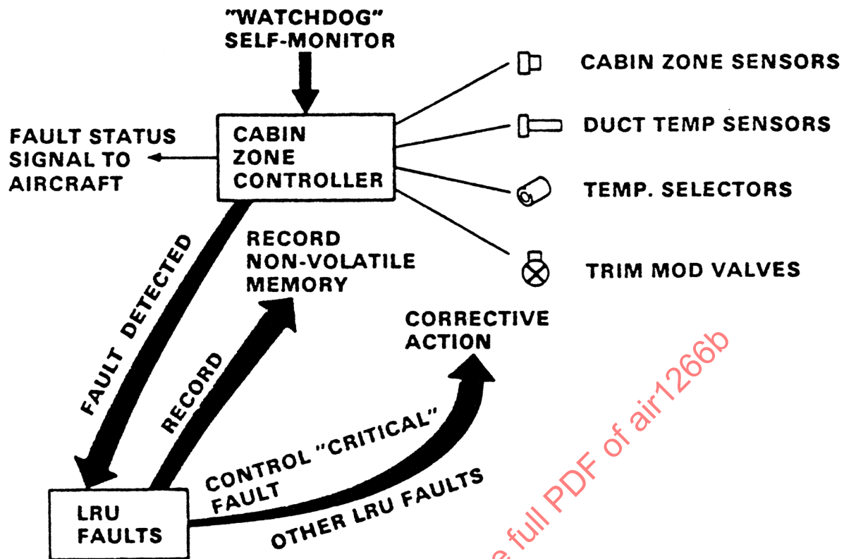
Figure 9 - BIT continuous monitoring mode cabin zone subsystem
