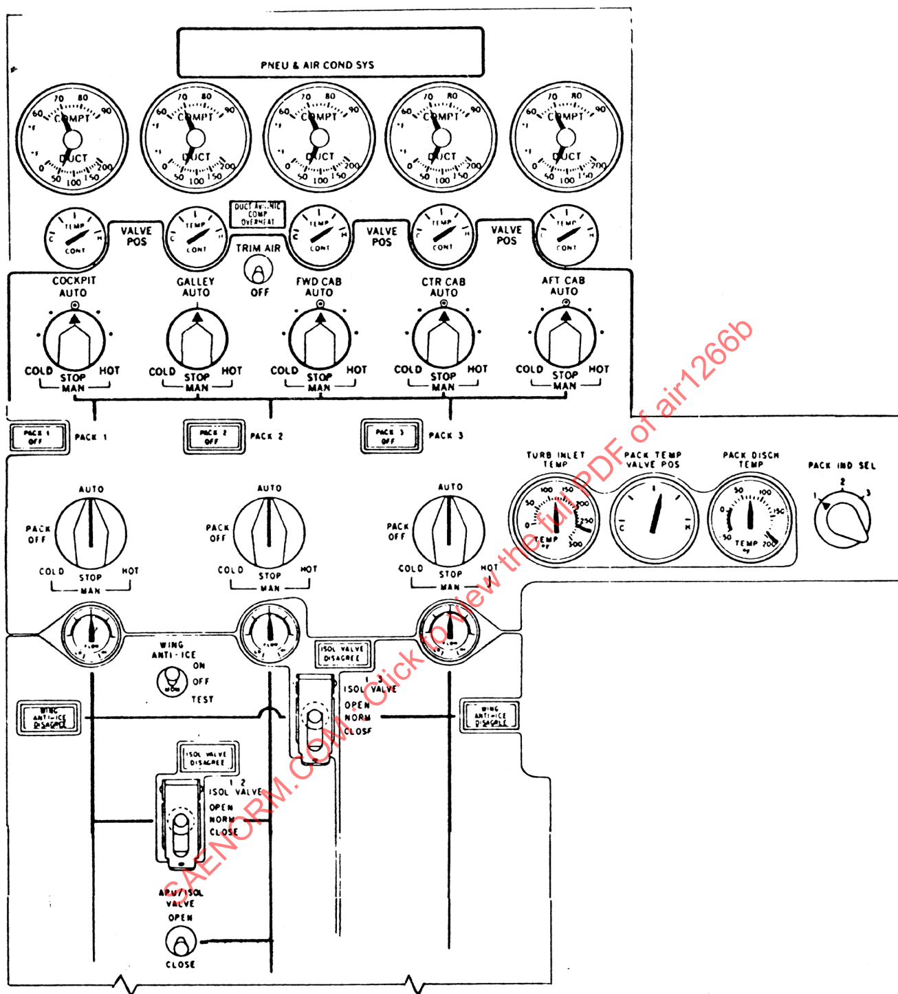
Figure 6 - Flight deck panel zone and pack temperature control
