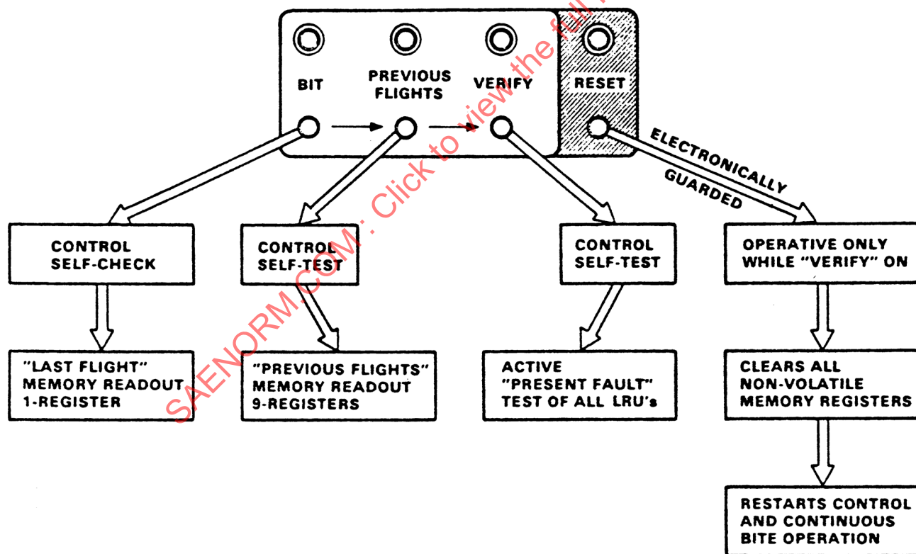
Figure 10 - BIT initiated mode pushbutton operation
