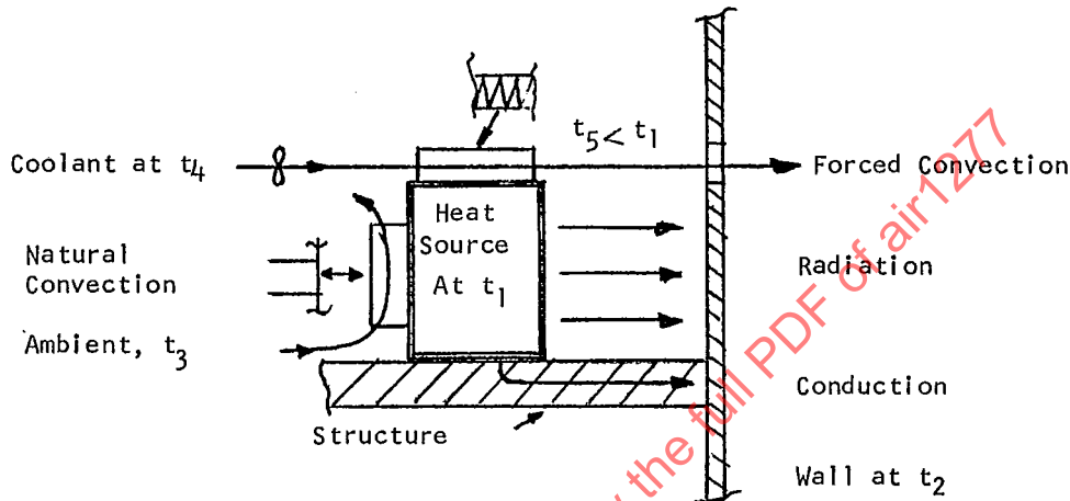
FIGURE 2. Combined Modes of Cooling
