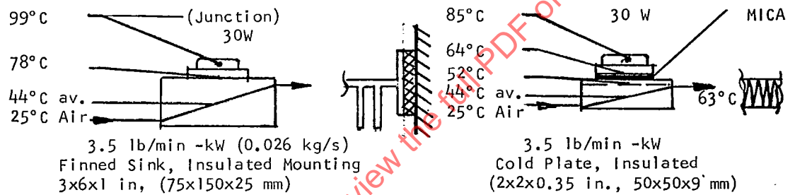
(a) EDS, Air Cooling
