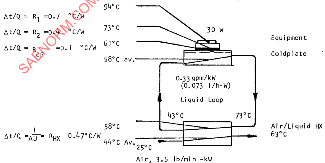
(b) Liquid loop Cooling with Air Heat Sink
