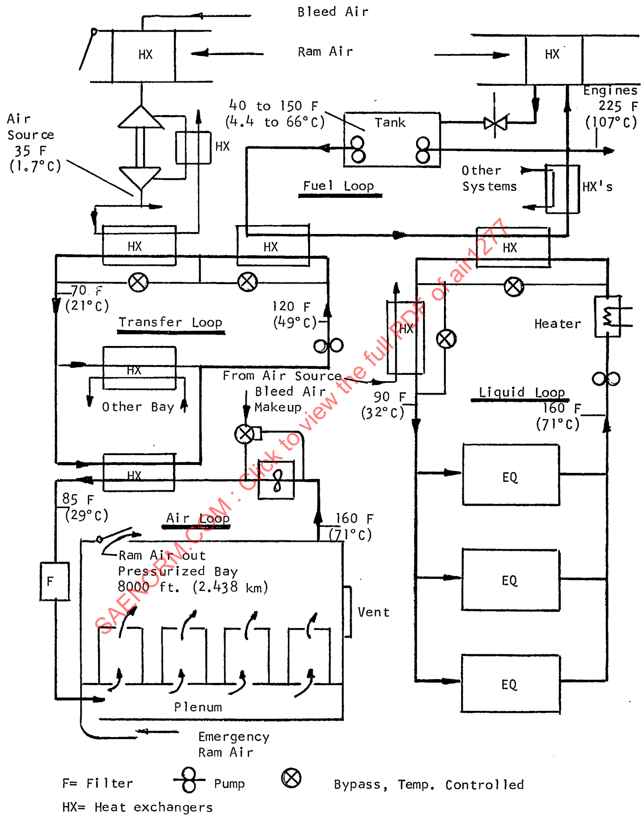
FIGURE 13. Multiloop Cooling
