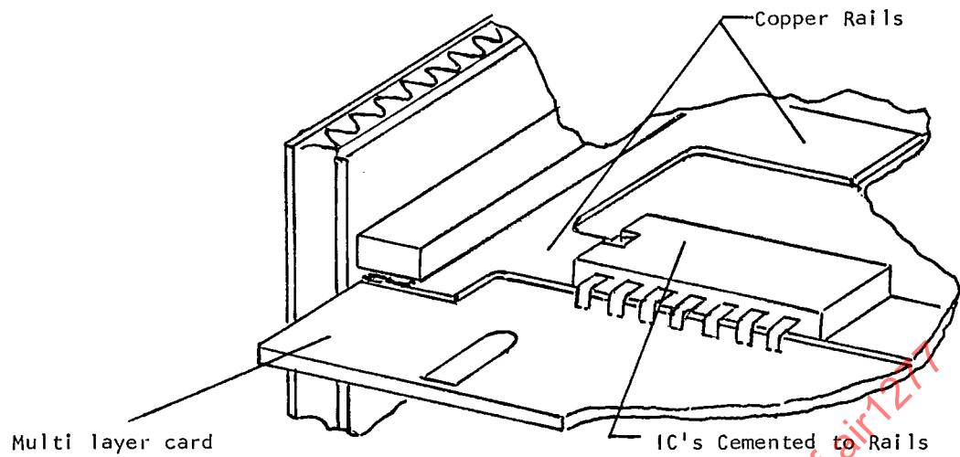
(c) Thermal Shunt Rail
