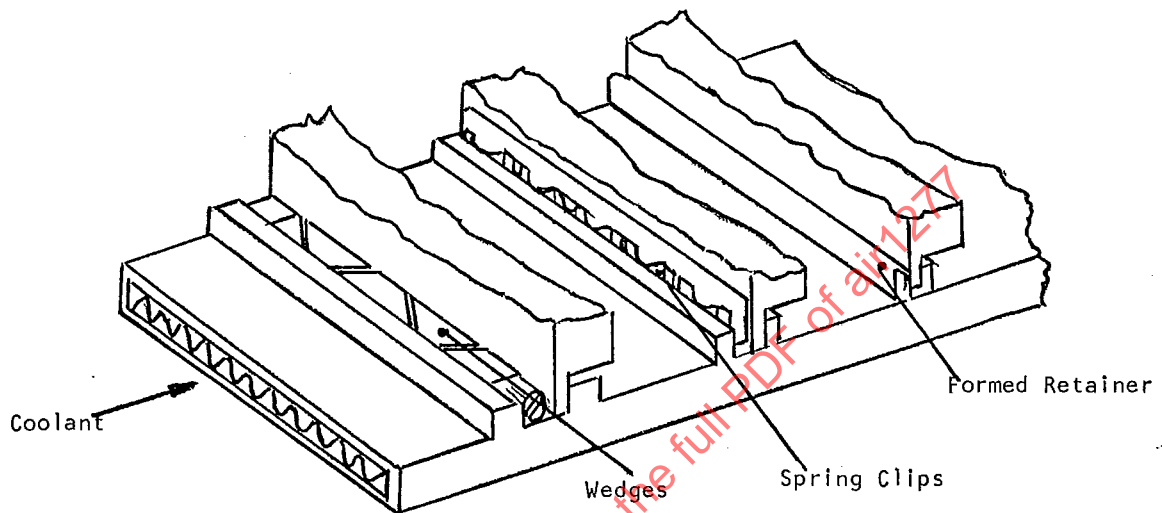
(a) Retaining Circuit Modules with Thermal Conduction
