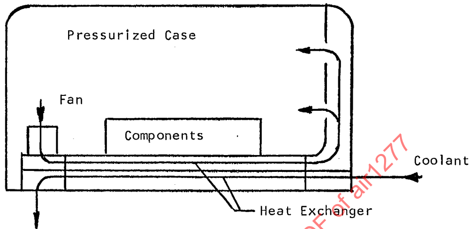
FIGURE 6. Unit with Internal Circulation
