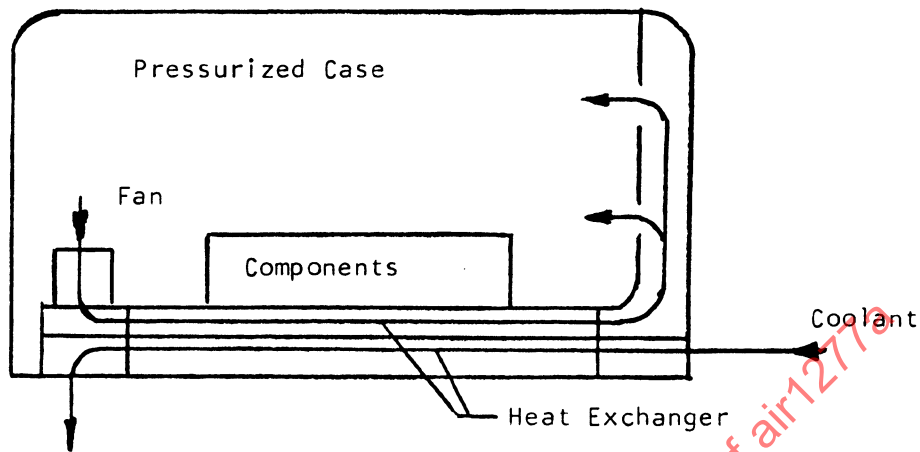
FIGURE 8 - Unit with Internal Circulation
