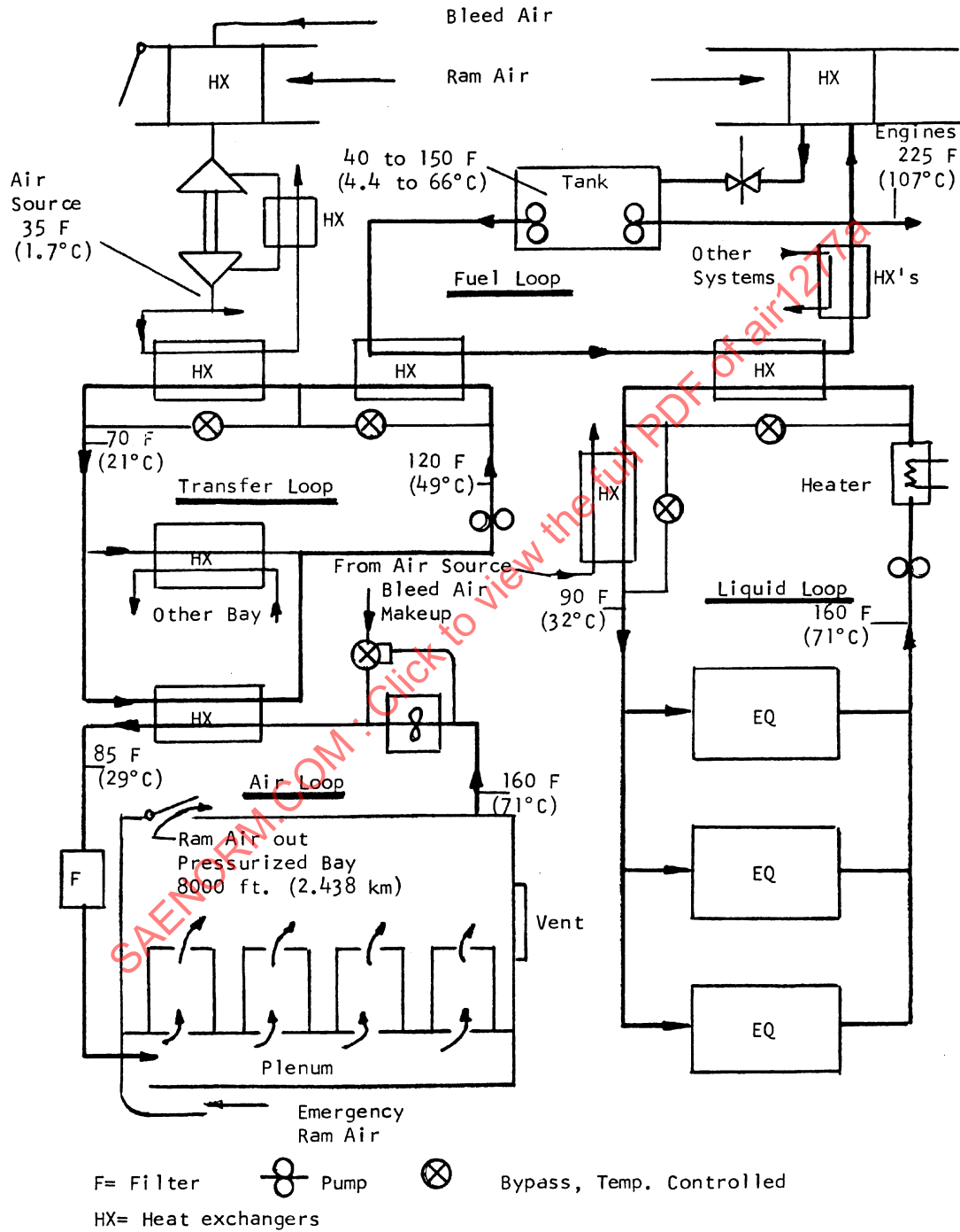
FIGURE 6 - Multiloop Cooling
