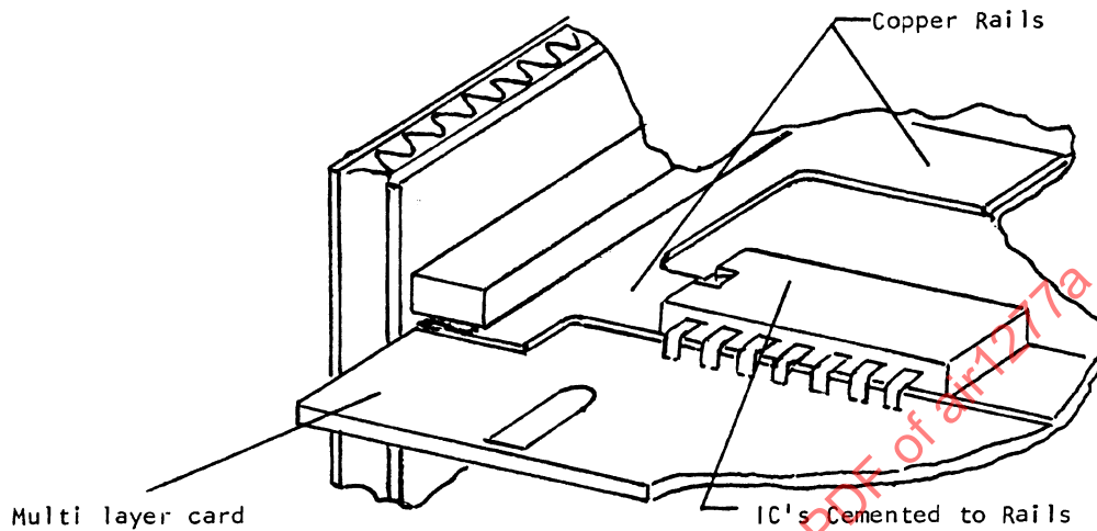
(c) Thermal Shunt Rail
