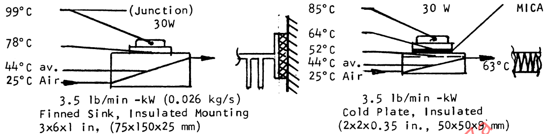
(a) ECS, Air Cooling
