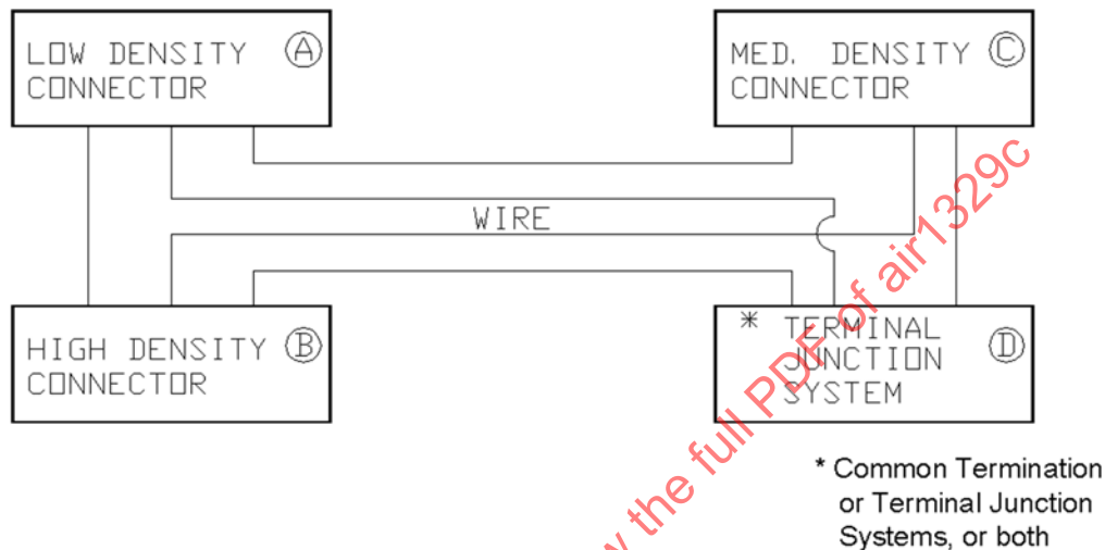
FIGURE 2 - TYPICAL WIRING HARNESS CONCEPT
