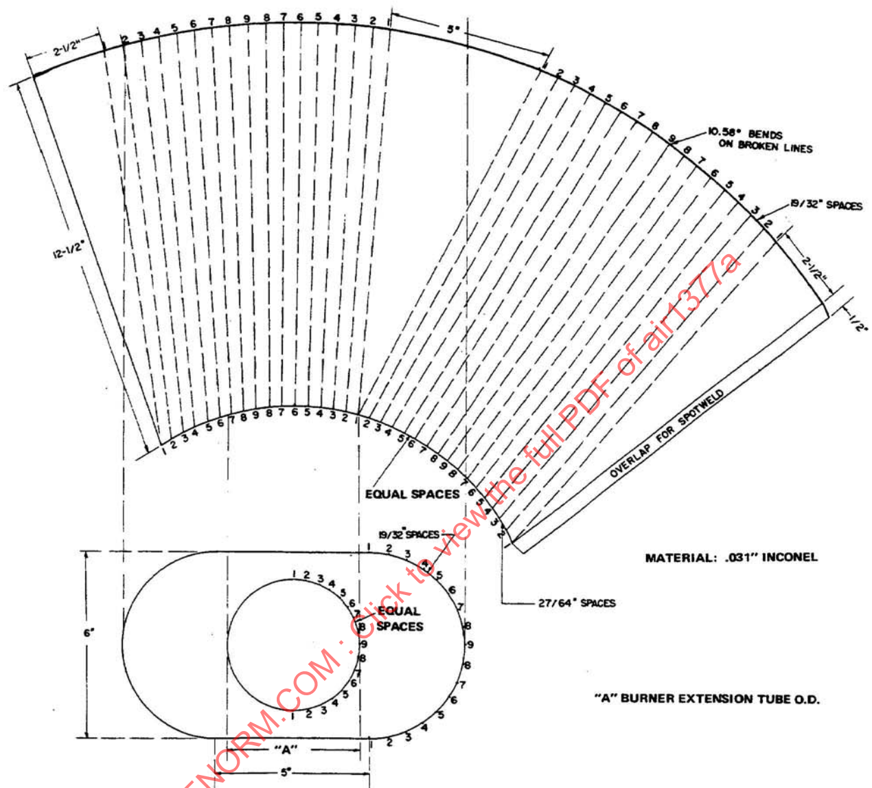
FIGURE 3 - Burner Tube Extension
