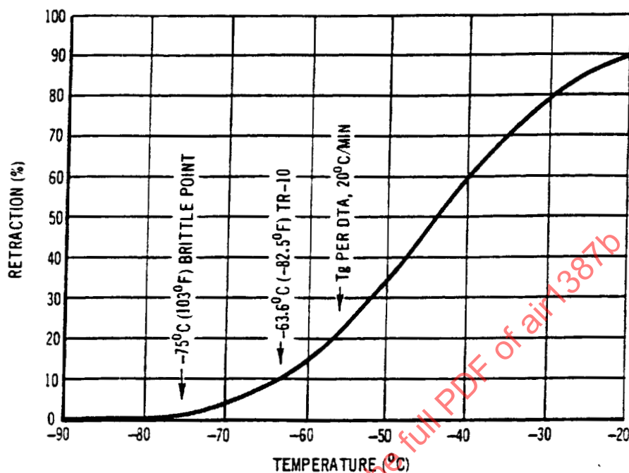
FIGURE 2 - Relationship Between Glass Transition ( T_g ), TR-10 and Brittle Point for a Specific Ethylene Propylene Rubber Compound, as Shown on a Complete Temperature Retraction Curve
