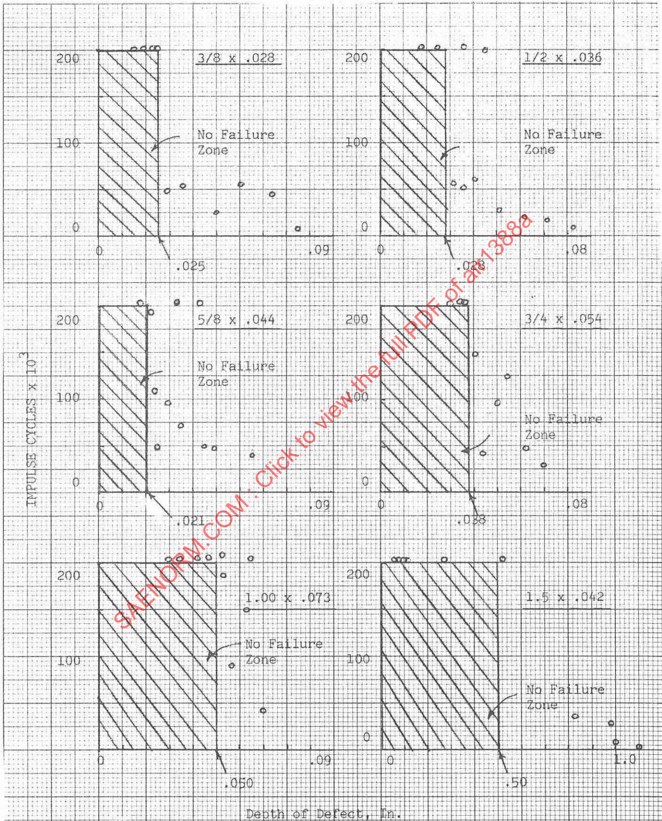
Figure 7 Defect Limits: Dent, Seamless, Annealed, 3Al-2.5V Tubing
