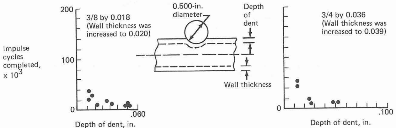
FIGURE 3. IMPULSE TEST DATA, DENTED TUBING, 3000-PSI SYSTEM
