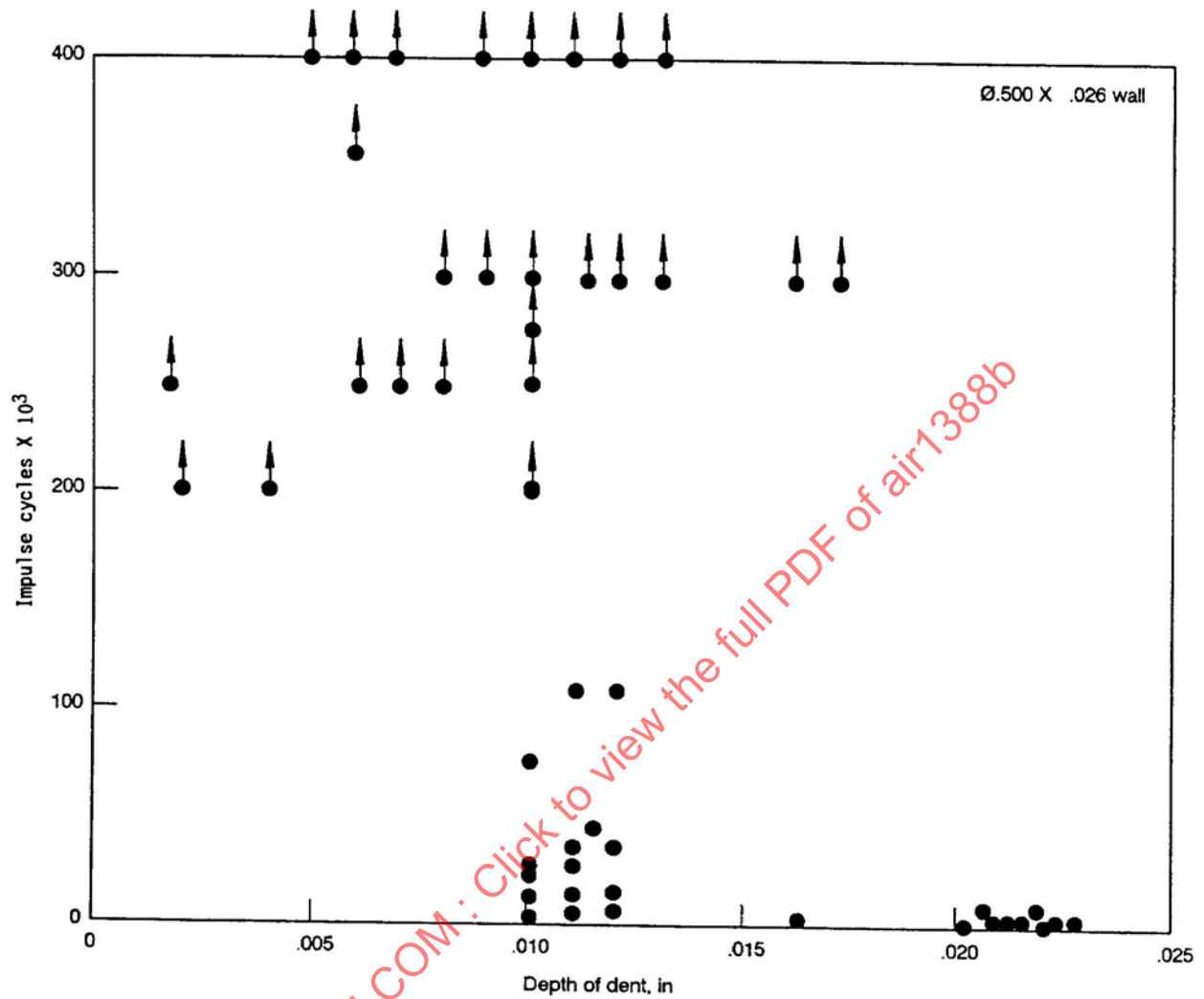
FIGURE 9—Impulse Test Data, Chafed Tubing, Ti-3Al-2.5V CWSR Tubing
