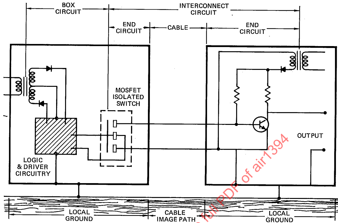
FIGURE 1 INTERCONNECT CIRCUIT
