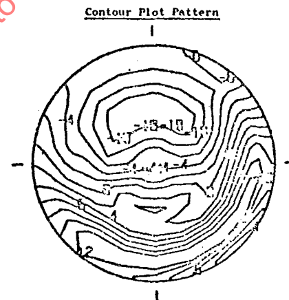
FIGURE 2.13 Tip-Radial Distortion Pattern
