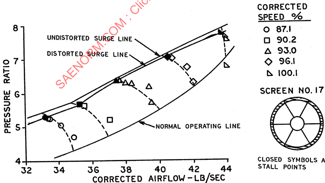
FIGURE 3.16 Example of Tip Radial Total-Pressure Distortion, Narrow Extent
