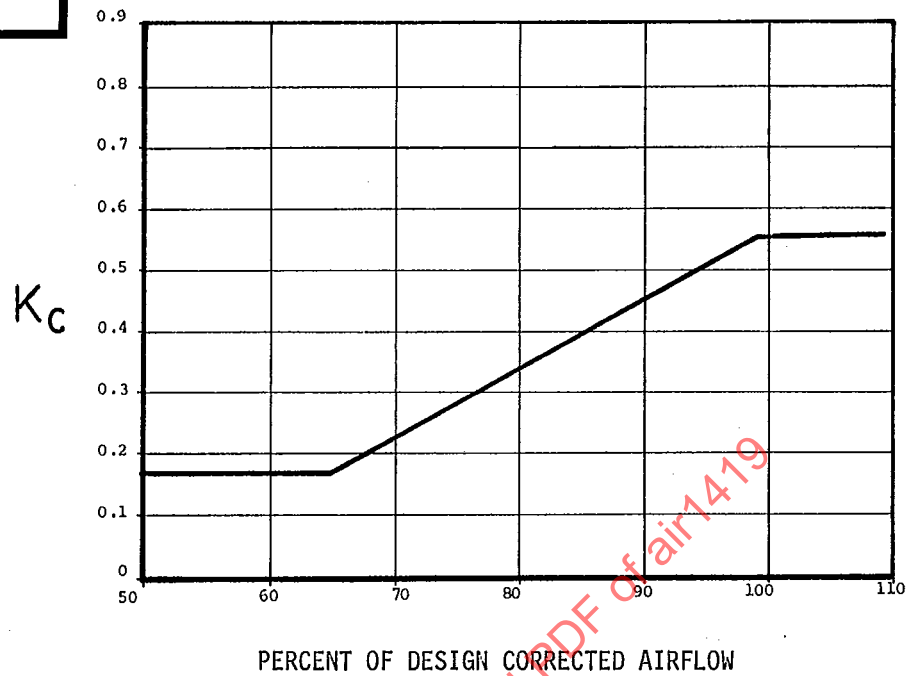
FIGURE 2.22 Circumferential Sensitivity
