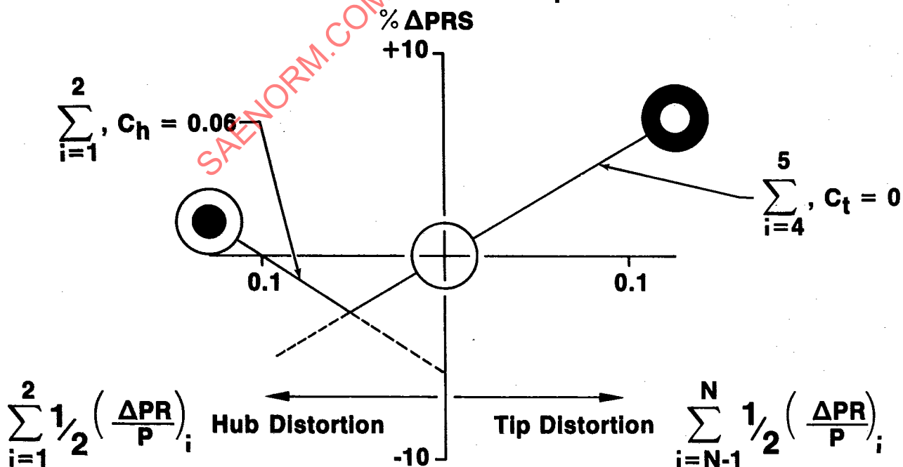
FIGURE 2.29 Modeling Radial Distortion
