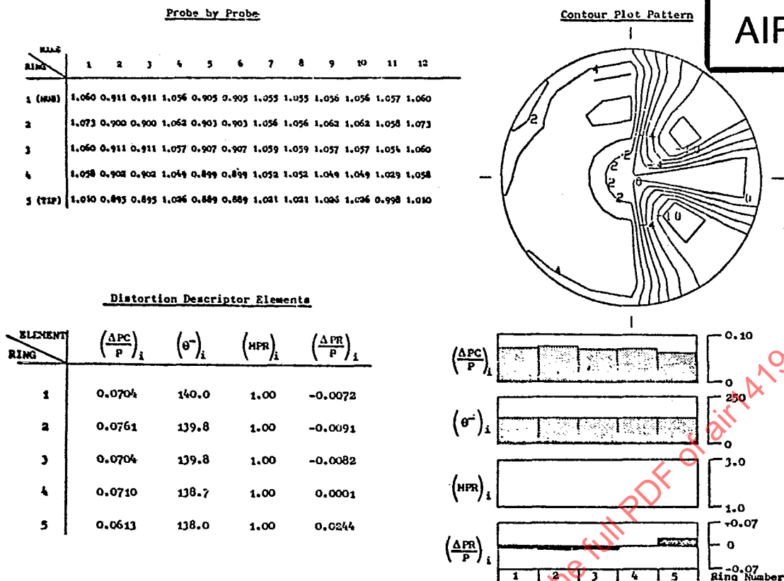
FIGURE 2.17 2/Rev With Lows Closer Than 25 Degrees and With Tip-Radial Distortion Pattern
