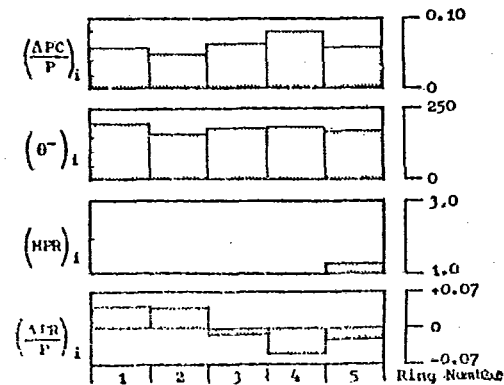
FIGURE 2.14 180 Degree 1/Rev + Hub-Radial Combined Distortion Pattern
