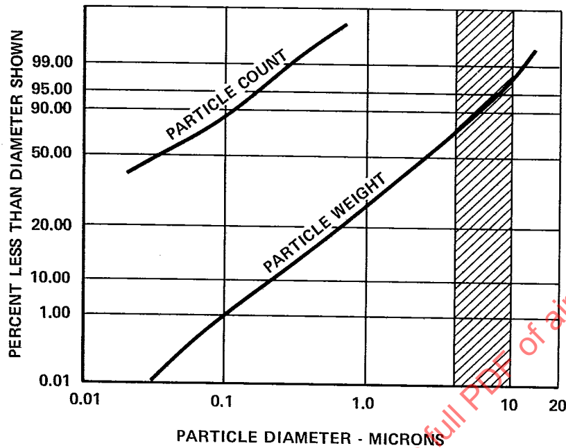
Figure 1. Particle Size Distribution of Atmospheric Dust
