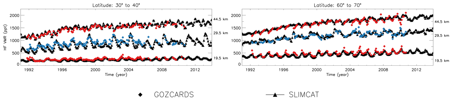
Figure 9 - Hydrogen fluoride measured at latitude © Harrison et al. [2016]. Reproduced with permission. License CC by 3.0. All rights reserved.
