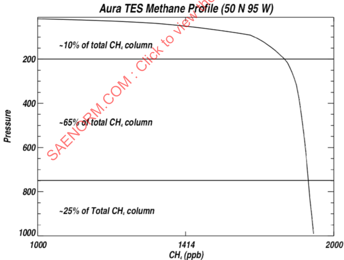
Figure 10 - Methane measured at atmospheric pressure © Worden, J.R., Turner, A.J., Bloom, A.A., Kulawik, S.S., et al. [2015]. Reproduced with permission. License CC by 3.0. All rights reserved.
