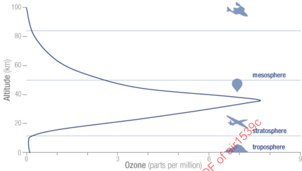
Figure 5 - Ozone measured at altitude © NASA. [2018]. All rights reserved.
