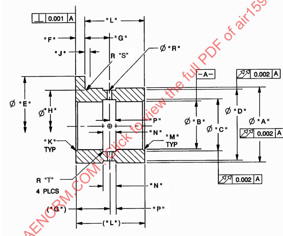
FIGURE 1 - TYPICAL LANDING GEAR JOURNAL BEARING
