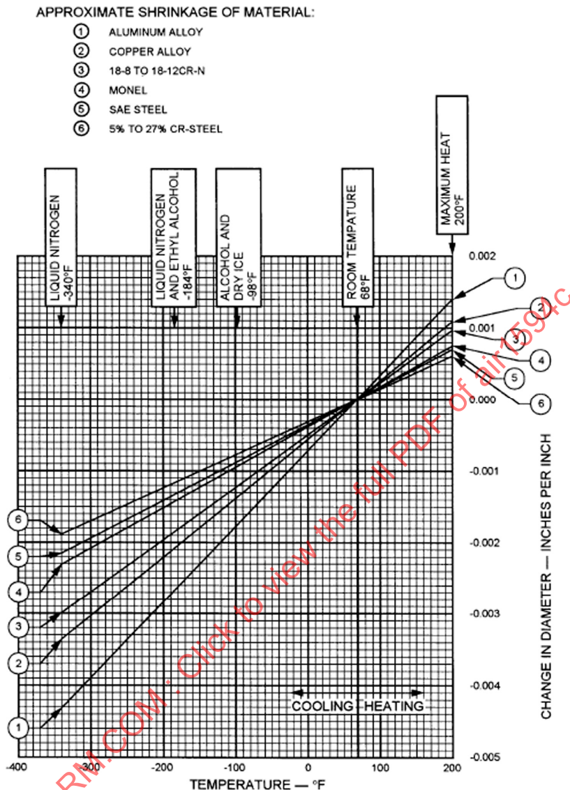
FIGURE 2 - SUB-ZERO INSTALLATION OF BEARINGS
