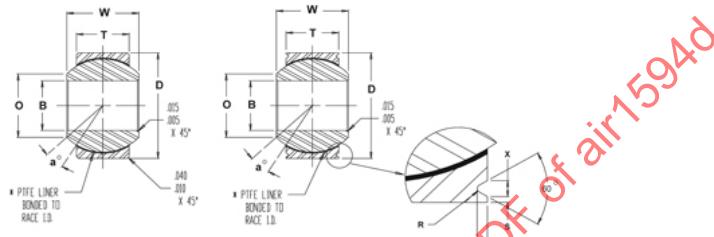
Figure 2 - Typical PTFE lined landing gear spherical bearing
