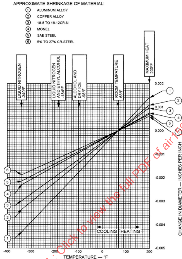
Figure 3 - Sub-zero installation of bearings
