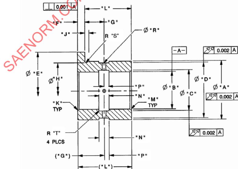
Figure 1 - Typical landing gear journal bearing
