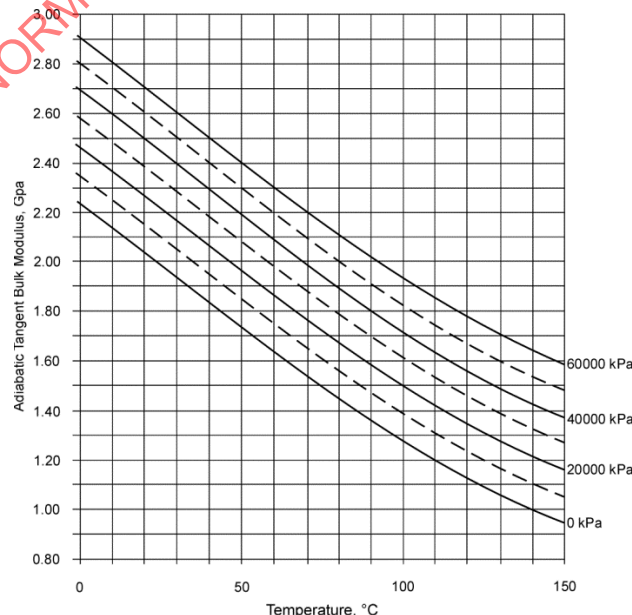
Figure 6 - Adiabatic tangent bulk modulus, MIL-PRF-83282
