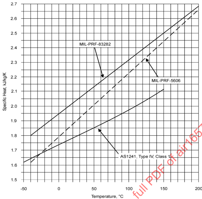
Figure 8 - Specific heat of hydraulic fluids
