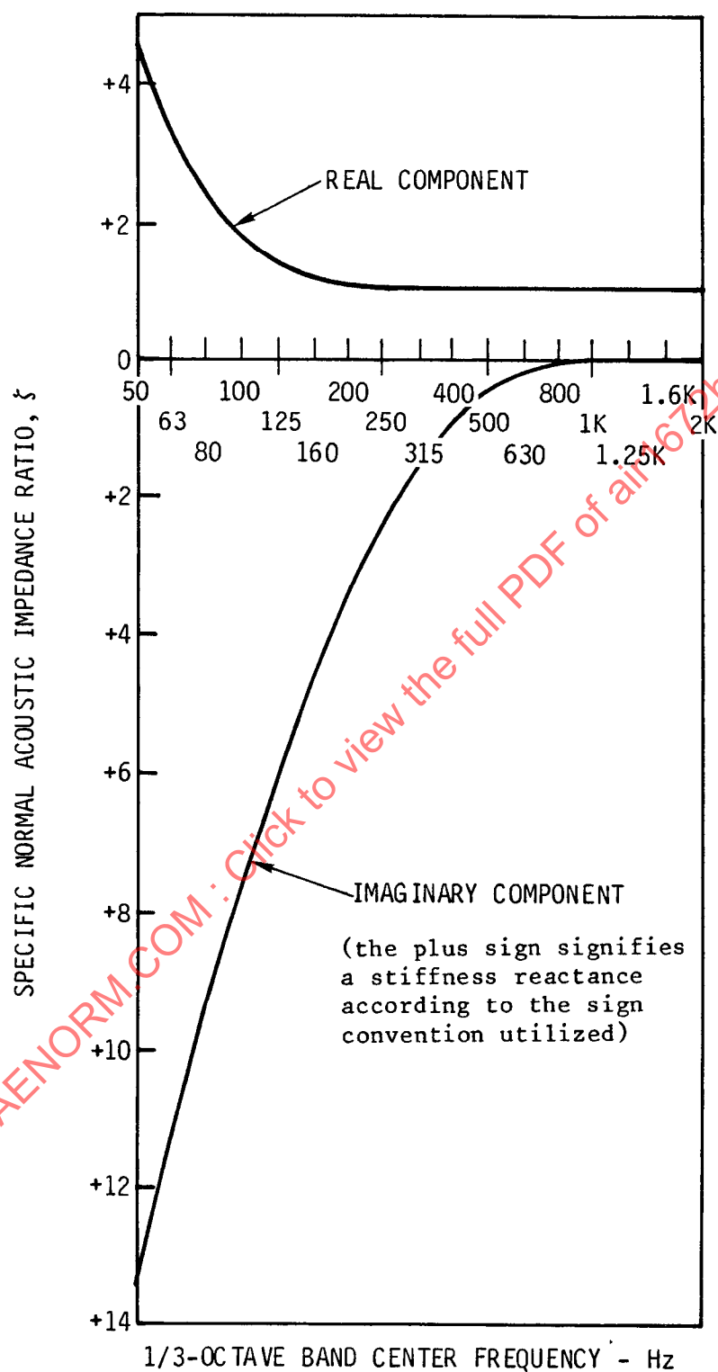
Figure C7 Specific Normal Acoustic Impedance Ratio for the Crushed Stone Surface at the P&WA Test Facility
