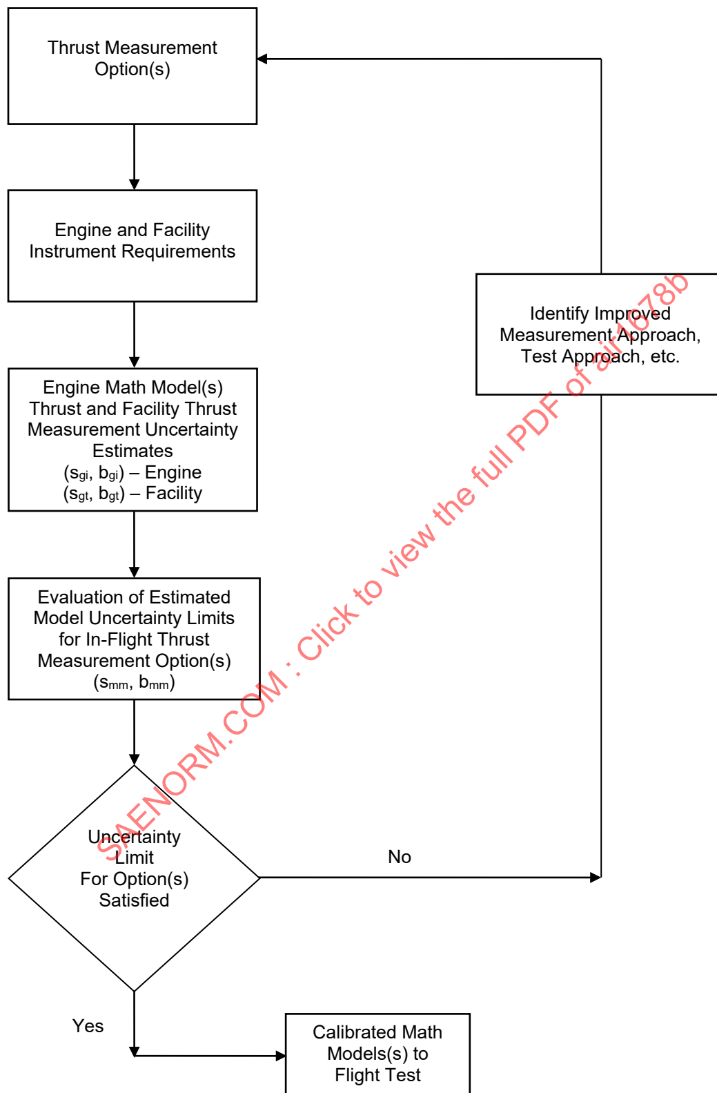
FIGURE 13 - GROUND TEST MEASUREMENT PROCESS EVALUATION CYCLE
