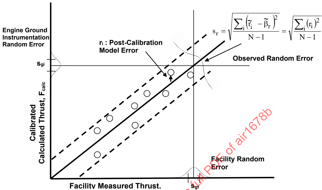
FIGURE 16 - ILLUSTRATION OF MATHEMATICAL MODEL (CORRECTED FOR \tilde{\beta}_r ) STANDARD DEVIATION
