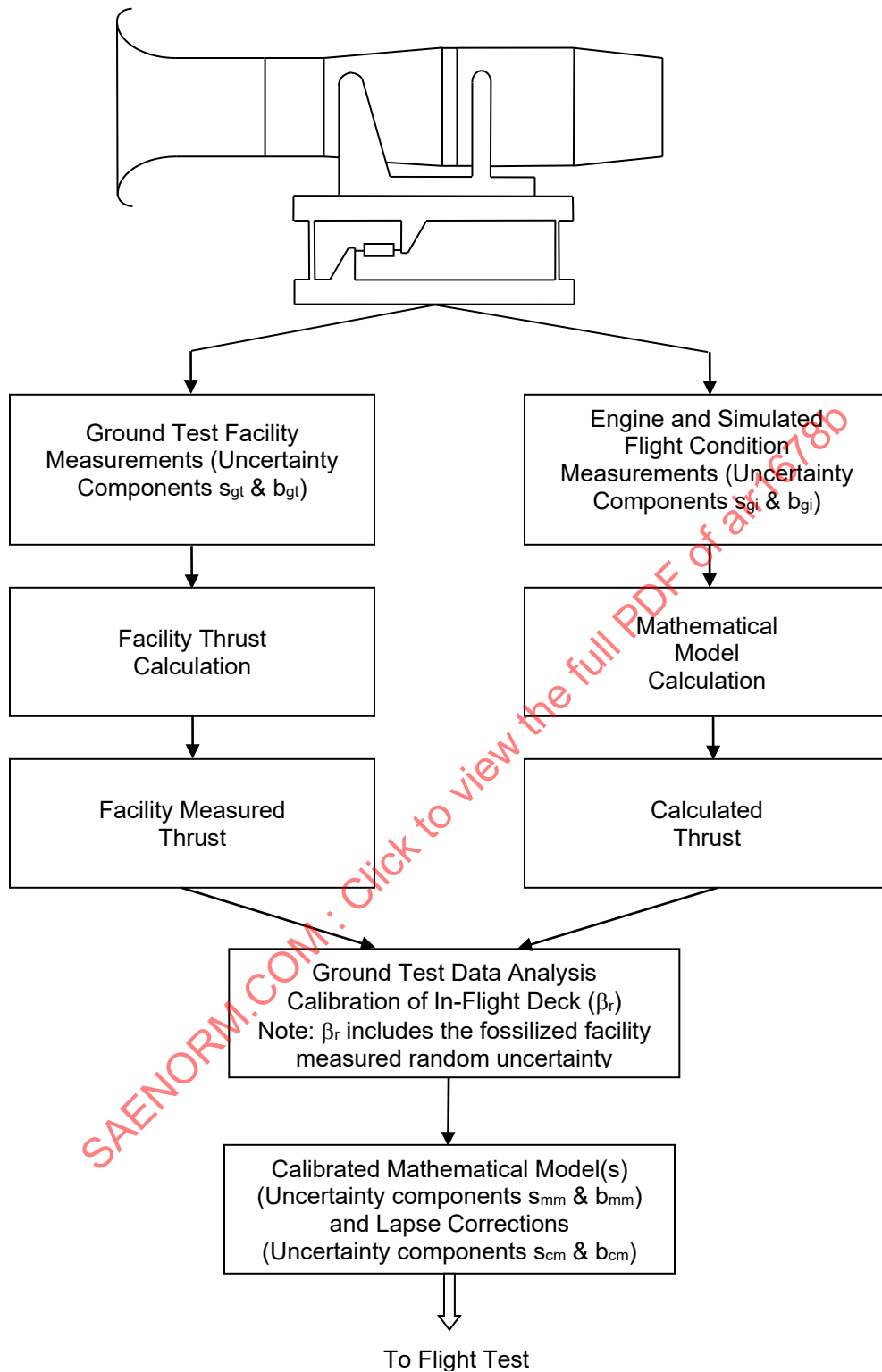
FIGURE 11 - GROUND TEST THRUST MEASUREMENT PROCESS INCLUDING DEFINITION/CALIBRATION OF MATHEMATICAL MODEL(S)
