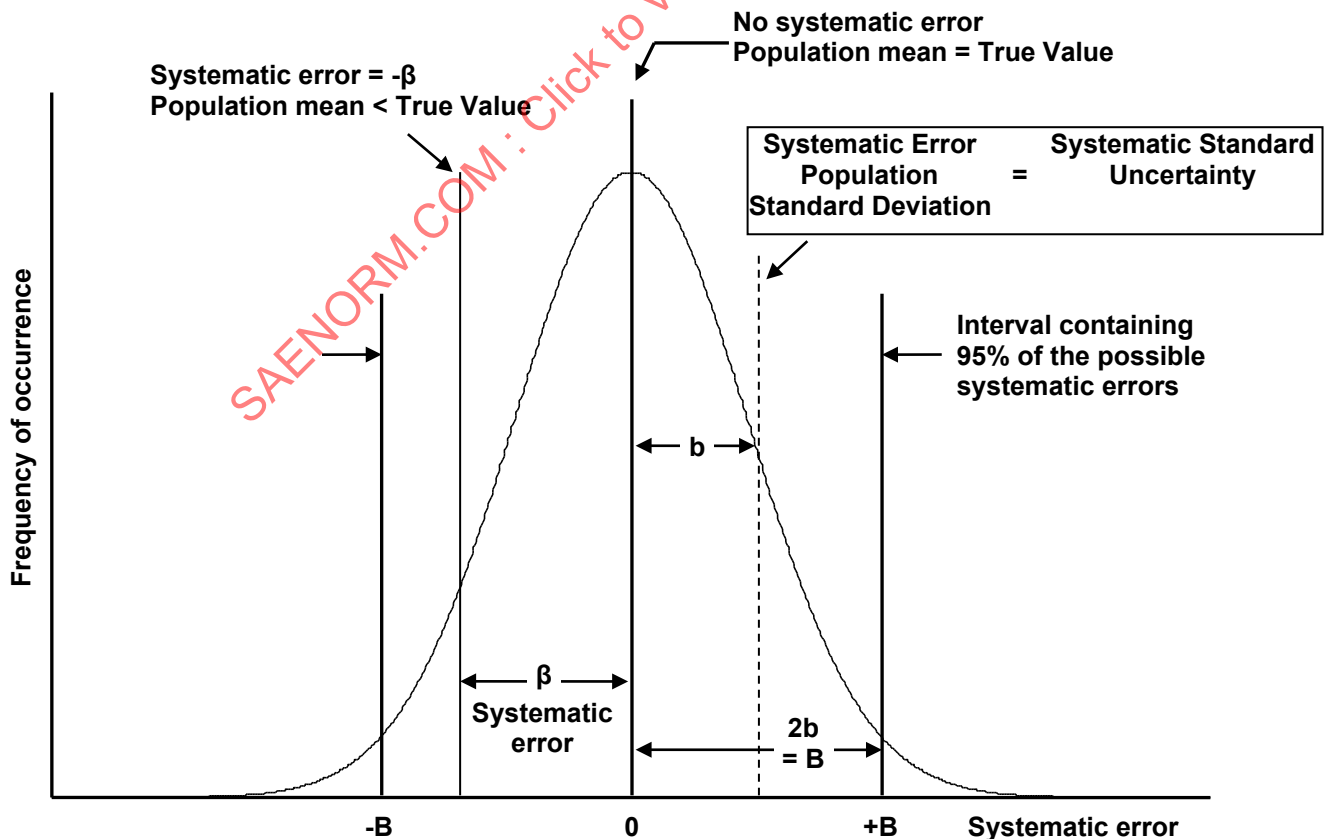
FIGURE 10 - SYSTEMATIC STANDARD UNCERTAINTY ESTIMATION (WITH A NORMAL DISTRIBUTION OF B)
