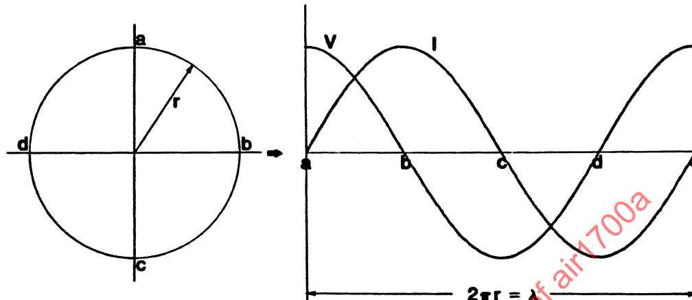
FIGURE 1 - Voltage and Current Distribution on a Cylinder in a Plane Transverse to the Axis of Propagation, When the Perimeter of the Cylinder is One Wavelength Long
