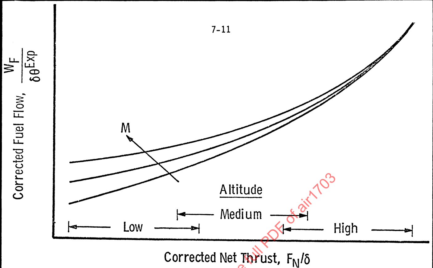
Figure 7.5 - Engine Part-Power Corrected Thrust Versus Corrected Fuel Flow
