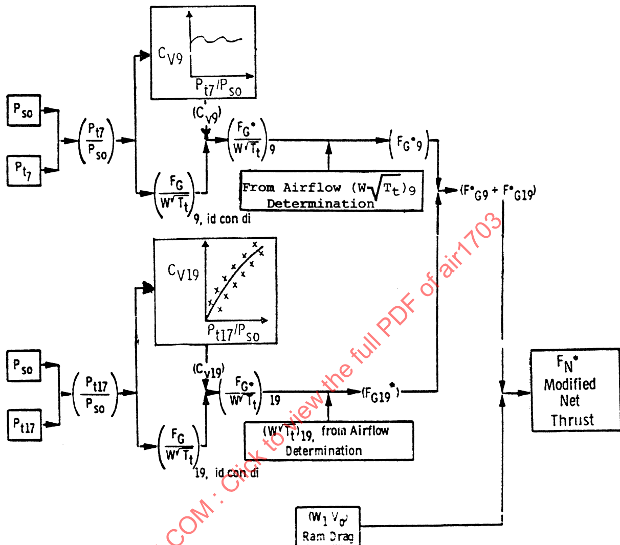
Figure 4.7 (Cont'd) - Gas-Path/Nozzle Method for Separate-Stream Turbofan
