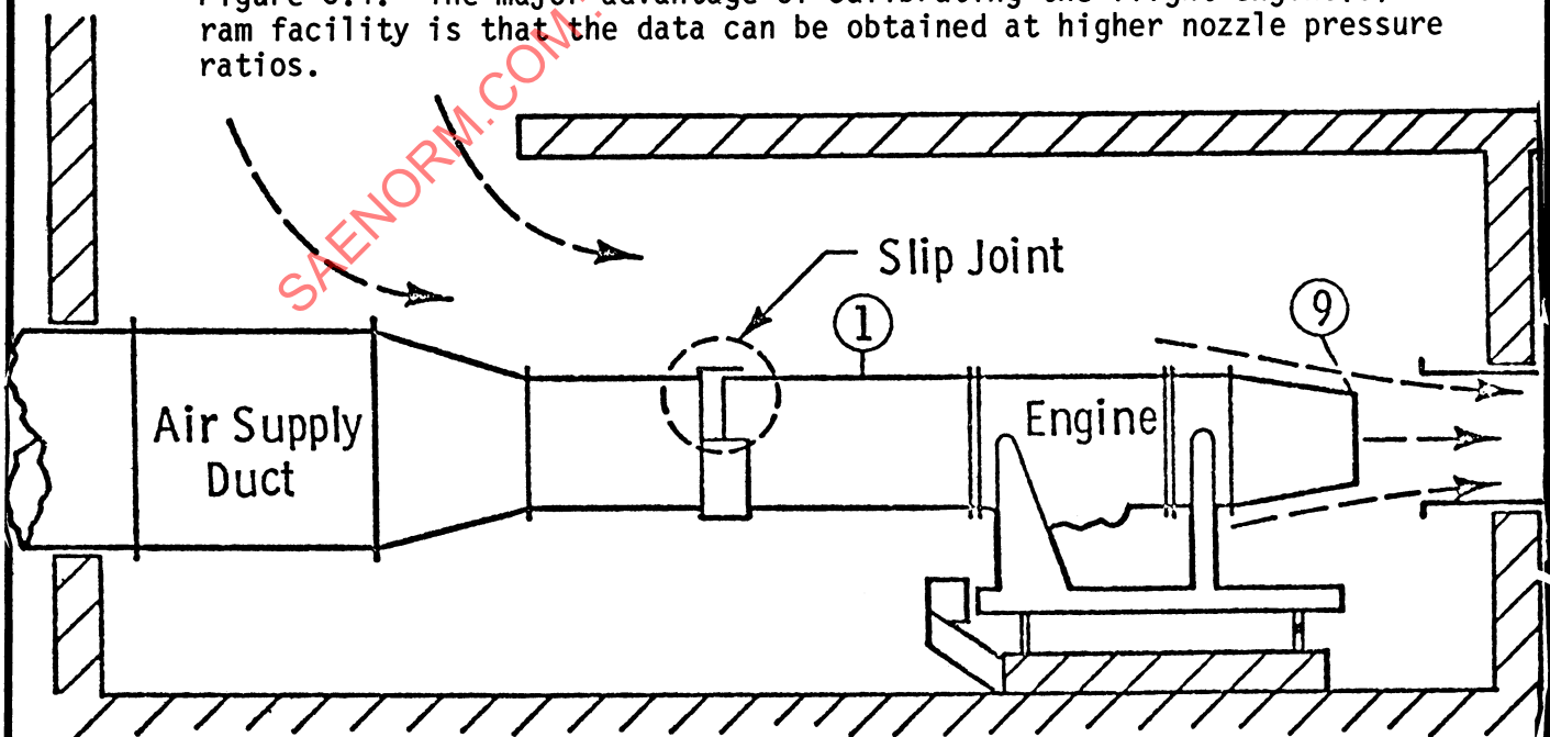
Figure 5.5 - Ground Level Test Cell with Inlet Ram Capability
