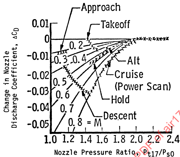
Figure 5.14 - Nozzle Flow Coefficient Suppression
