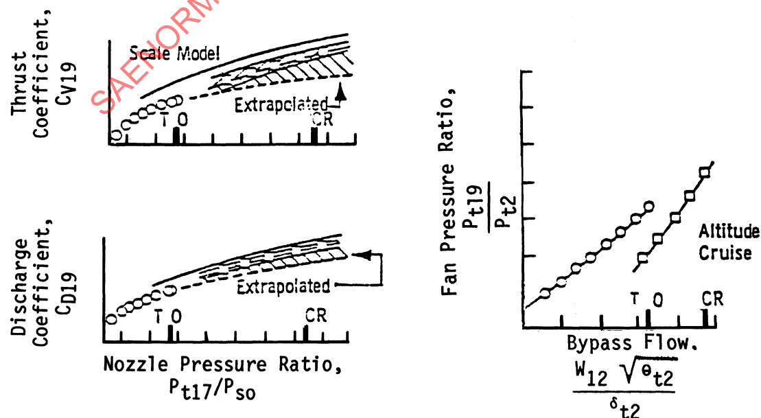
Figure 4.2 - Nozzle Coefficient Extrapolation for High-Bypass-Ratio Engine
