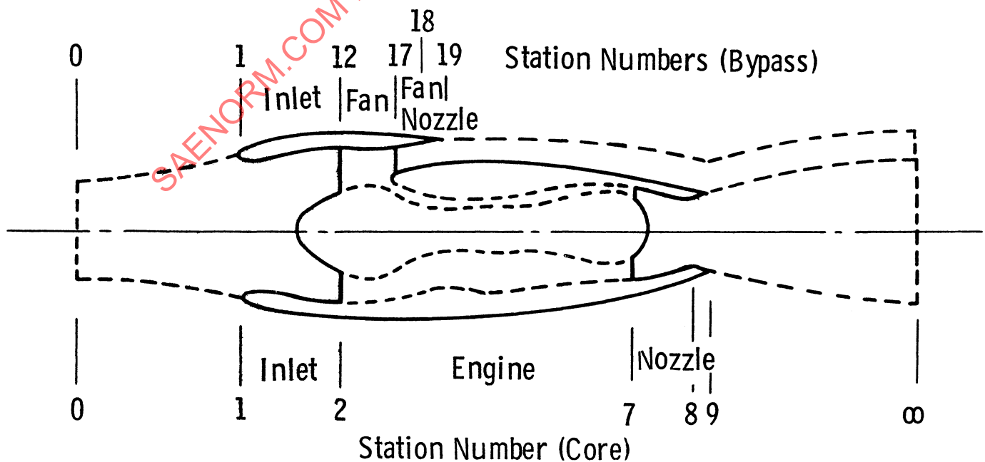
Figure 2.1 - Station Numbering System
