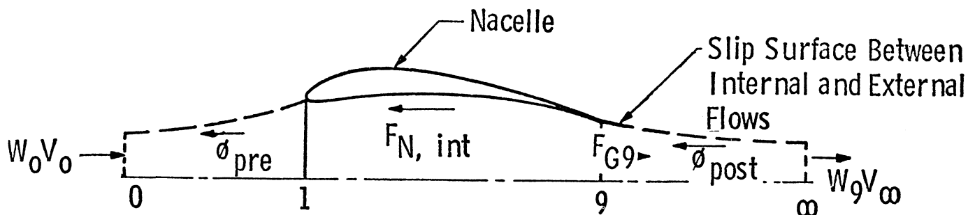
Figure 2.2 - Force Components for Simple Nacelle
