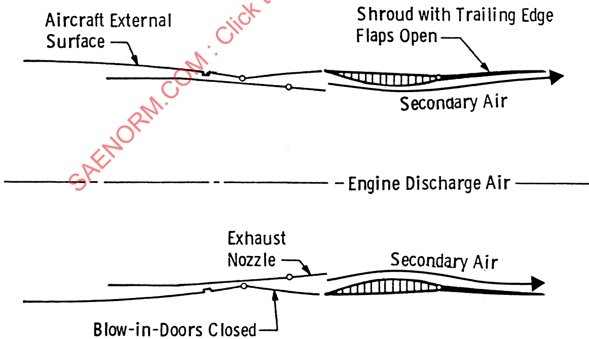
Figure 3.7 - Typical Ejector Nozzle, Afterburning
