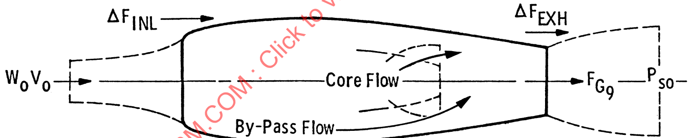
Figure 3.3 - Mixed-Flow Turbofan
