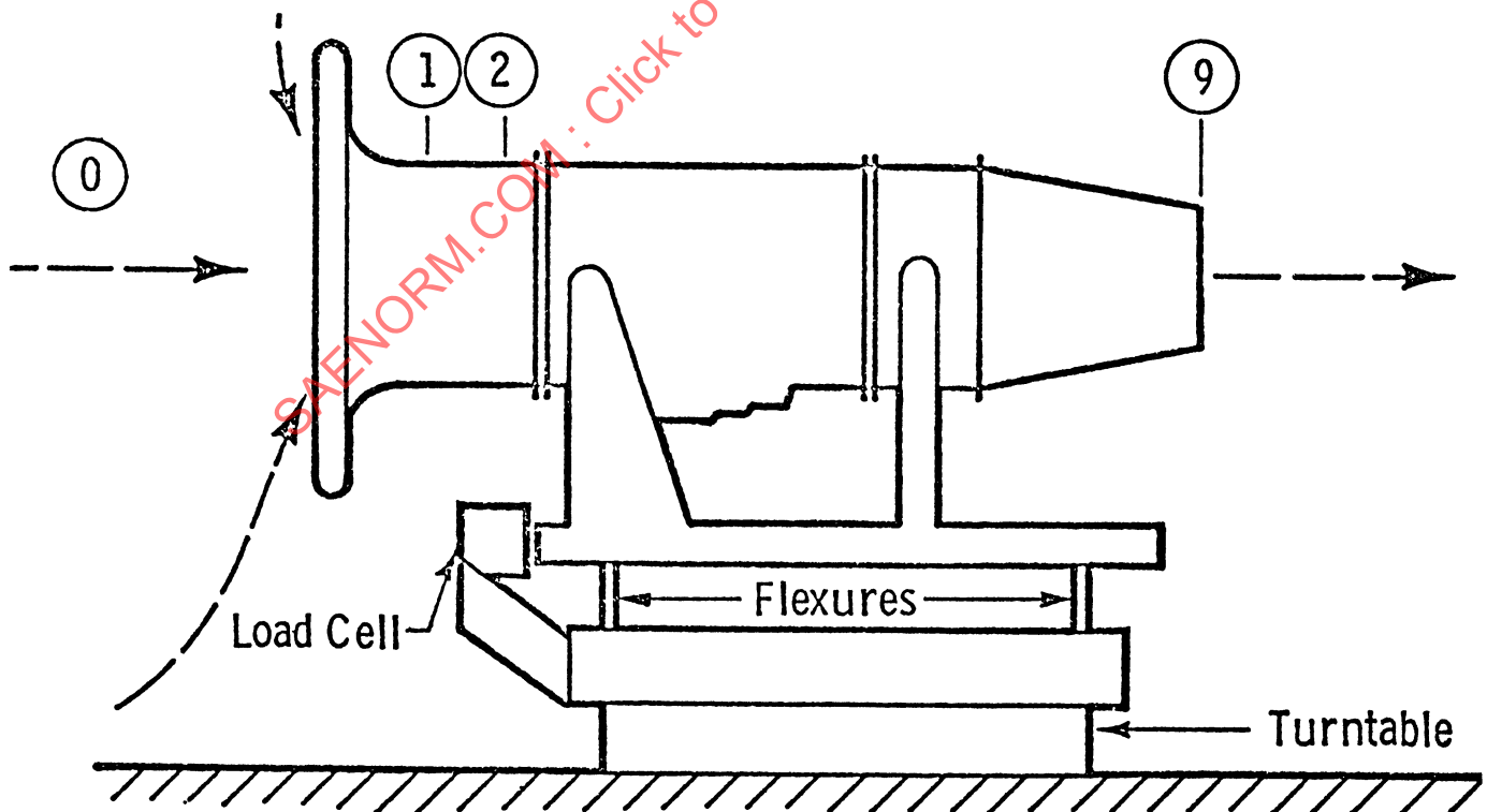
Figure 5.1 - Open-Air Test Stand
