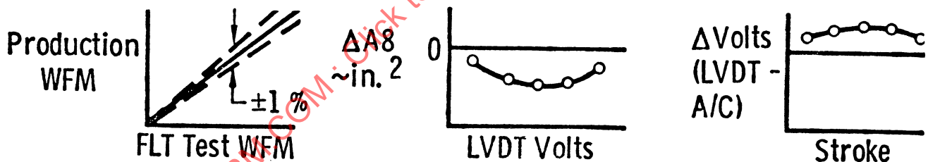
Figure 7.17 - Data Validity Checks - Steady-State Maneuvers
