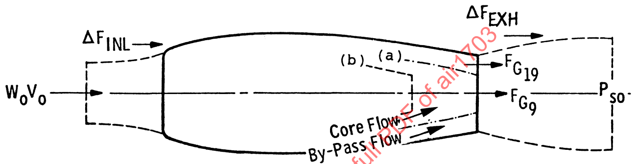
Figure 3.2 - Long-Duct Turbofans
