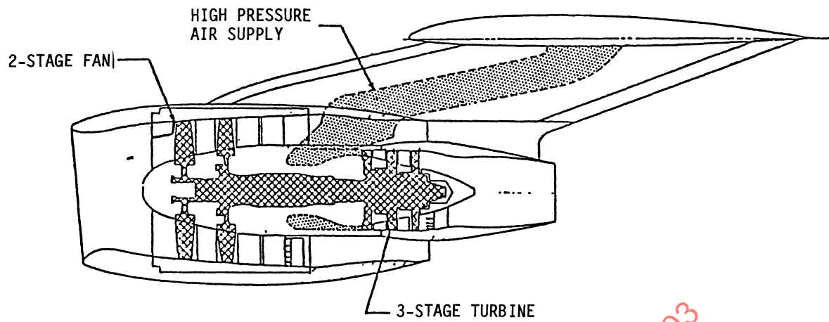
Figure 5.21 - Subsonic Turbo-Powered Simulator Cross Section
