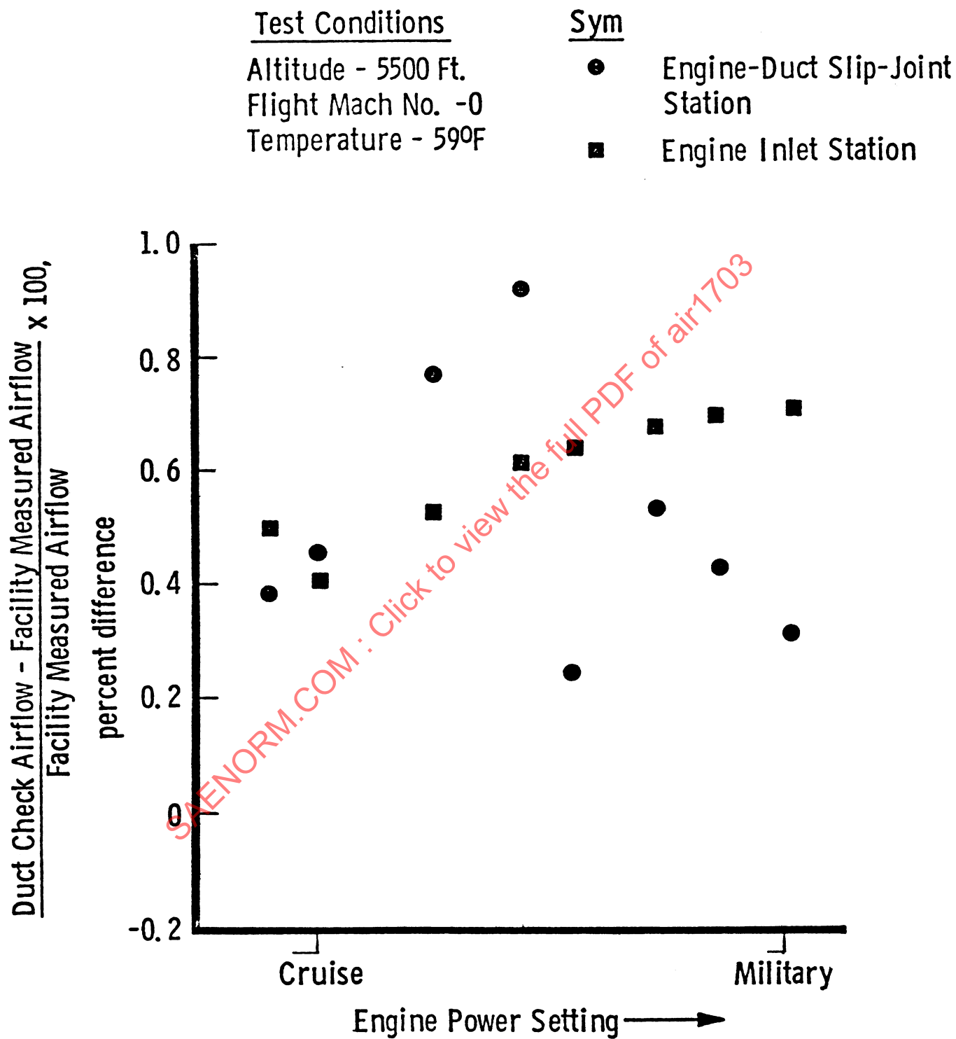
Figure 7.1 - Airflow Duct Check (Nonafterburning Turbojet Engine)
