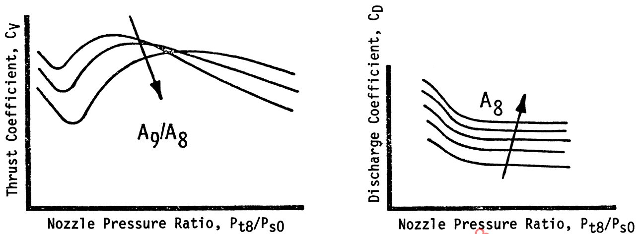
Figure 5.13 - C-D Nozzle Performance Curves
