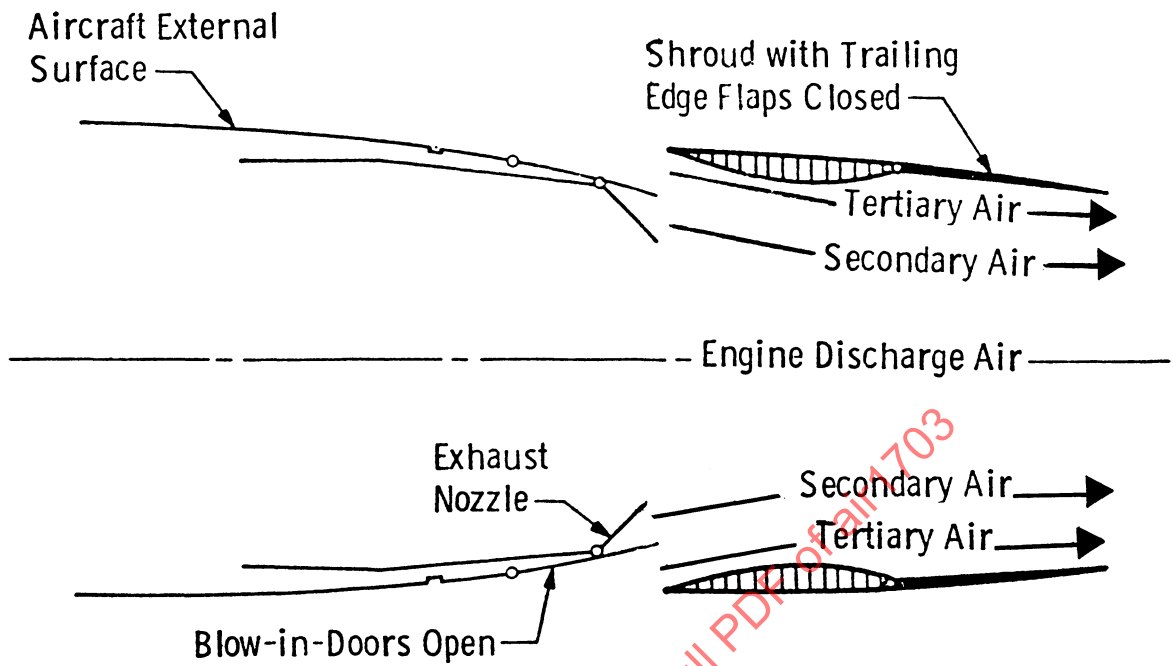
Figure 3.6 - Typical Ejector Nozzle, Non-Afterburning
