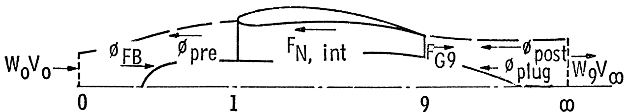
Figure 2.3 - Force Components for Centerbody Nacelle
