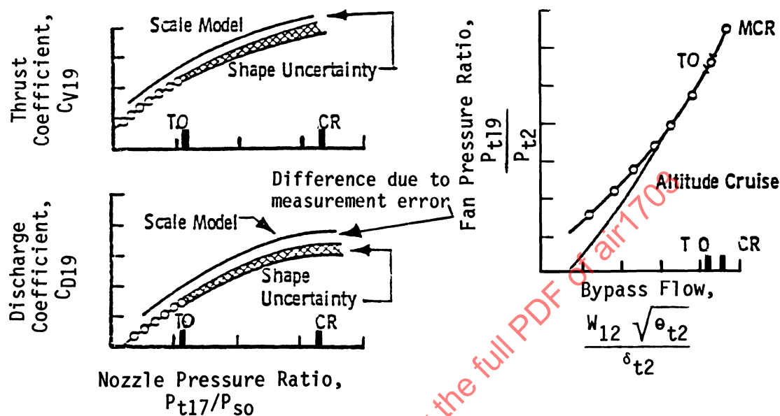
Figure 4.1 - Nozzle Coefficient Extrapolation for Low-Bypass-Ratio Engine
