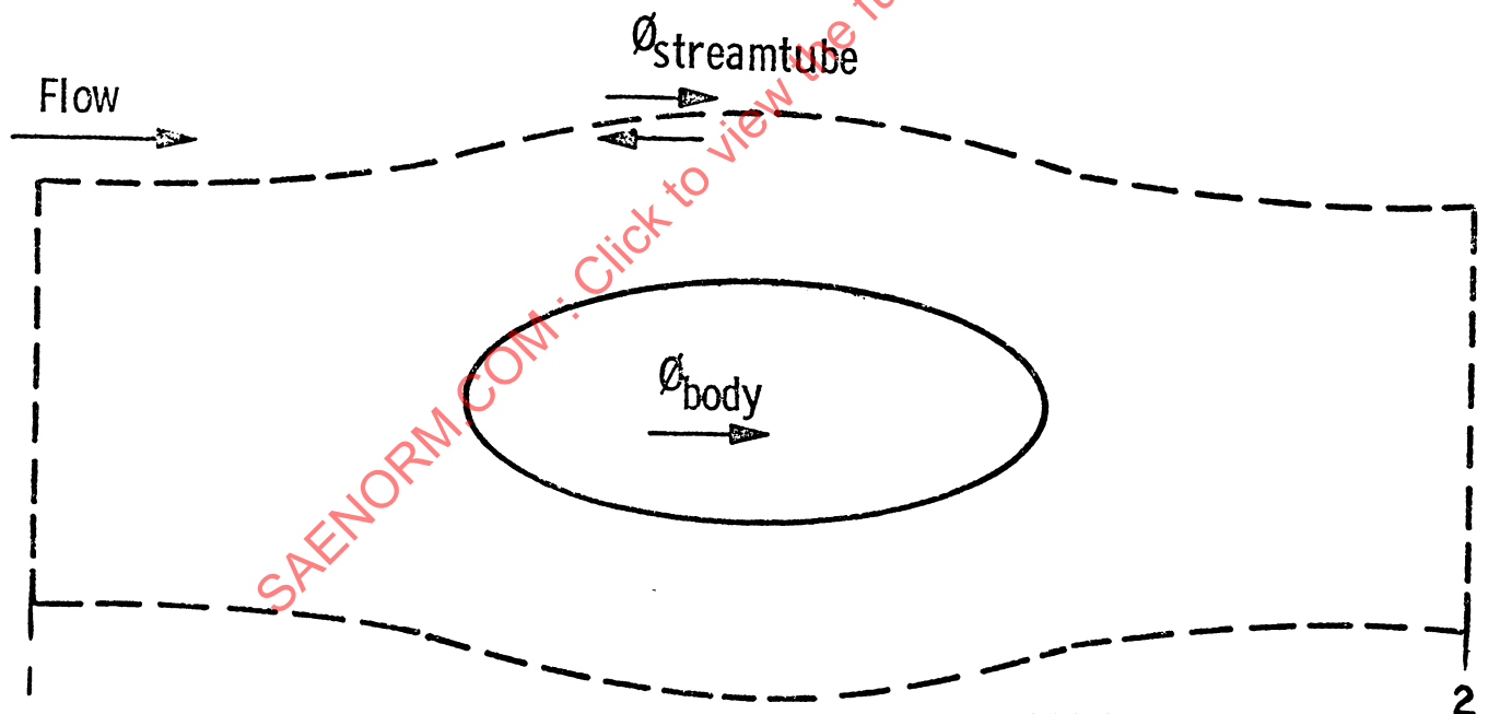
Figure A.3 - Flow About a Closed Non-Lifting Body
