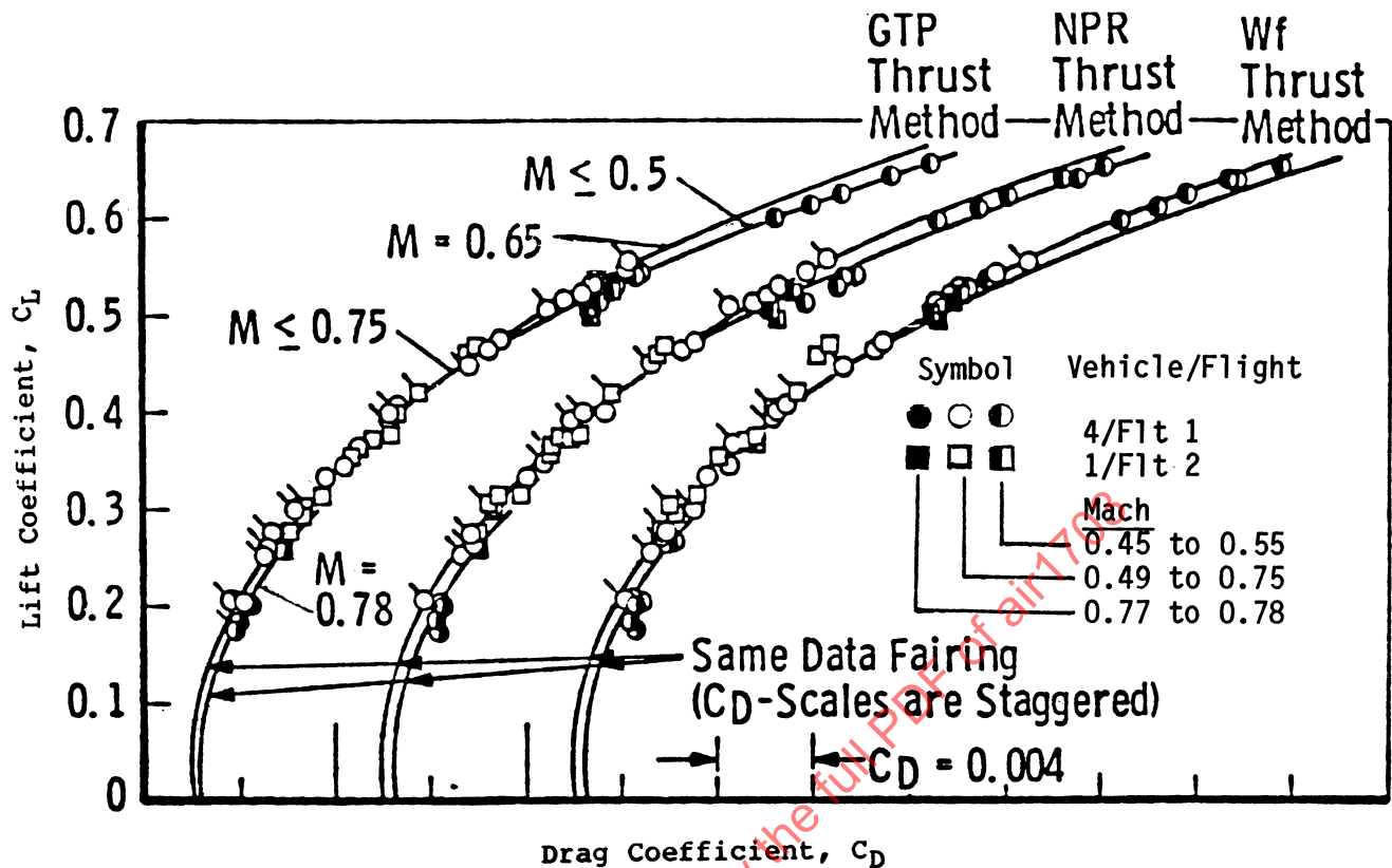
Figure 7.12 - Flight Test Drag Variation with Lift - Thrust Method Comparison
