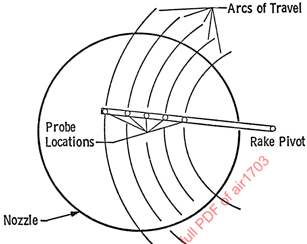
Figure 4.3 - Traversing Rake Arrangement
