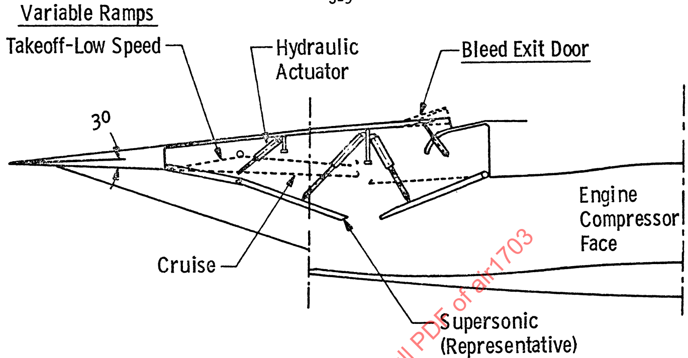
Figure 3.8 - Typical 2-D Inlet With Ramps
