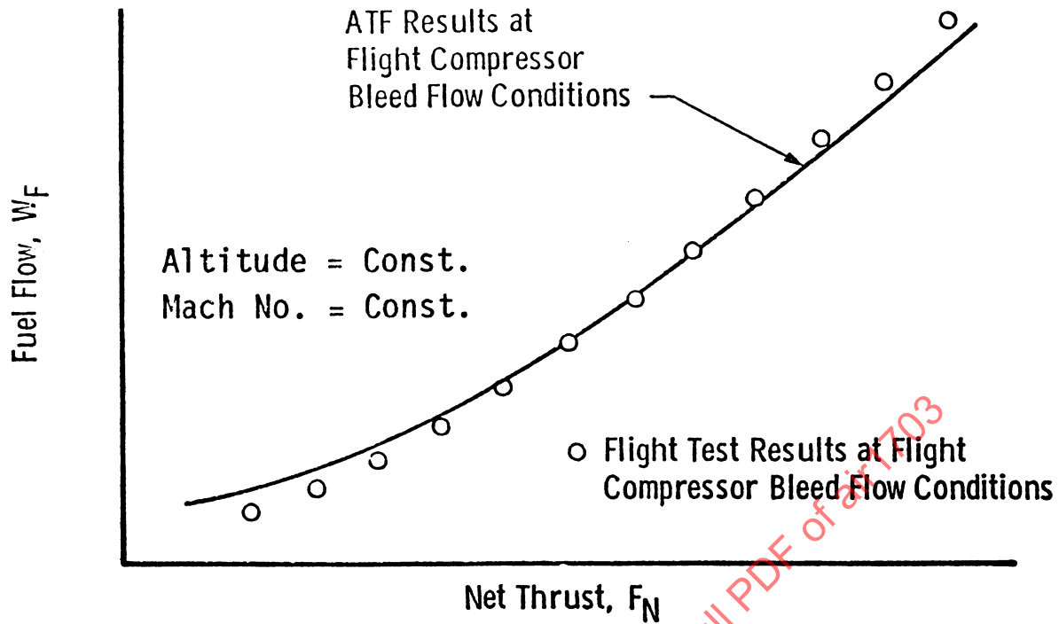
Figure 7.7 - ATF/Flight-Engine Thrust Versus Fuel Flow With Compressor Bleed Airflow
