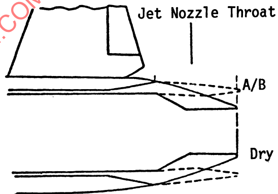
c. Variable Area Convergent/Divergent
