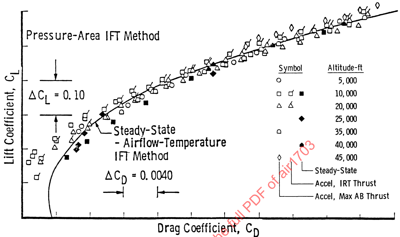
Figure 7.18 - Flight Test Drag Characteristics-Pressure-Area IFT Method
