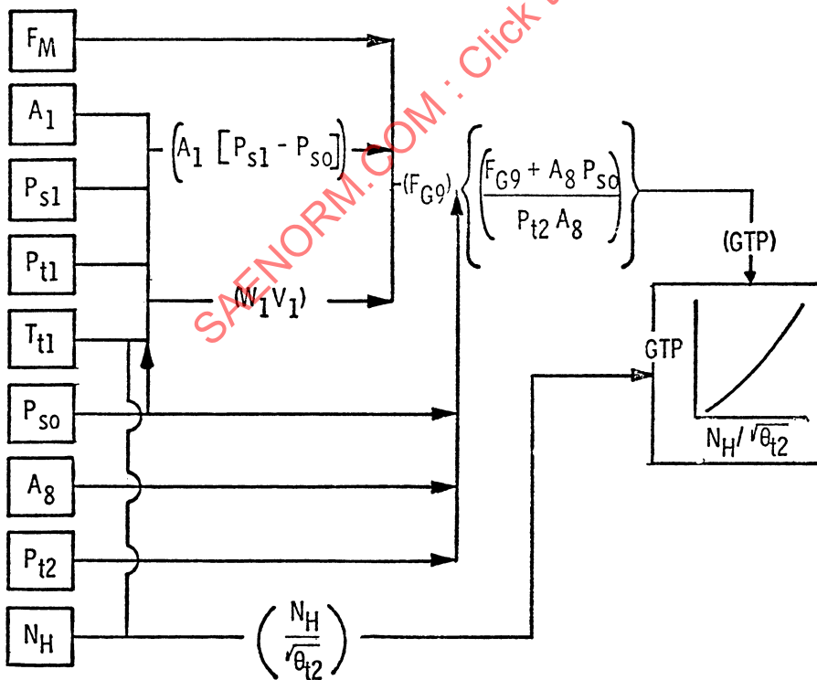
Figure 5.6 (Cont'd) - Single-Exhaust Turbofan ATF Calibration
