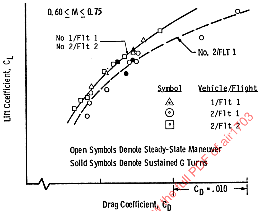
Figure 7.9 - Flight Test Drag Characteristics
