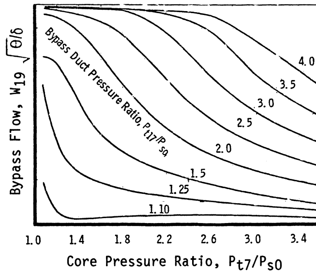
Figure 5.12 - Alternate Mixed Flow Exhaust System Performance Parameters
