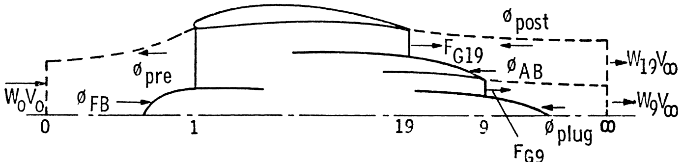
Figure 2.4 - Force Components for Dual Stream Nacelle
