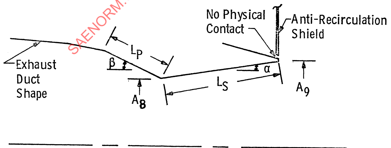
Figure 5.16 - Model Geometric Similarities
