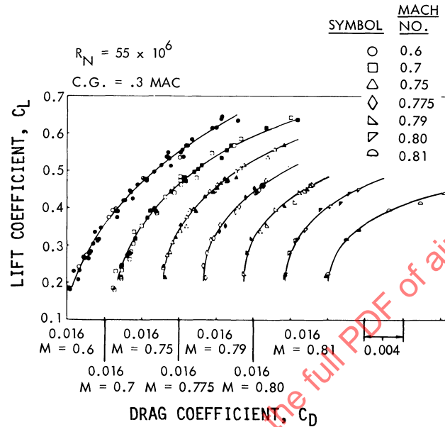
Figure 7.15 - Flight Test Drag Characteristics
