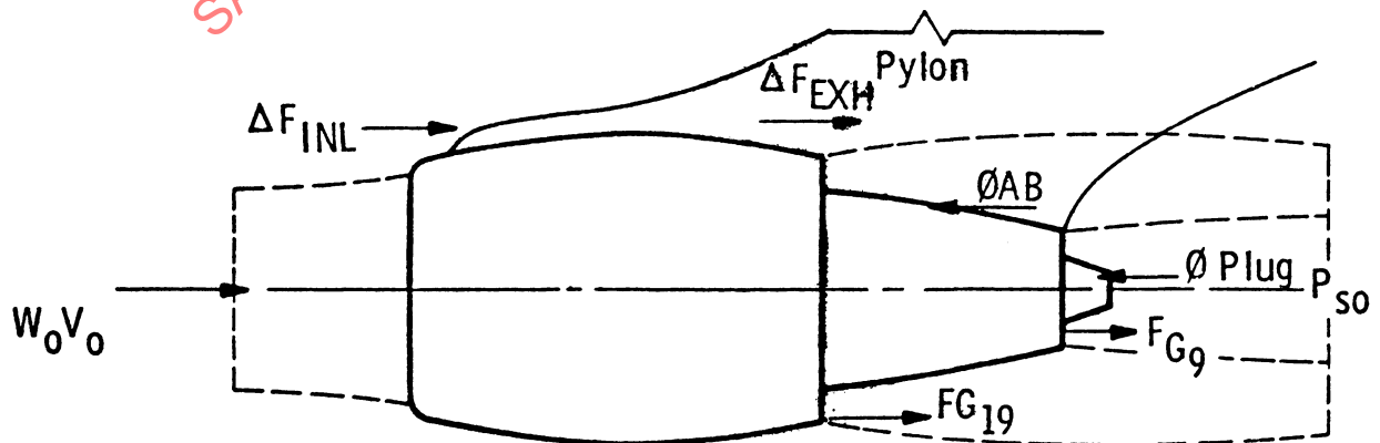
Figure 3.4 - Intermediate or Short Duct Turbofan
