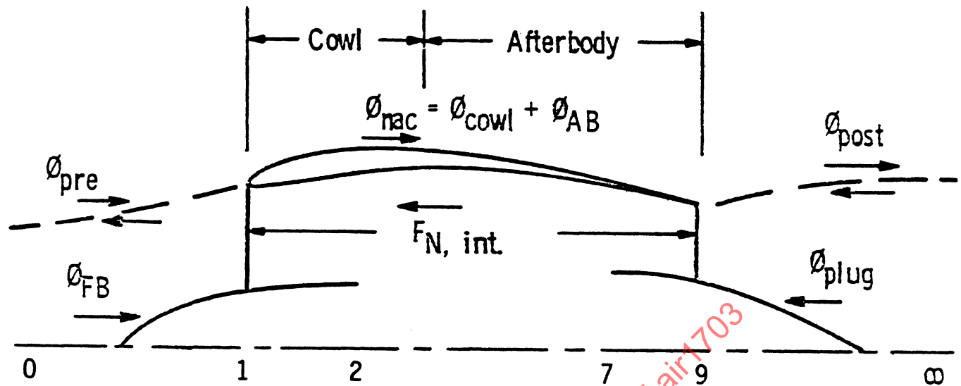
Figure 2.5 - Forces Acting on a Propulsion System
