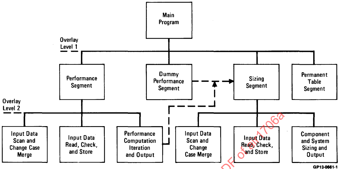
Figure 1. Computer Program Structure
