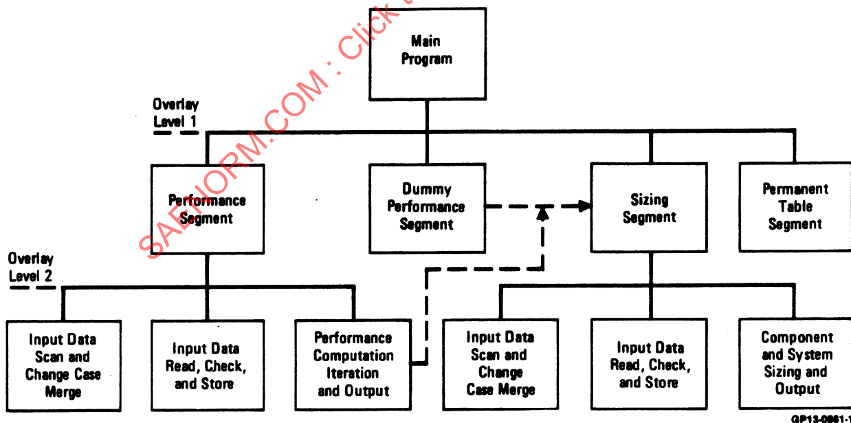
FIGURE 1 - Computer Program Structure
