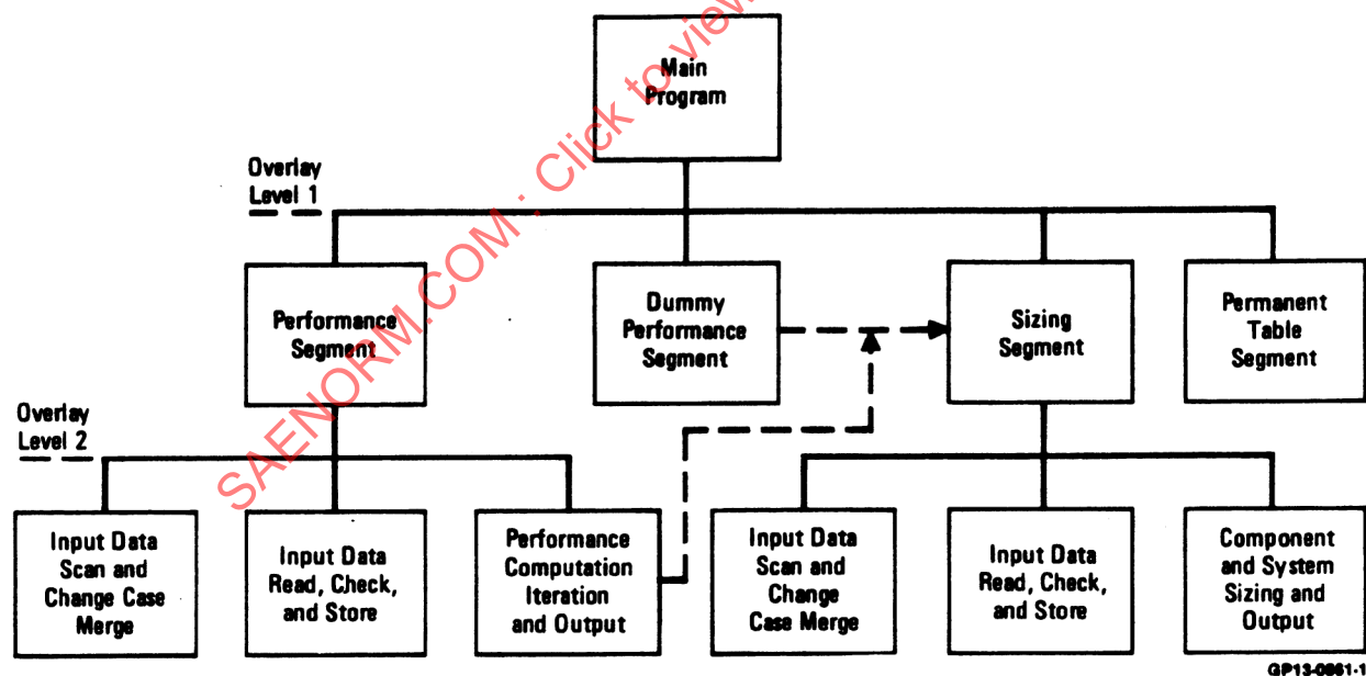
FIGURE 1 - Computer Program Structure
