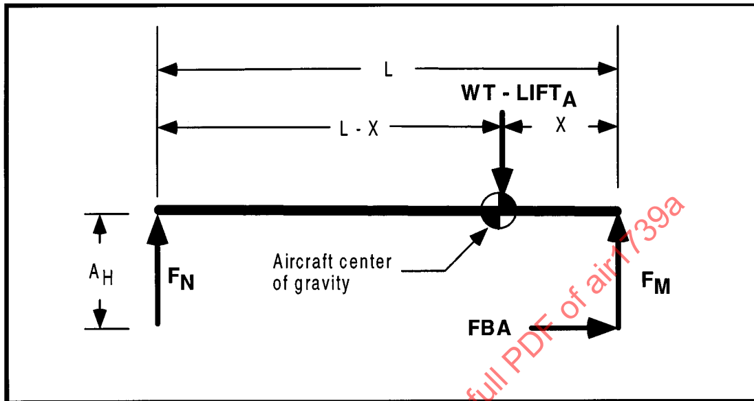
FIGURE 13 - Aircraft Landing Gear Geometry
