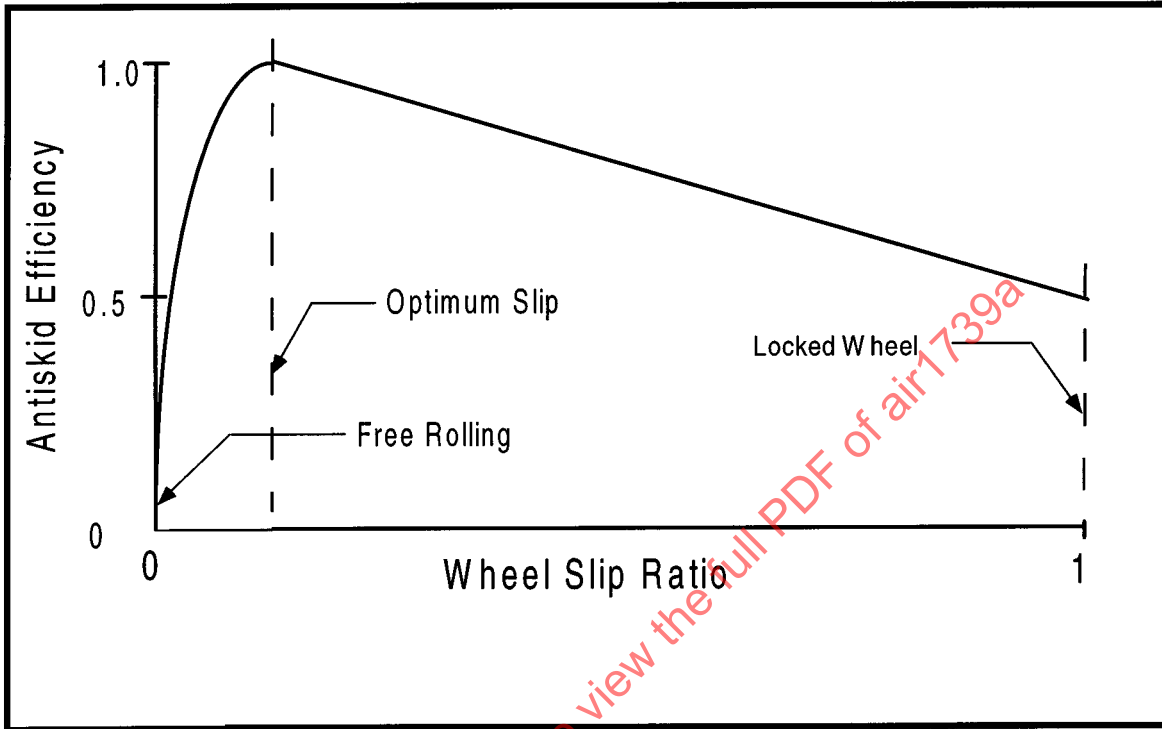
FIGURE 15 - Antiskid Efficiency Versus Wheel Slip Ratio
