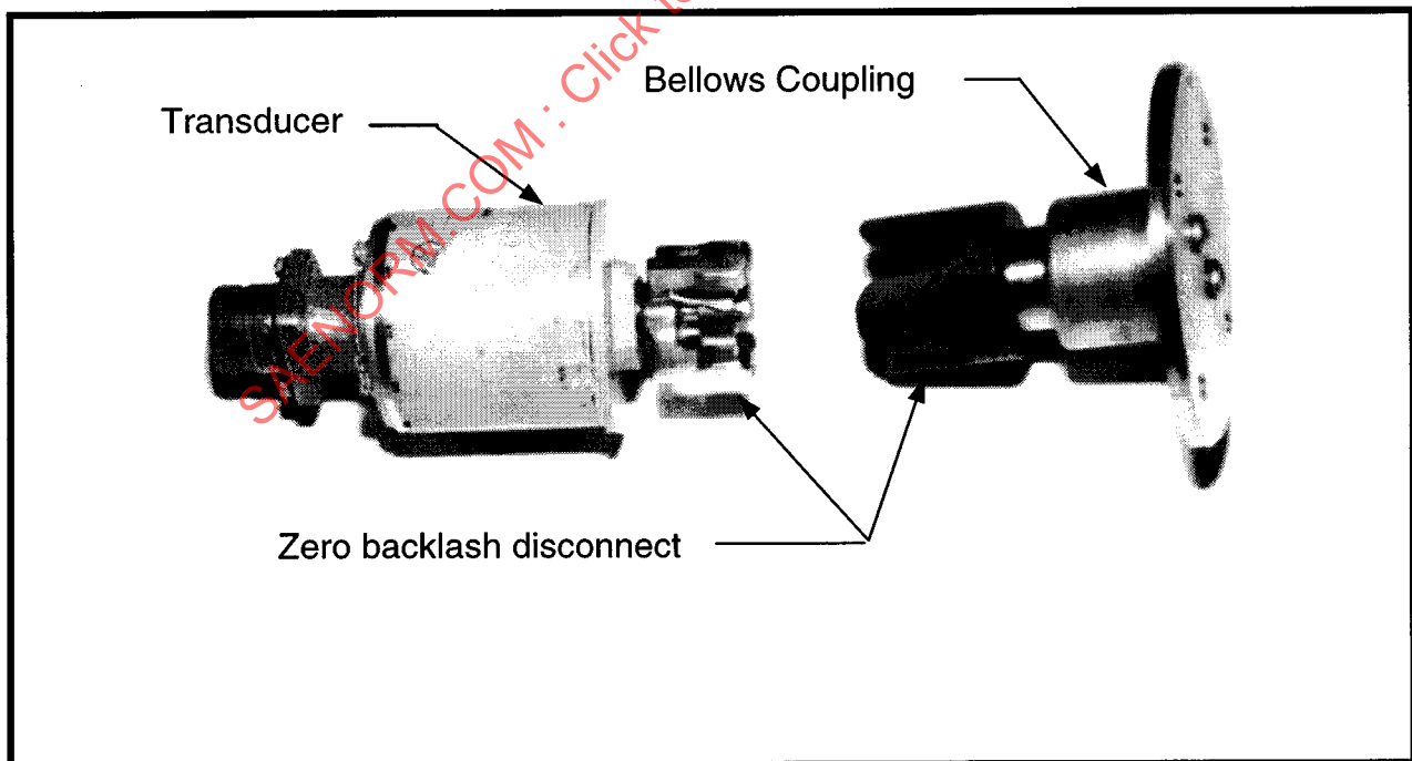
FIGURE 8 - Bellows Coupling
