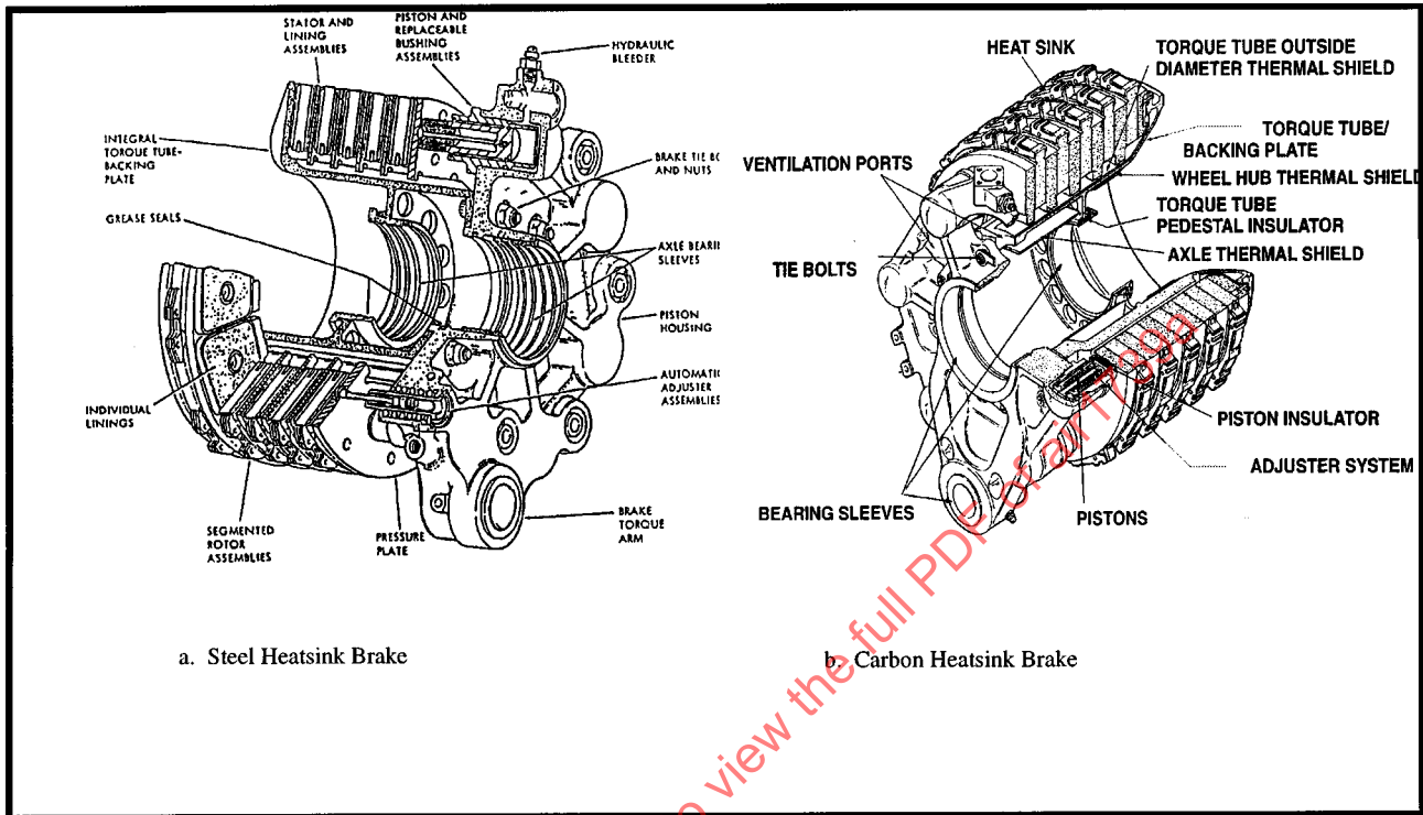
FIGURE 11 - Typical Aircraft Brake Assemblies
