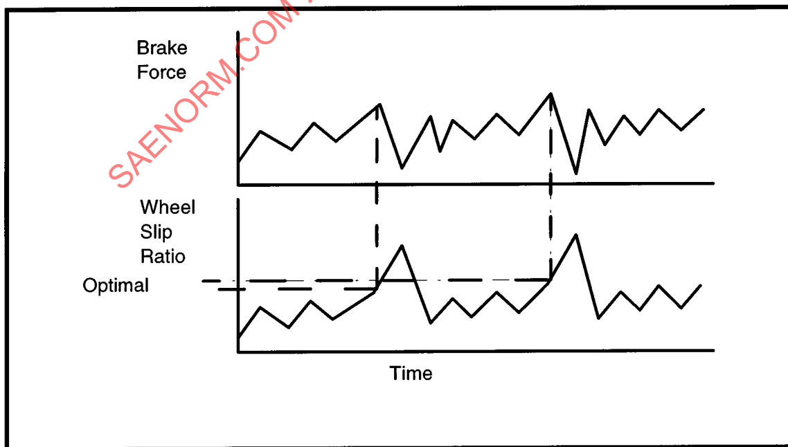
FIGURE 16 - Optimum Slip Ratio Determination
