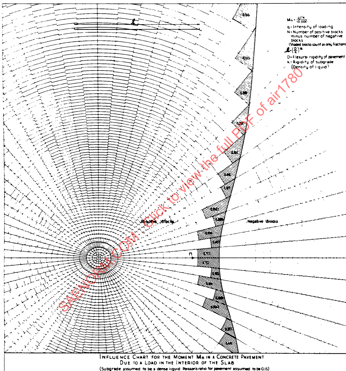
Figure 6. Influence Chart for Rigid Pavement Analysis
