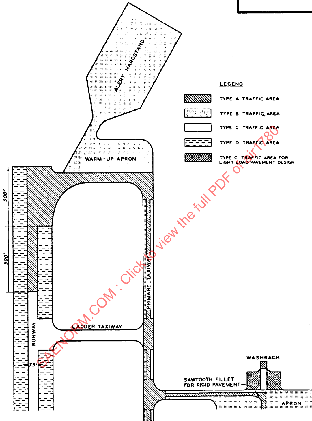
Figure 2. Typical Layout of Air Force Heavy - Load Pavements
