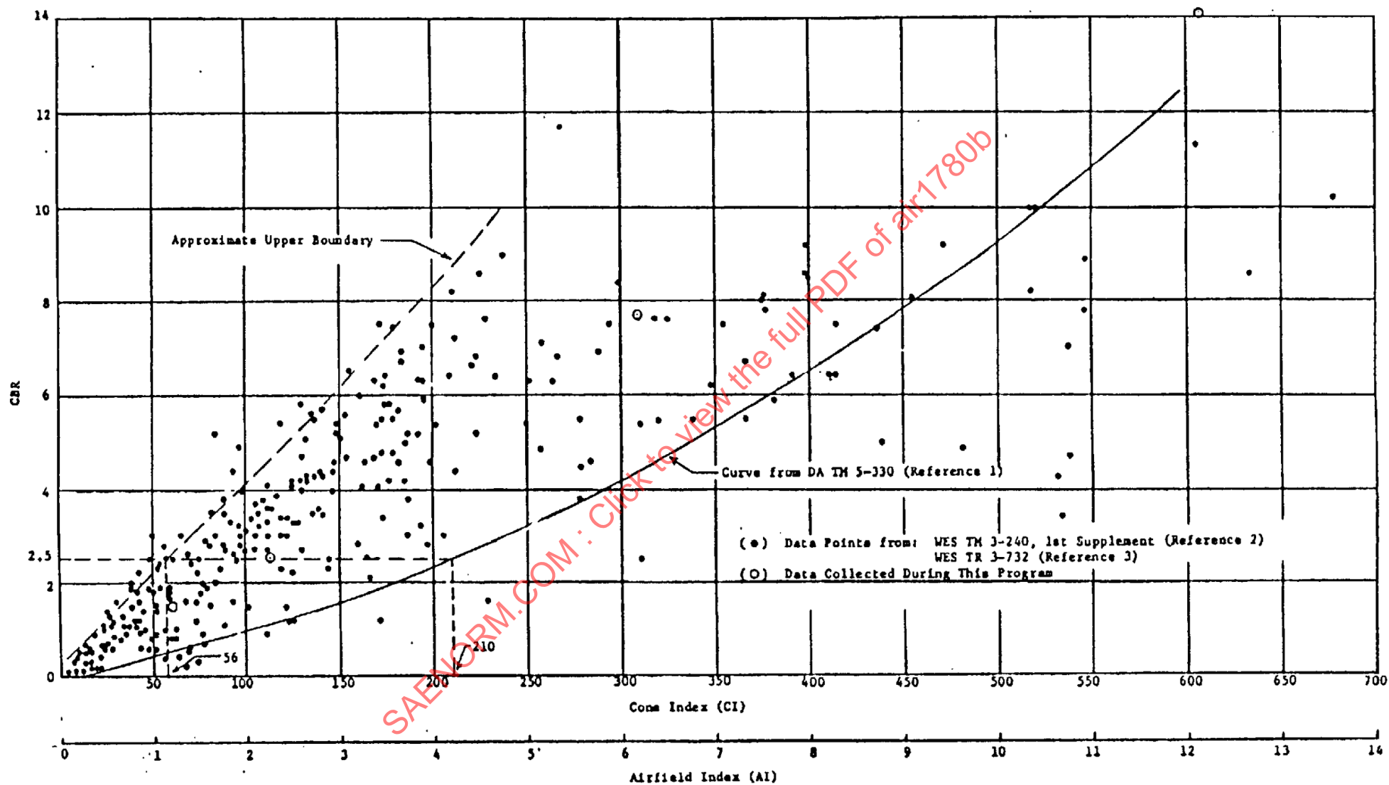
Figure 5 - Correlation of CBR, CI, and AI (fine-grained soils)
