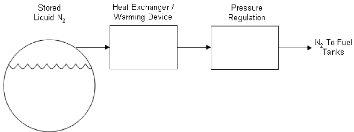
Figure 4 - Schematic of typical stored liquid nitrogen inerting system
