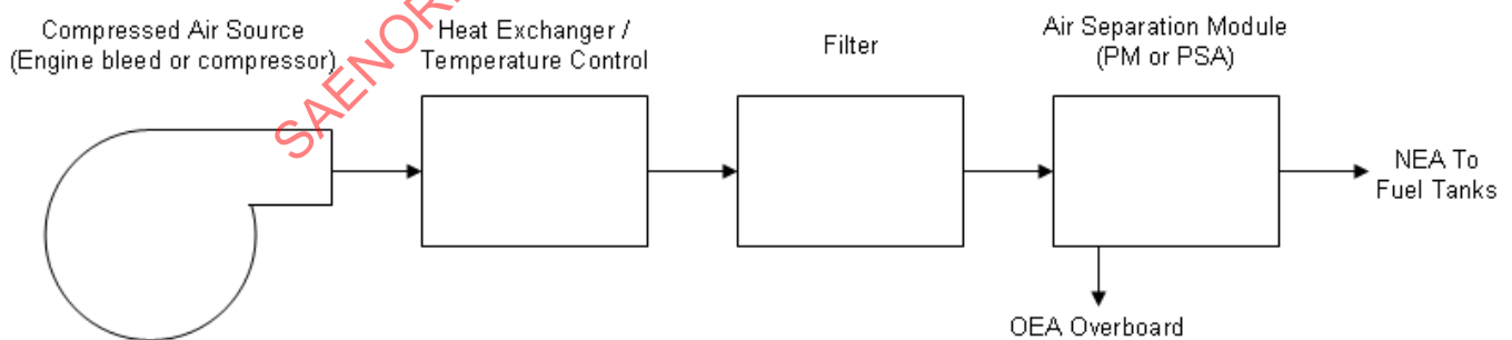
Figure 2 - Schematic of typical PM or PSA OBIGGS
