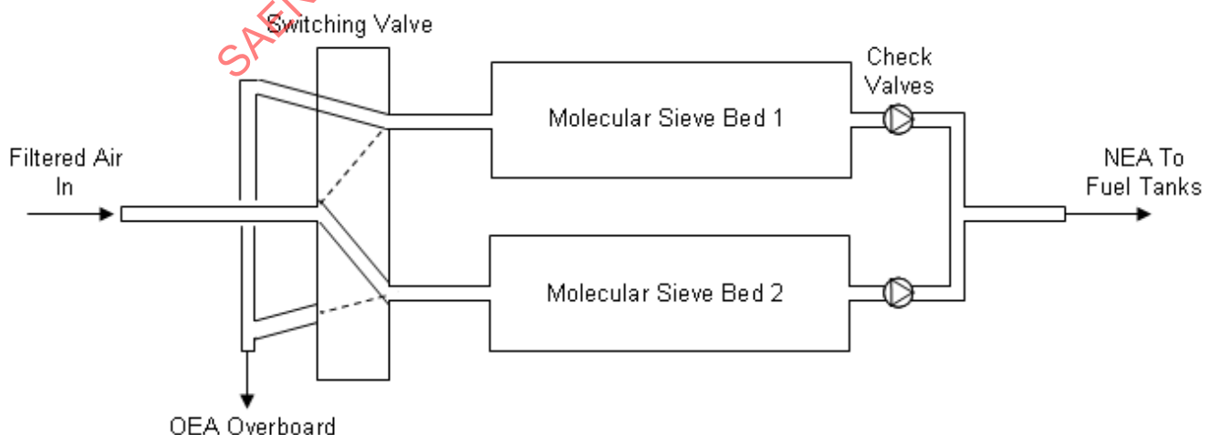
Figure 3 - Schematic of typical PSA inerting system
