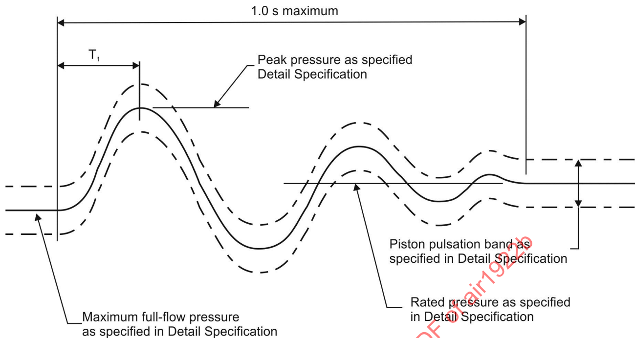
Figure 2 - Typical pressure transient full flow to zero flow
