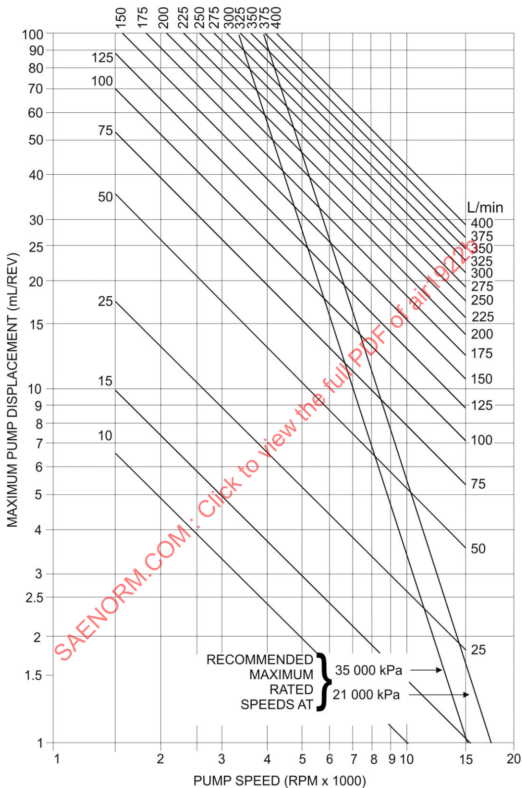
Figure 4D - Maximum pump displacement versus pump speed (metric units) – Military aircraft applications
