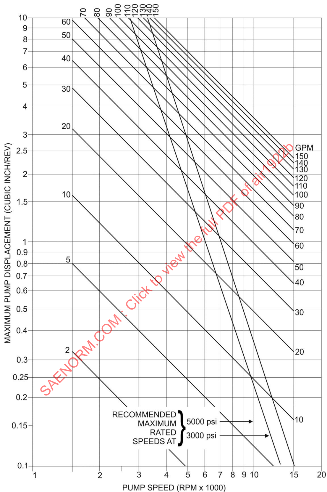
Figure 4C - Maximum pump displacement versus pump speed (imperial units) – Military aircraft applications
