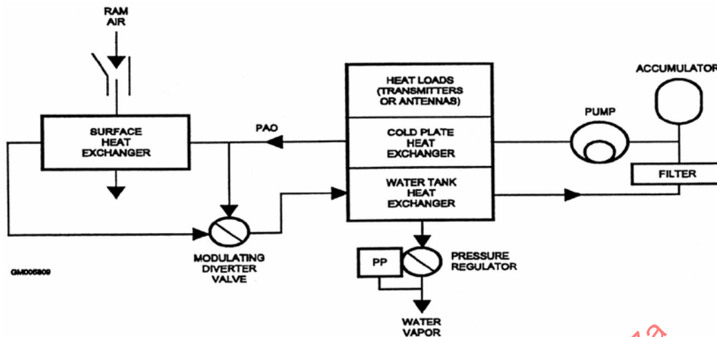
Figure 13 - Example of expendable water heat sink design
