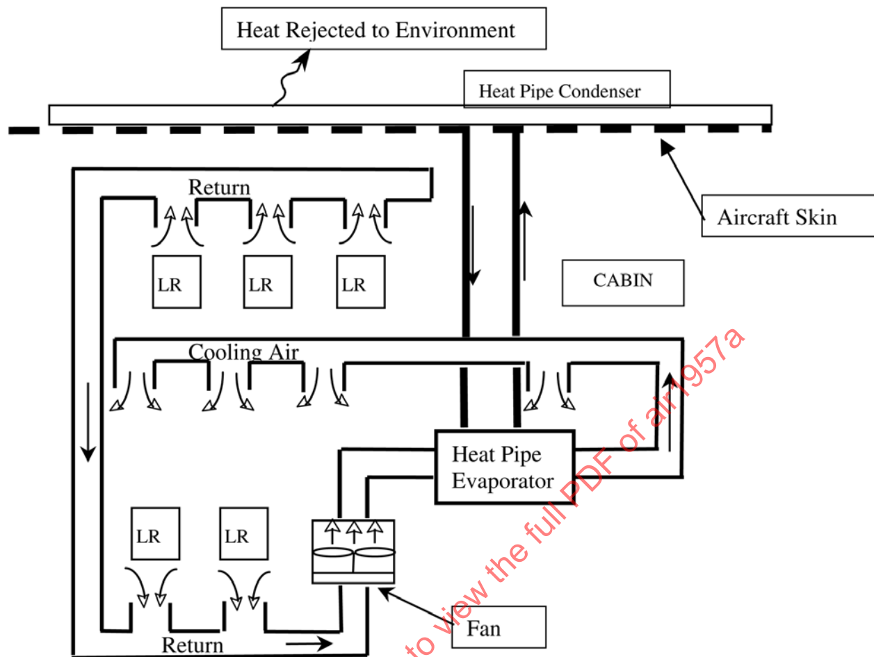
Figure 5 - Skin convective cooling with heat pipe
