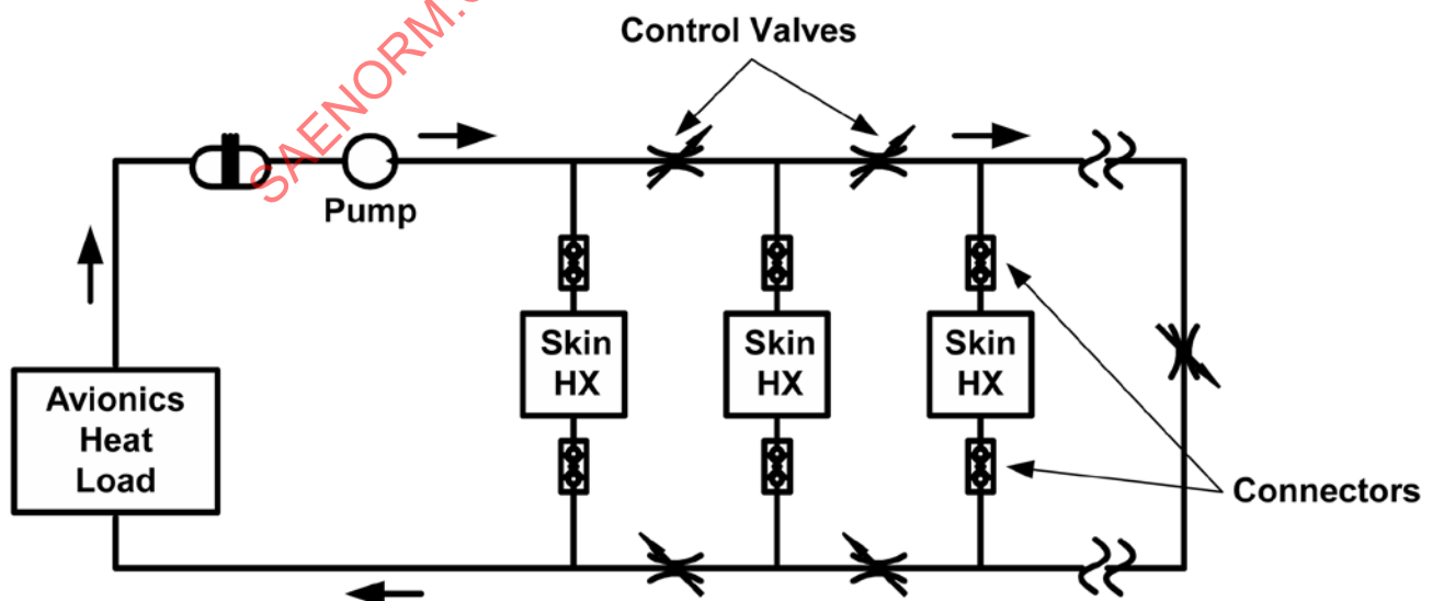
Figure 3 - Liquid-to-air skin heat exchanger
