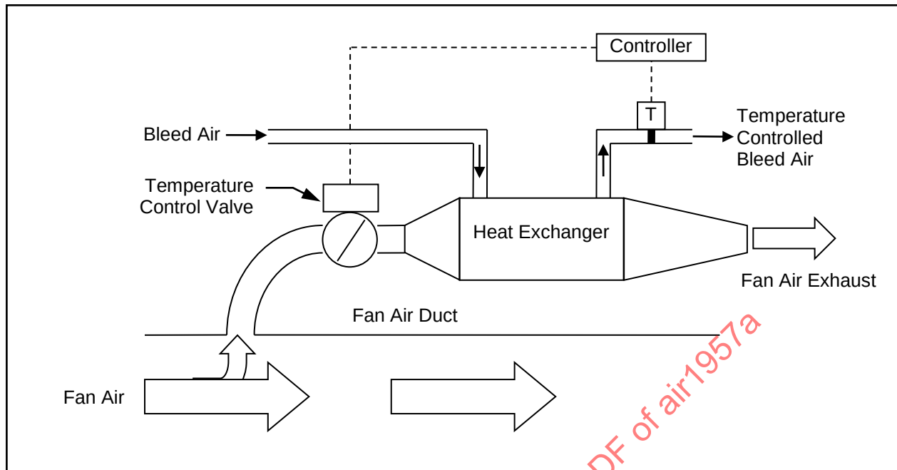
Figure 9 - Fan air extraction system with fan air modulation temperature control
