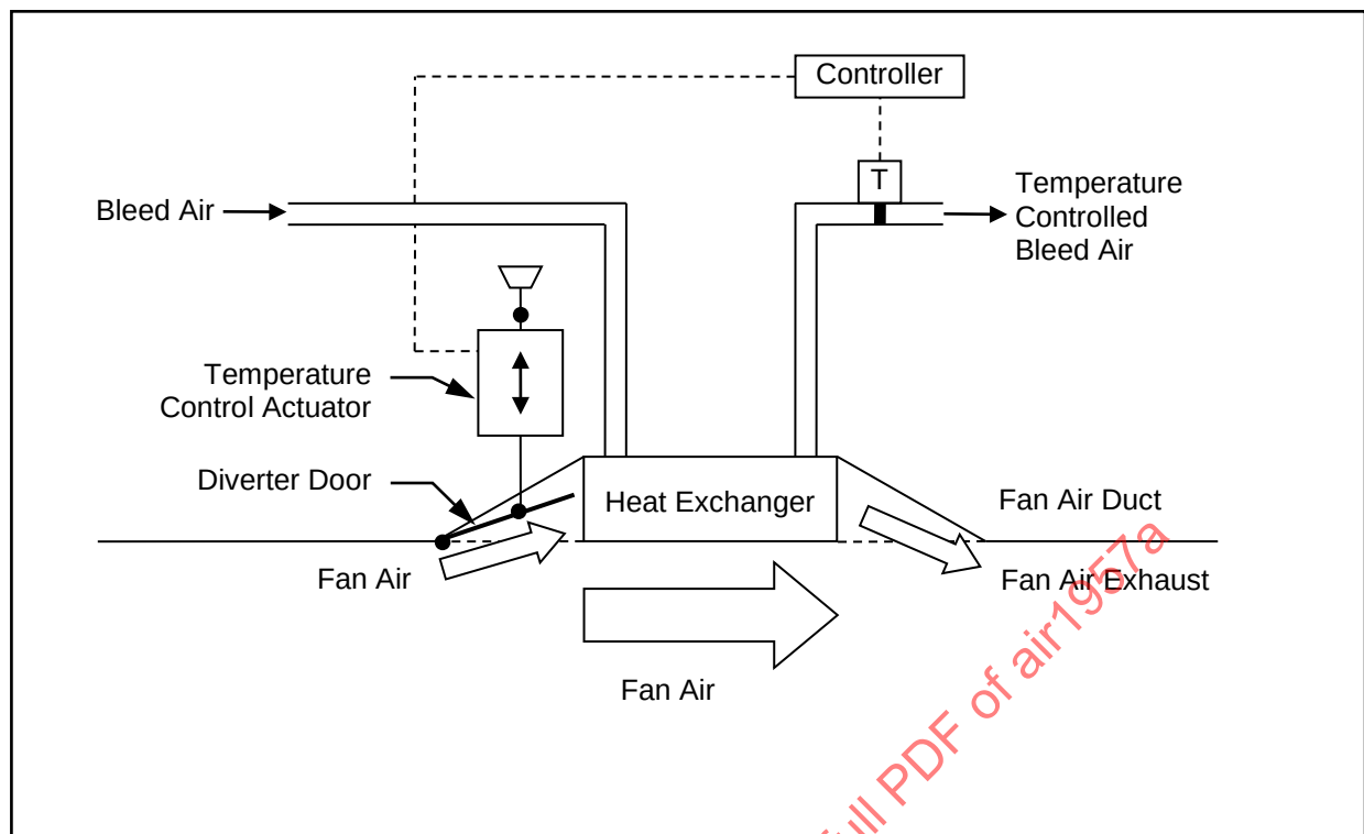
Figure 12 - Fully recessed fan duct heat exchanger with fan air modulation temperature control
