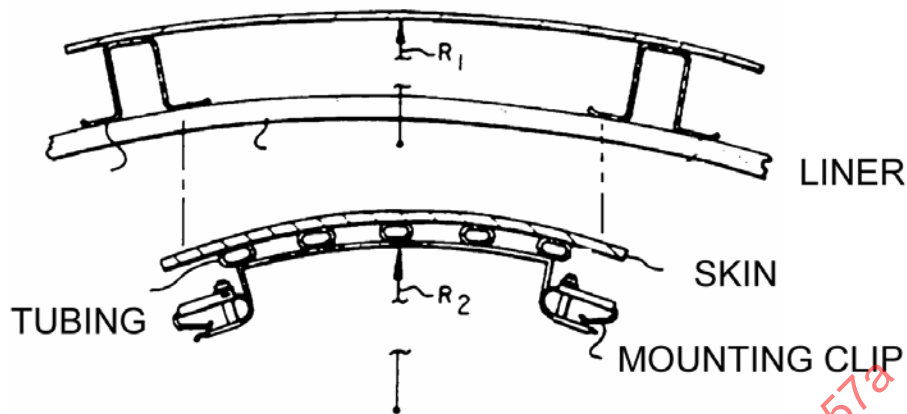
Figure 4 - Liquid-to-air skin heat exchanger cross-section
