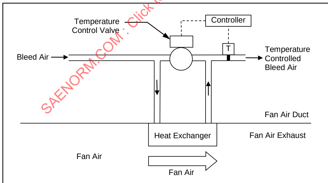
Figure 10 - Fan duct heat exchanger with bleed air modulation temperature control
