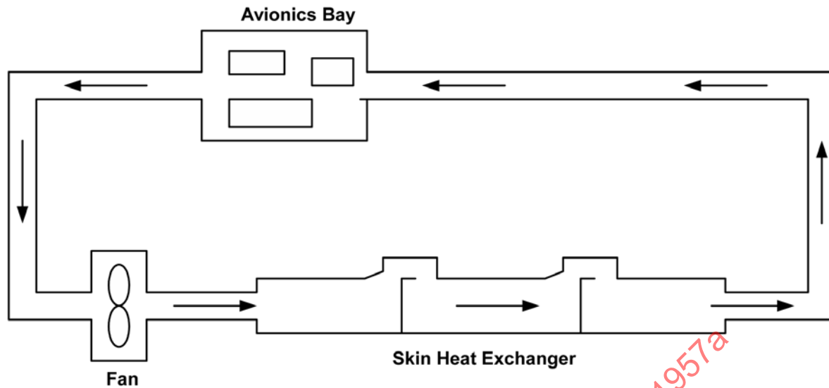
Figure 2 - Air-to-air skin heat exchanger
