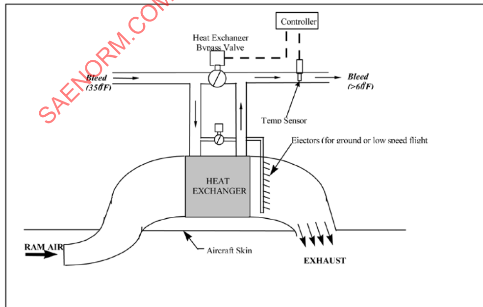
Figure 7 - Ram air heat sink with ejector augmentation
