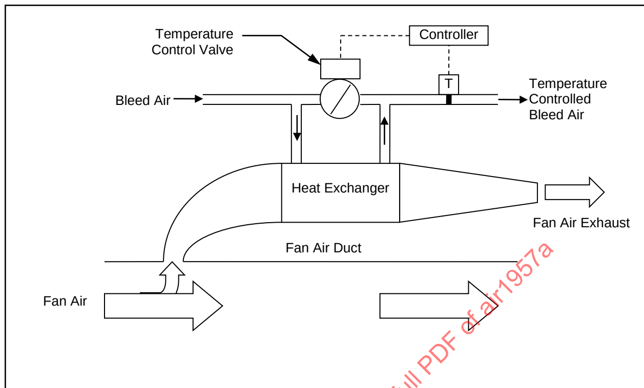
Figure 8 - Fan air extraction system with bleed air modulation temperature control
