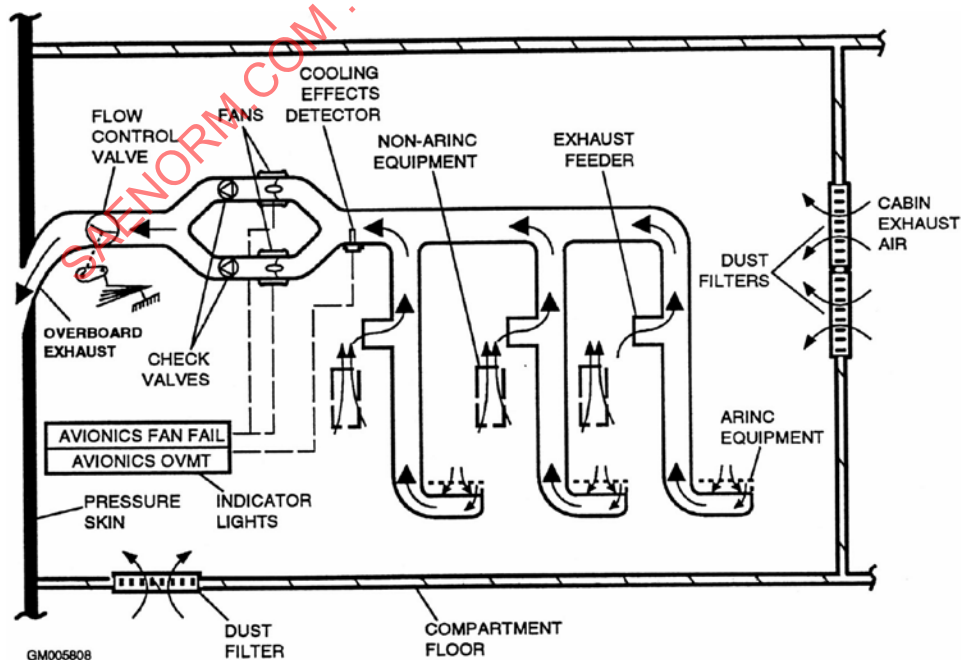
Figure 14 - Typical transport aircraft avionics cooling system
