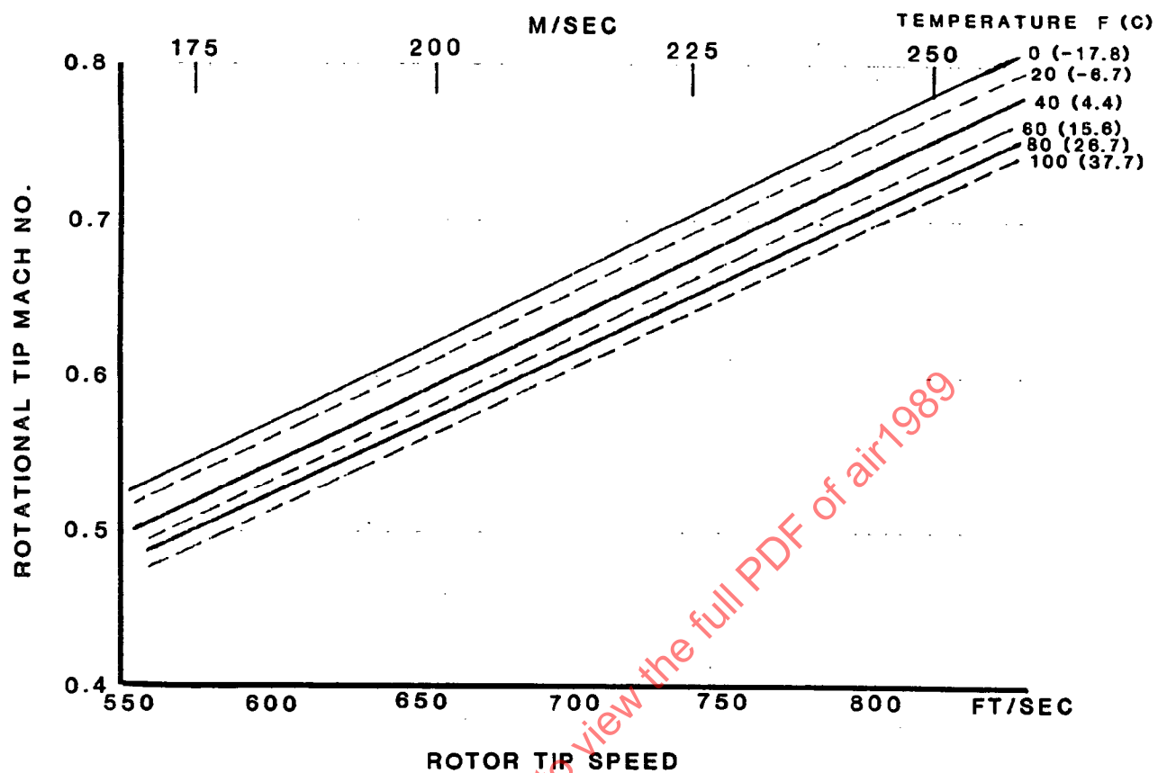
FIGURE 1 - Tip Mach No. ( M_T )
