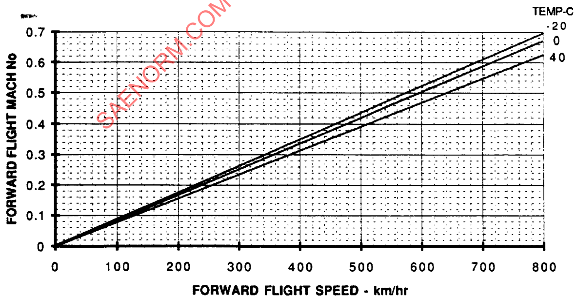
FIGURE 2 - Forward Flight Mach Number
