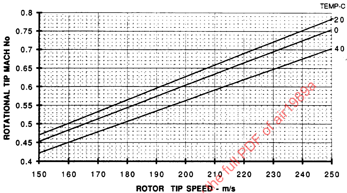
FIGURE 1 - Rotor Tip Mach Number
