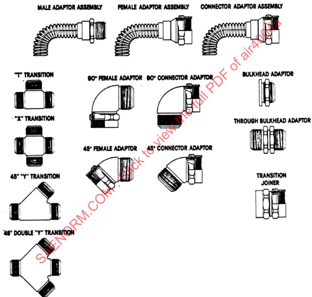
Figure 3 - Typical adaptors and transitions
