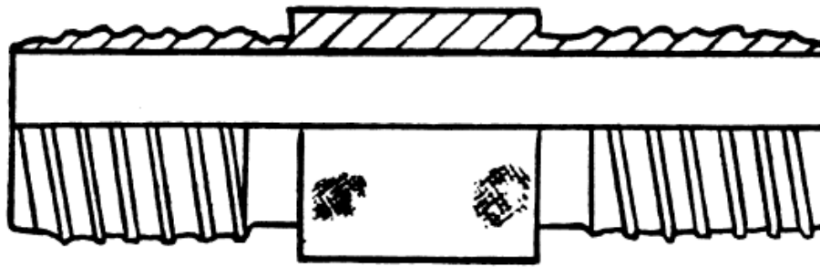
Figure 2 - Typical clamp adaptor
