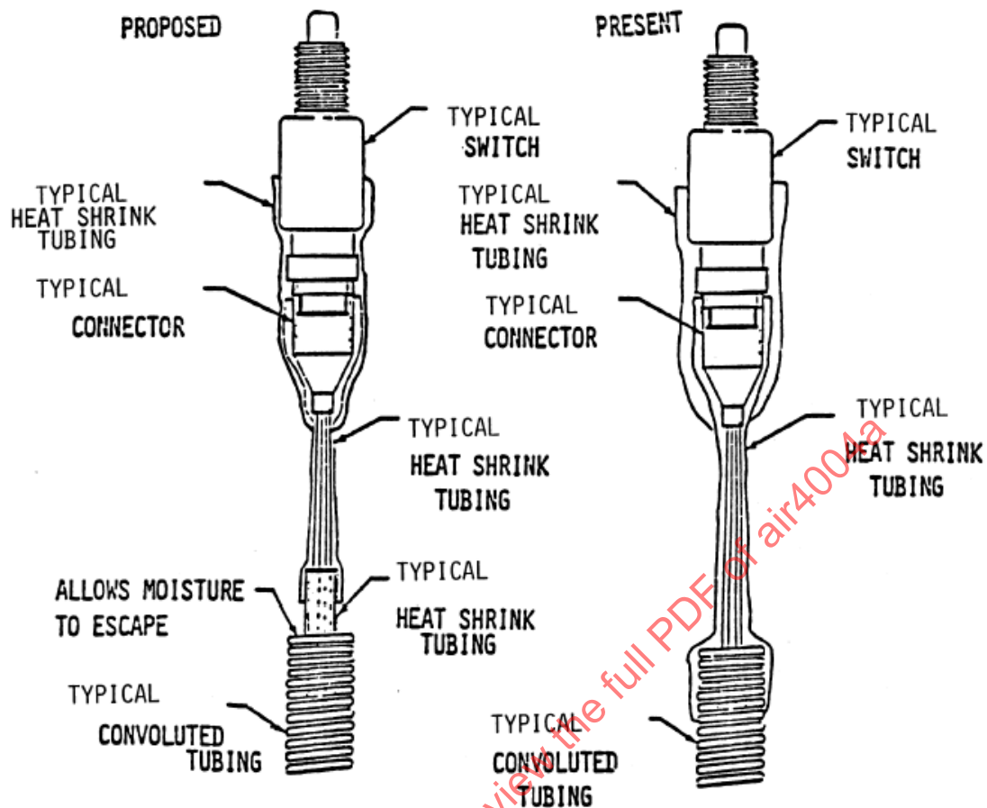
Figure 4 - Example of change to improve service life by elimination of trapped moisture
