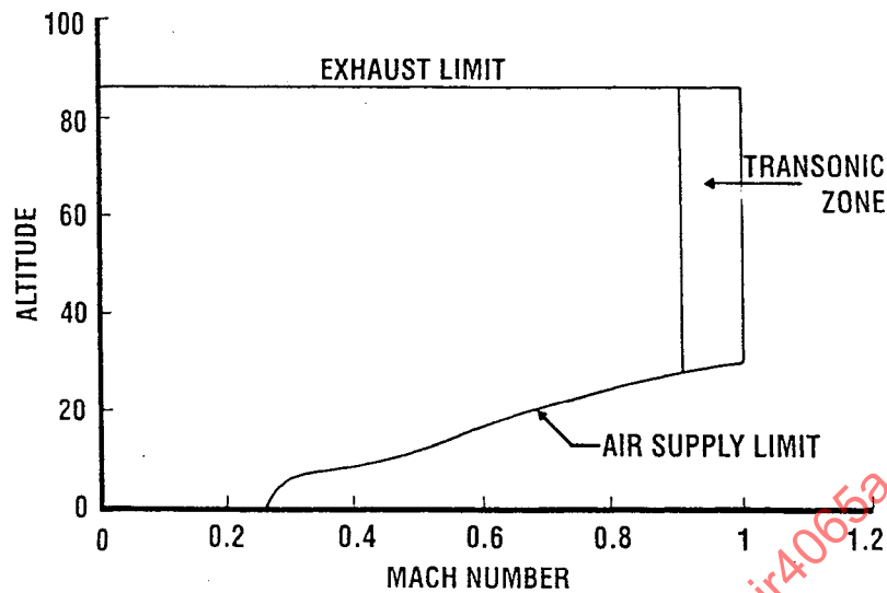
Figure 46 - AEDC Freejet Capability with 77 ft 2 Subsonic Nozzle
