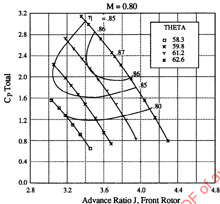
Figure 24 - Partial Efficiency Map (Counterrotation)
