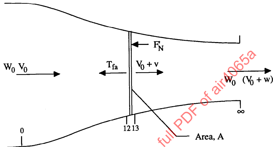
Figure A1 - Isolated Actuator Disc
