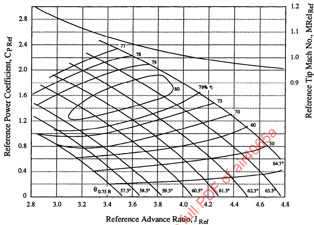
Figure 23 - Propeller Performance at Mach = 0.80
