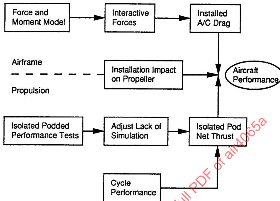
Figure 9 - Podded Installation Accounting System
