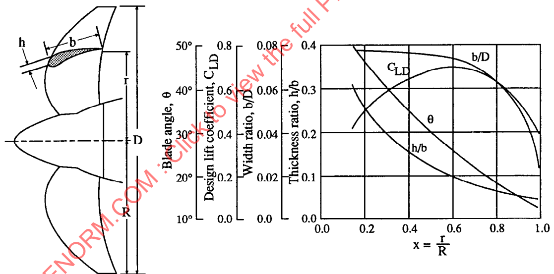
Figure 15 - Typical Blade Characteristic Data Sheet
