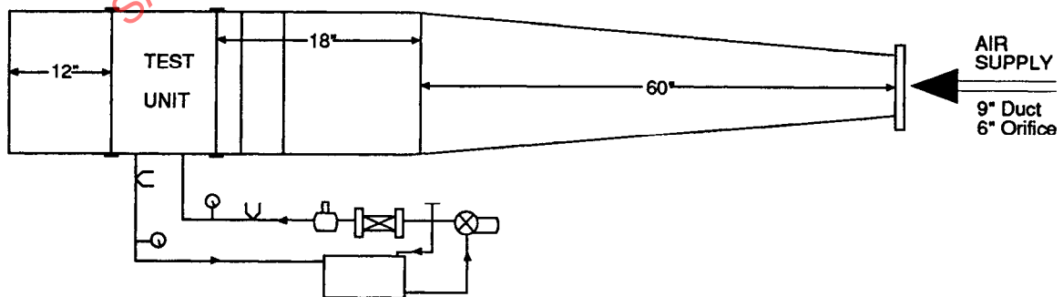
Figure B15 - Straight Duct Calibration (Installation and Instrumentation)
