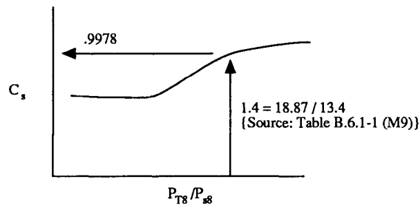
Figure B26 - C_s vs P_{T8}/P_{s8}
