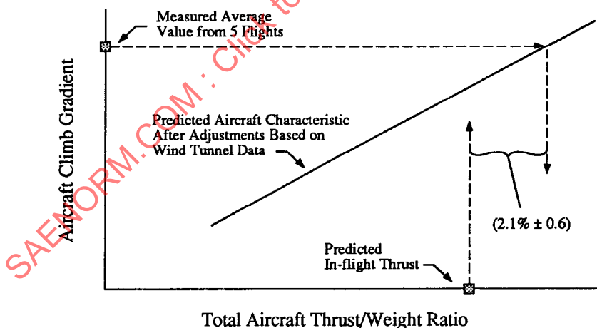
Figure B35 - In-flight Thrust Calculation Comparison
