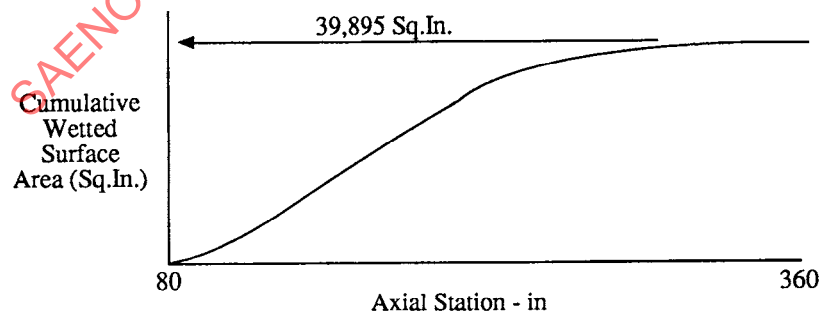
Figure B30 - Surface Area Distribution
