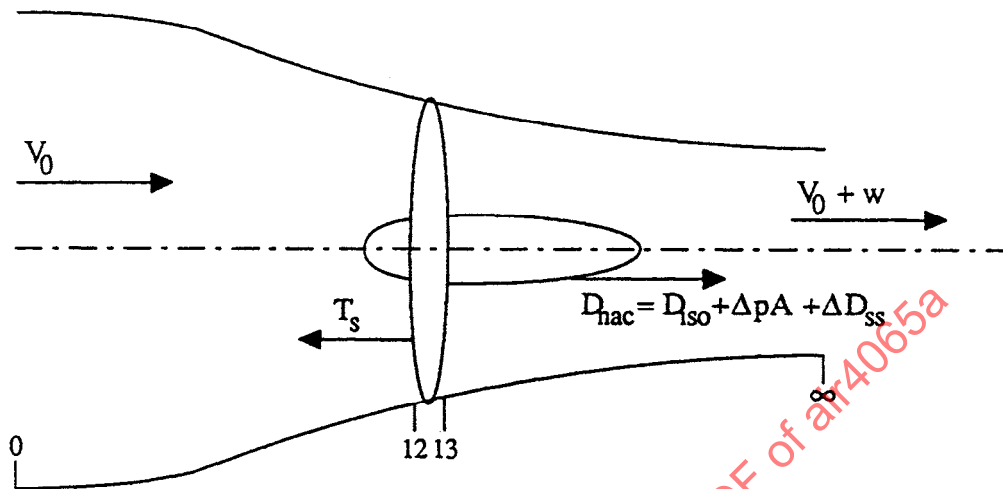
Figure 3 - Apparent Thrust for Propeller plus Centerbody
