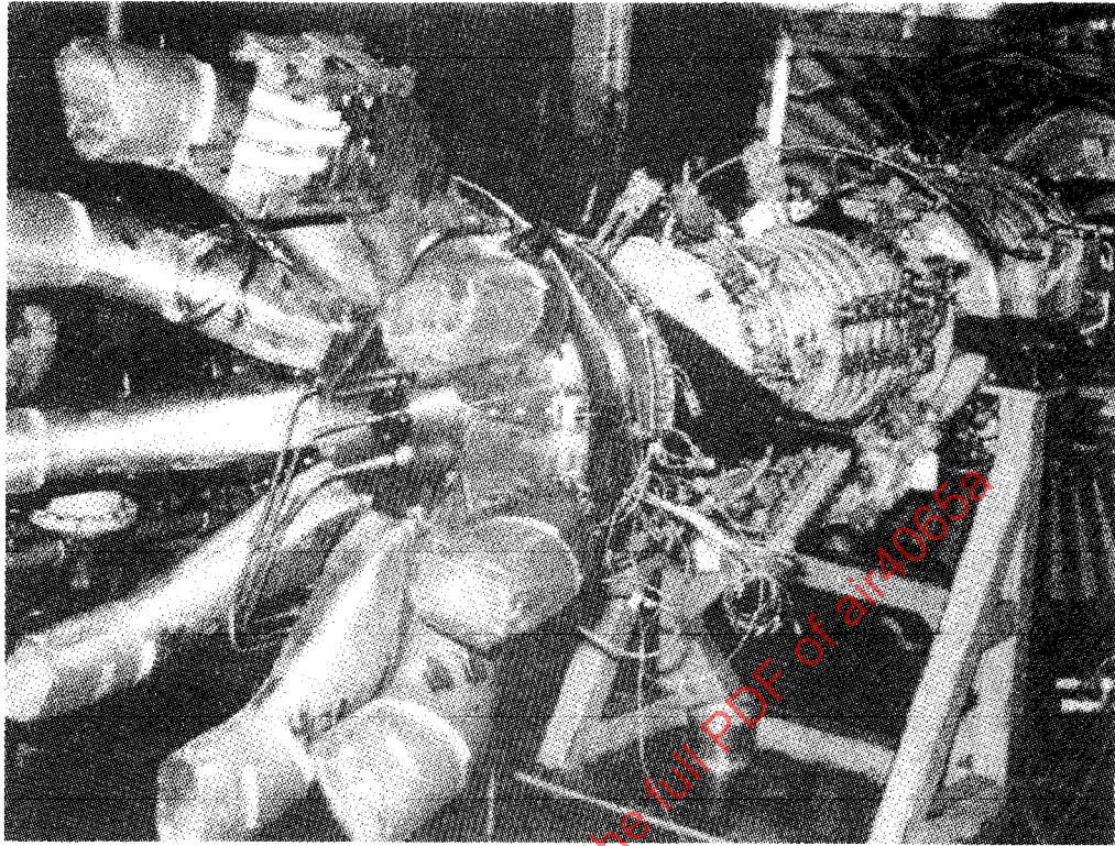
Figure B2 - 578-DX Lobe Nozzle Assembly
