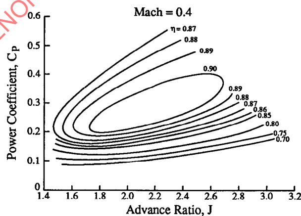
Figure 22 - Efficiency Chart for a Typical Propeller - Mach = 0.4
