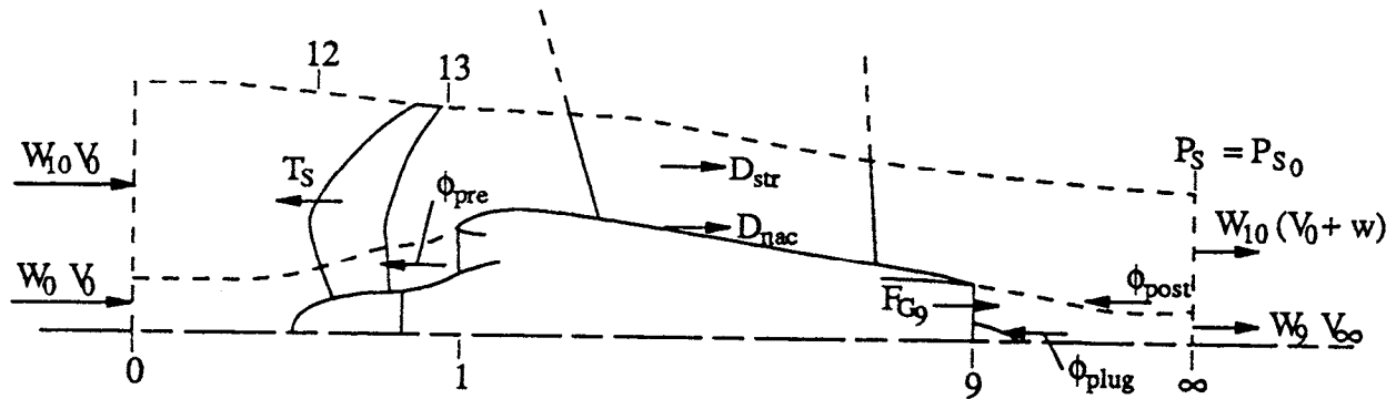
Figure 5 - Tractor Propeller with Body and Structure
