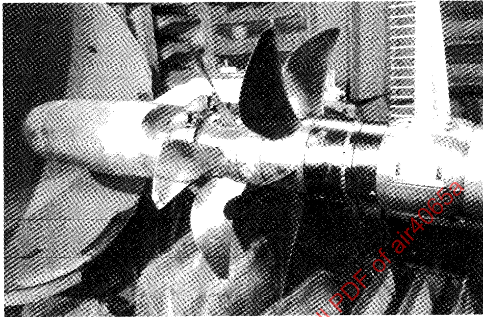
Figure B7 - Close Up Photo Showing Lobed Nozzles/Nacelle Positioned In Front of Test Propeller
