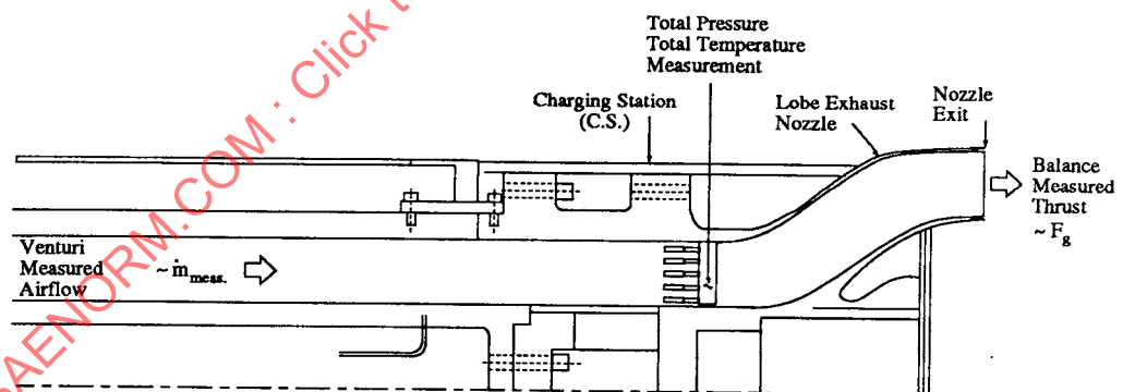
Figure B9 - Typical Nozzle Model Test Arrangement
