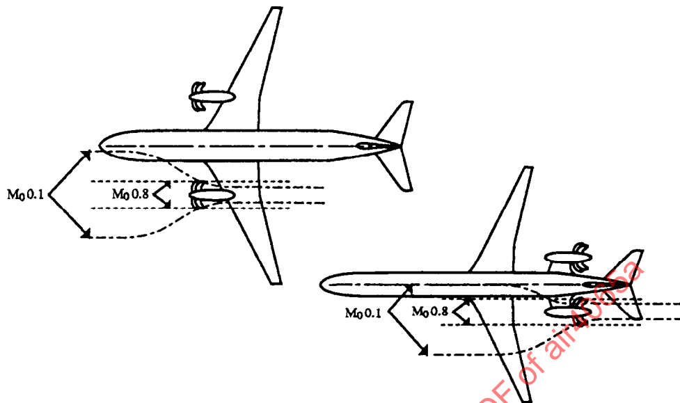
Figure 7 - Propeller Capture Stream Tube Coverage
