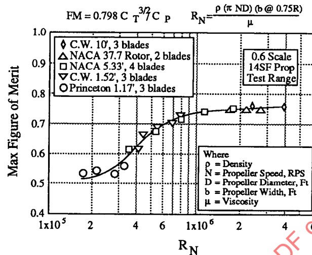
Figure 30 - Sample of Performance Correction
