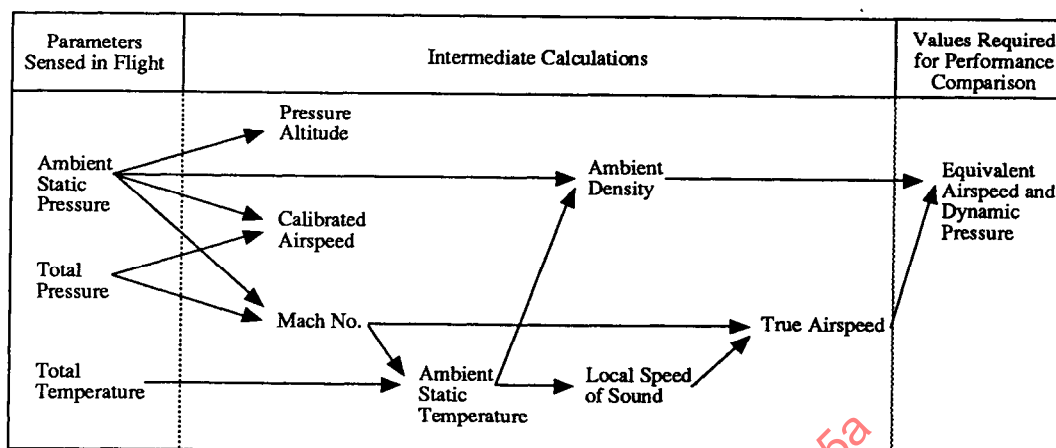
Figure 50 - Relation of Sensed Parameters to Required Performance Aerodynamic Data
