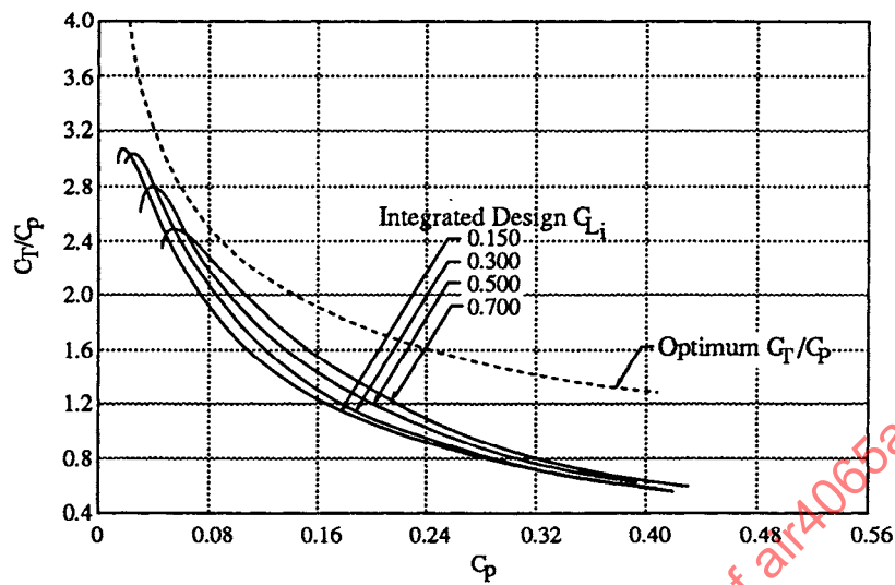
Figure 19 - Typical Static Performance Chart
