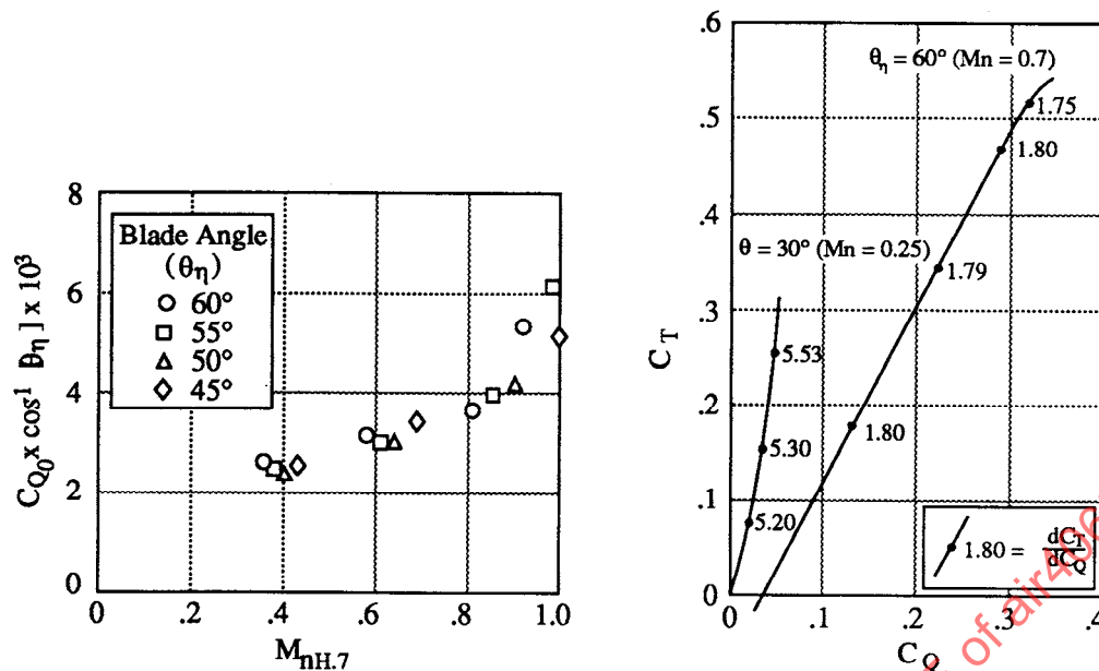
Figure 29 - Linearity of Constant Blade Angle Plot
