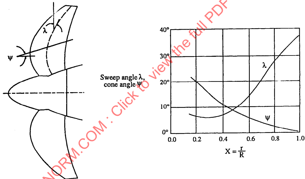
Figure 16 - Definition of Sweep and Cone Angles
