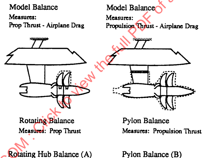
Figure 8 - Examples of Test Set-up Affecting Thrust/drag Definition
