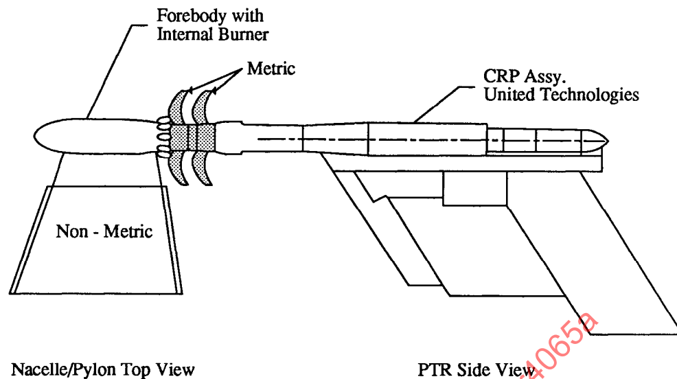
Figure B6 - Counter Rotation Propeller Test Rig - 2 Ft Diameter Blades
