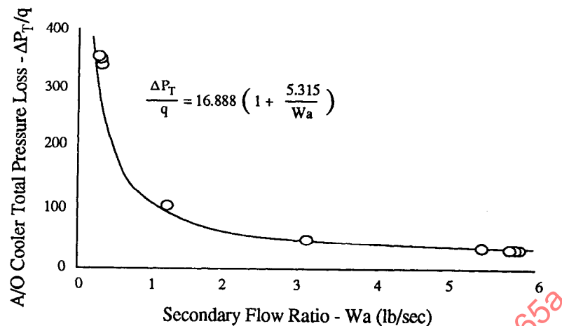
Figure B16 - Total Pressure Loss Through A/O Cooler
