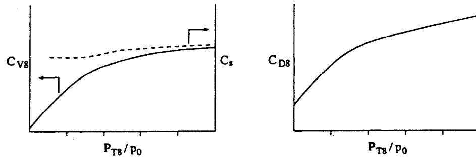
Figure B10 - Lobe Nozzle Thrust and Flow Coefficients
