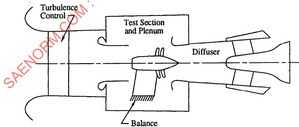
Figure 47 - Full Scale Self Powered Rig
