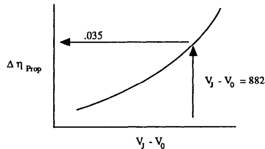
Figure B24 - Loss in Propeller Efficiency due to Jet Effect
