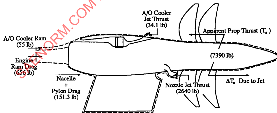
Figure B34 - Summation of Forces to Quantify Net Thrust
