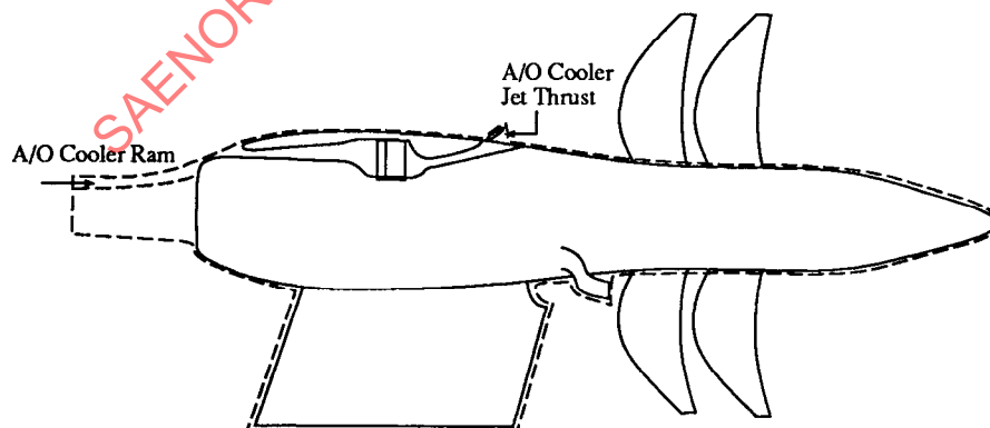
Figure B31 - Air/Oil Cooler Ram Drag
