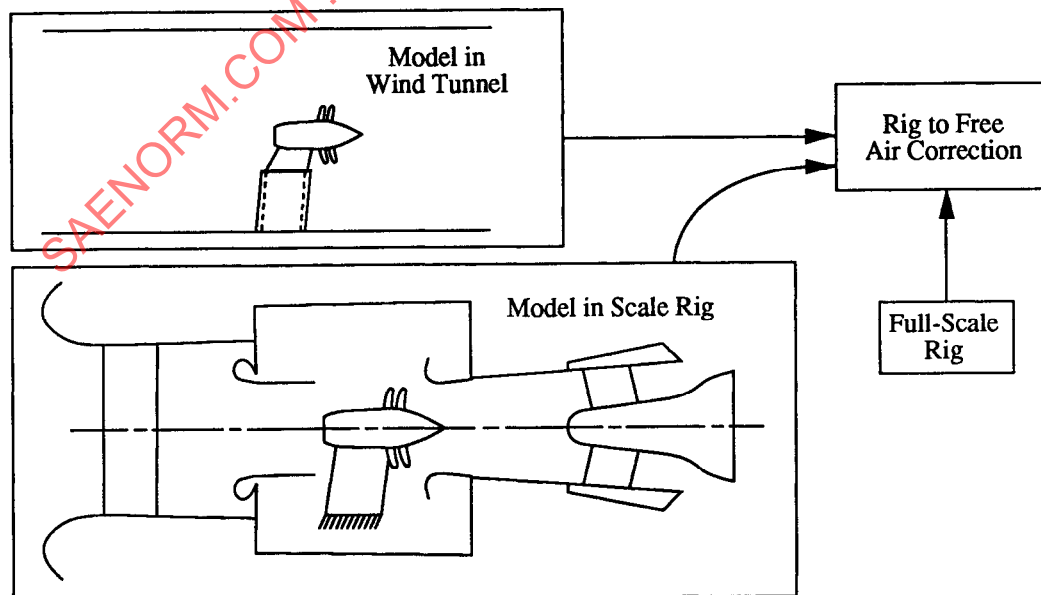
Figure 49 - Rig to Free Air
