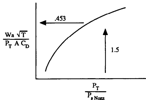
Figure B20 - Nozzle Curve
