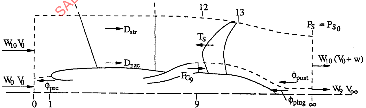
Figure 6 - Pusher Propeller Installation (Hot Gas Impingement)
