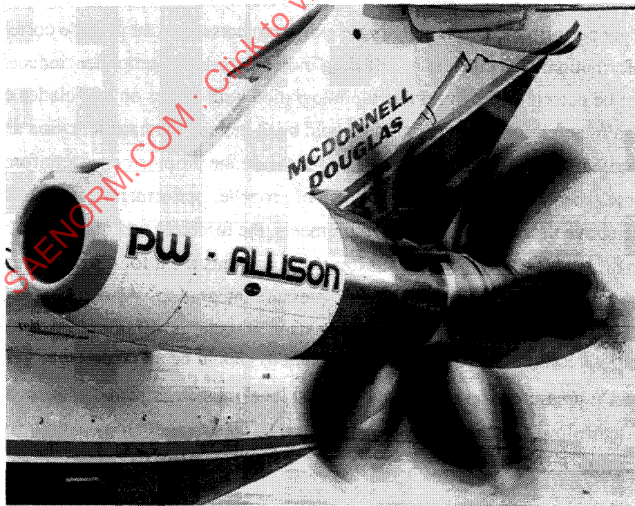
PW-Allison 578DX Demonstrator with exhaust nozzles ahead of propellers.
