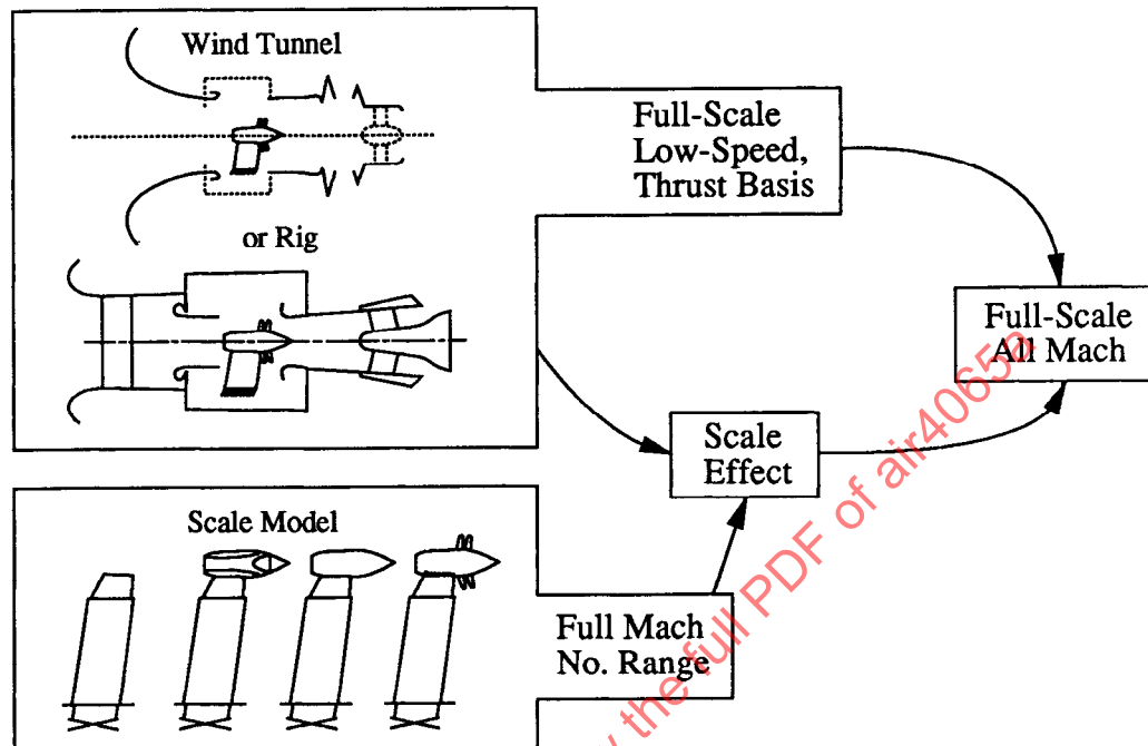
Figure 48 - Thrust Substantiation
