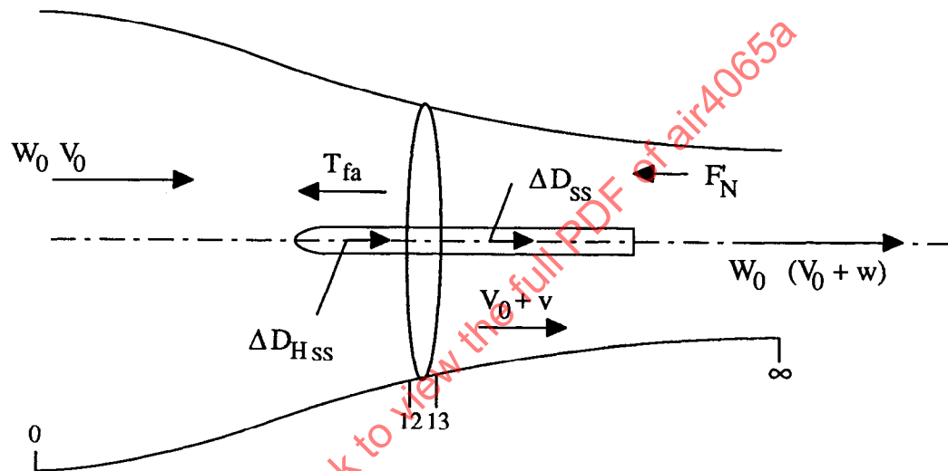
Figure A2 - "Isolated" Propeller Tested on a Propeller Test Rig (PTR)
