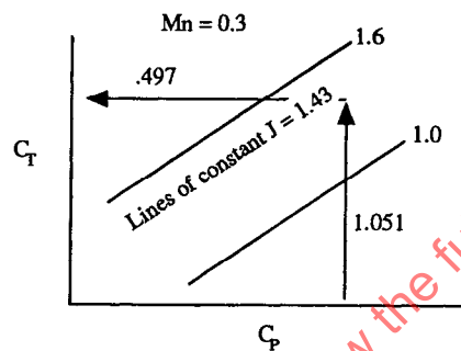
Figure B23 - Propfan Map
