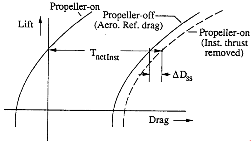
Figure 12 - Drag Polar Differencing for Integrated-Nacelle Propellers; Installed Net Thrust Method
