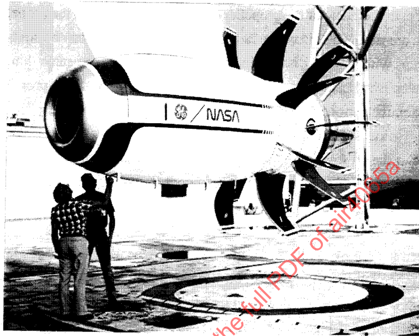
GE UDF Demonstrator with exhaust nozzle behind propellers.
