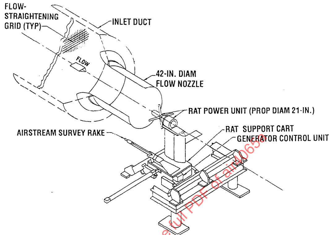
Figure 43 - Freejet Ram Air Turbine Test Installation Schematic
