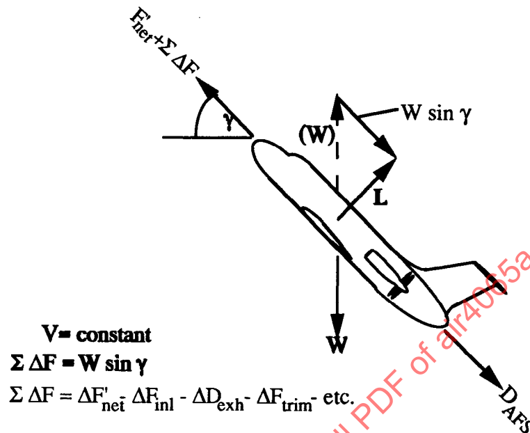
Figure 53 - Constant Speed Climb Validation of Thrust/Drag Increments from Full Scale Reference Condition
