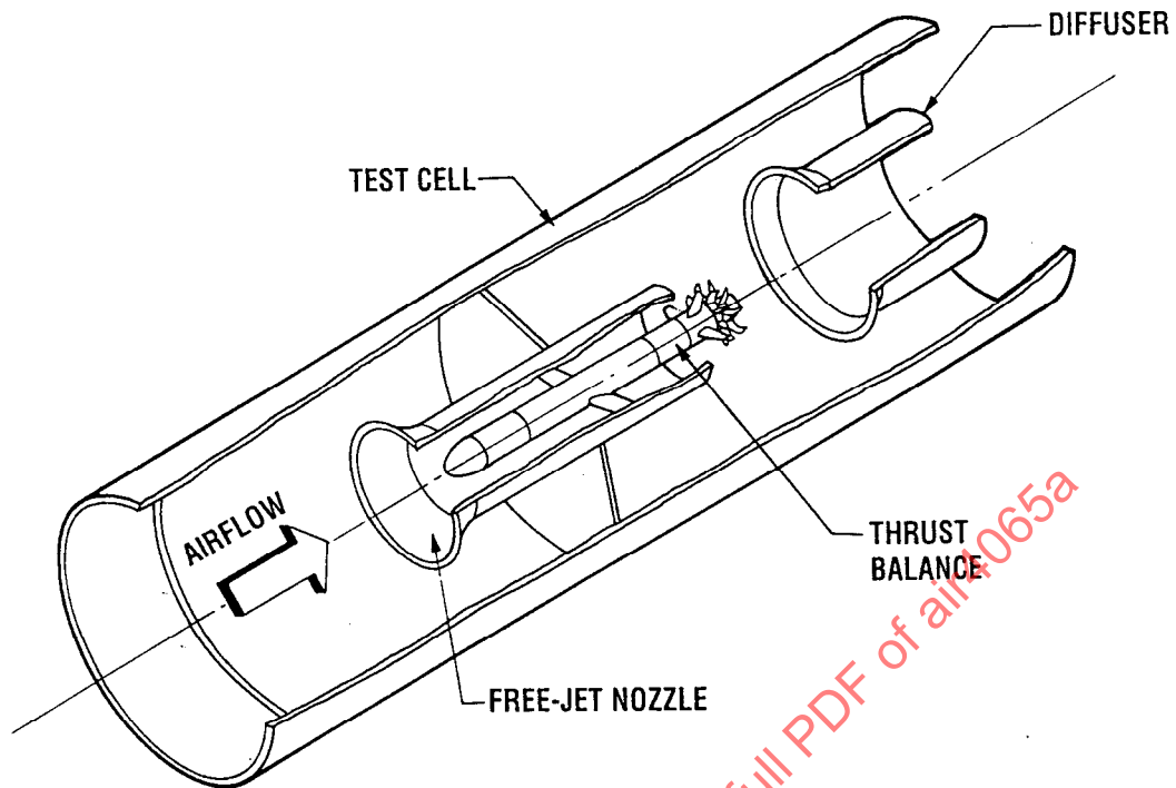
Figure 44 - Proposed Propfan Cruise Missile Freejet Test Installation Schematic
