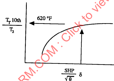
Figure B18 - Bleed Schedule
