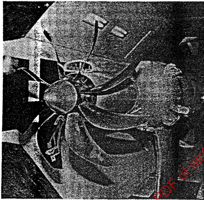
Figure 35 - Single-scoop Inlet with Diverter
