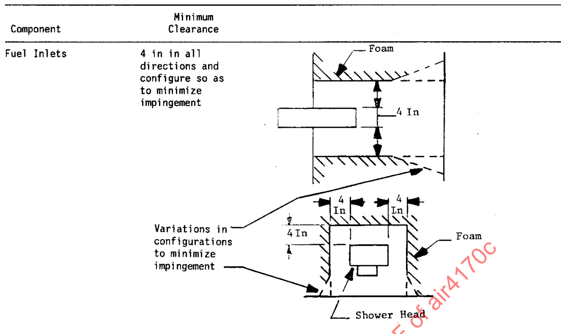
Figure 3 - Minimum clearance criteria (examples) dry, installed condition (continued)
