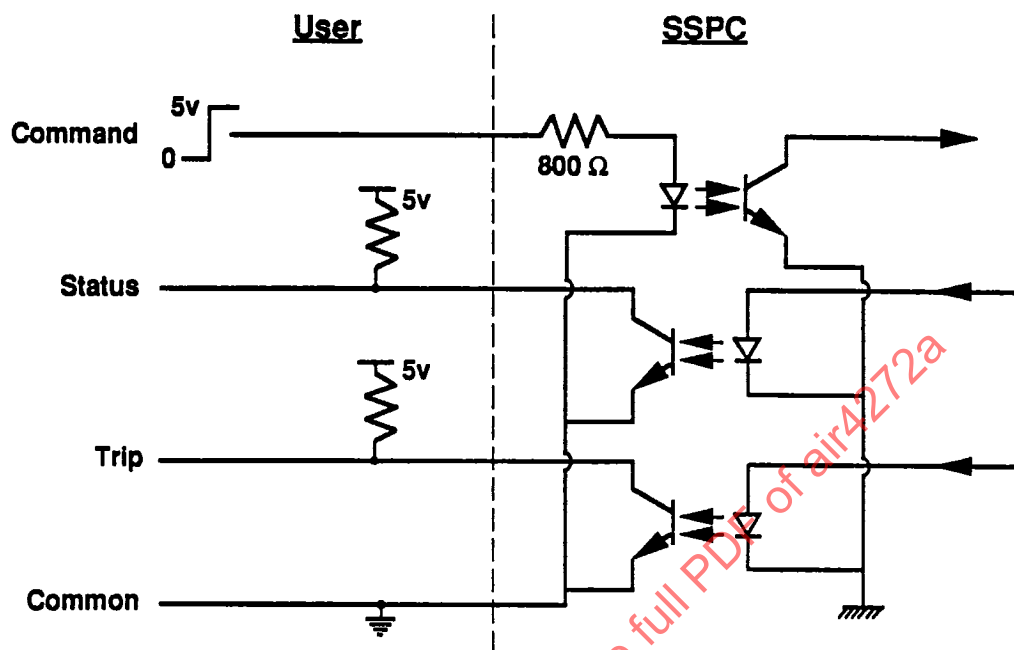
FIGURE 4 - TI SSPC Interface
