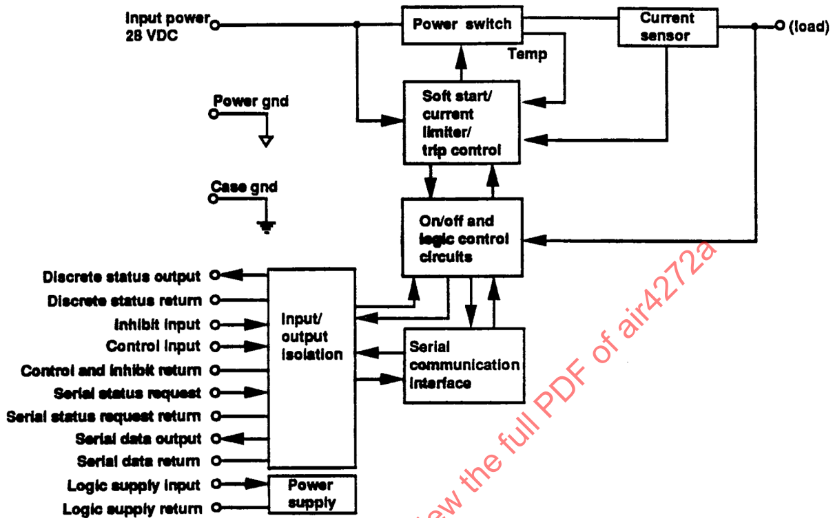
FIGURE 2 - Leach DC SSPC Interfaces
