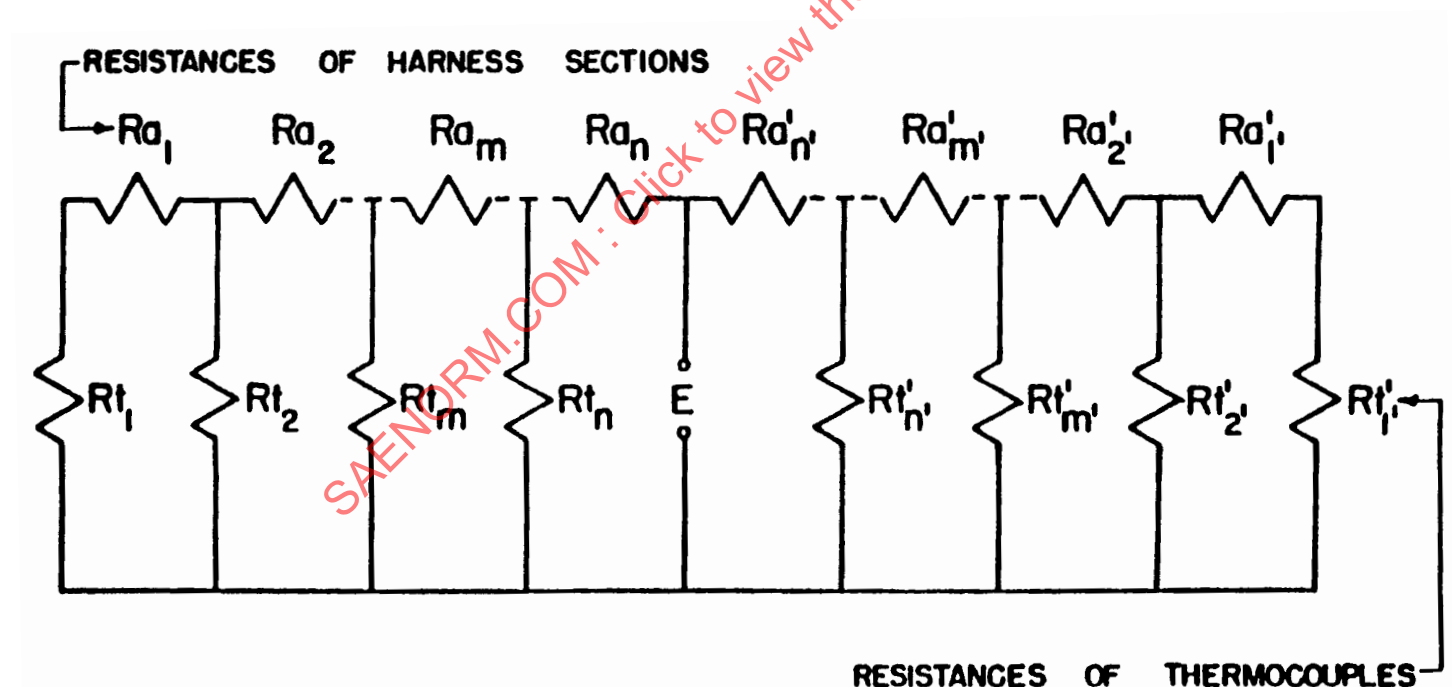
Figure 18 - Ladder-type system
