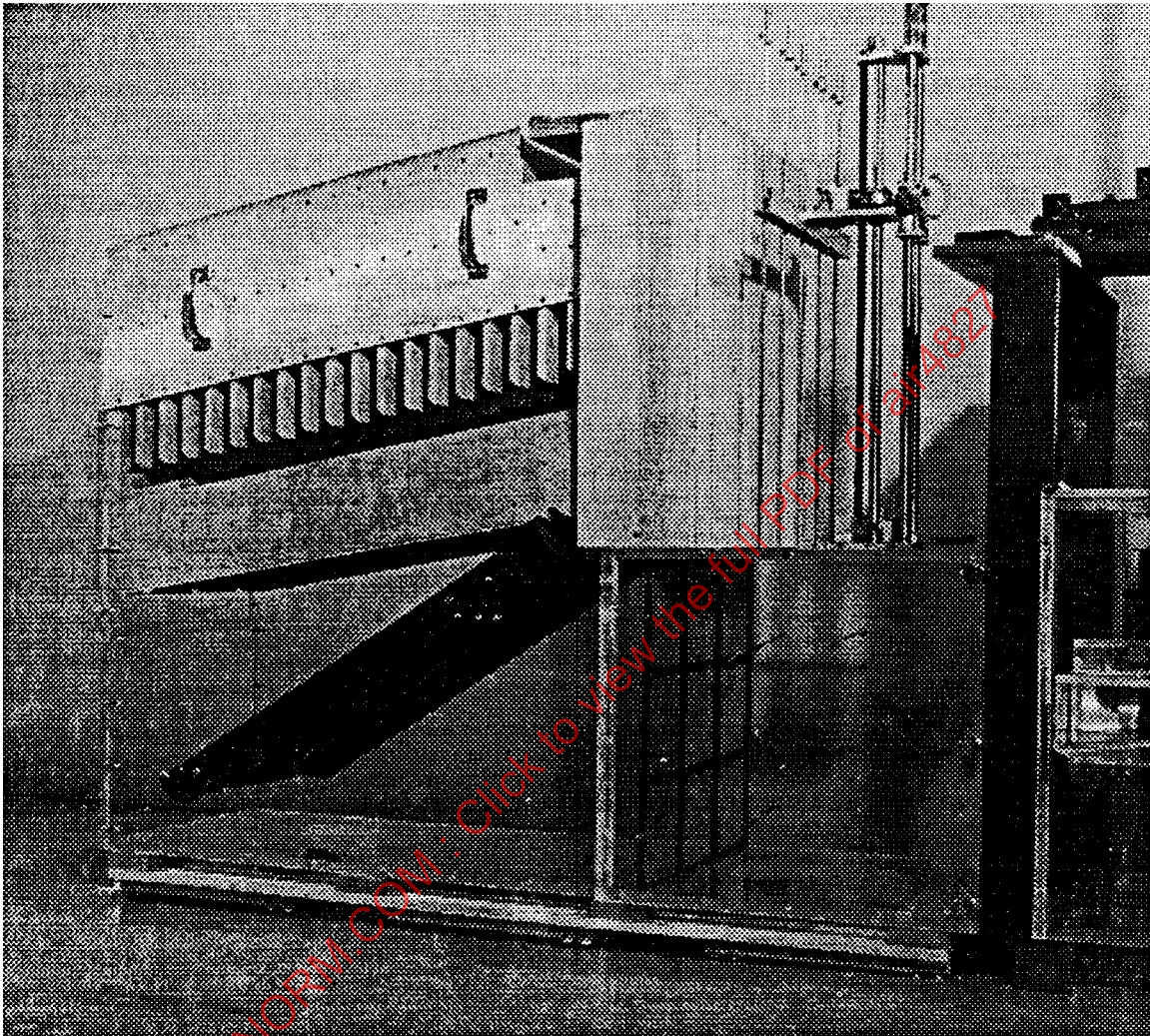
FIGURE 6 - Photograph of a Typical Installation of Hot Film Probes with Traversing System in the Front Cell Region of a Model Test Cell
