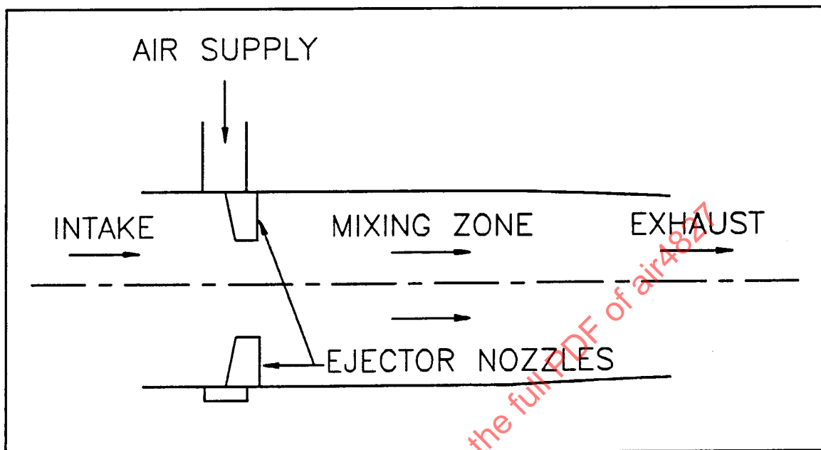
FIGURE 9 - Ejector-Powered Engine Simulator Interior Flow Features
