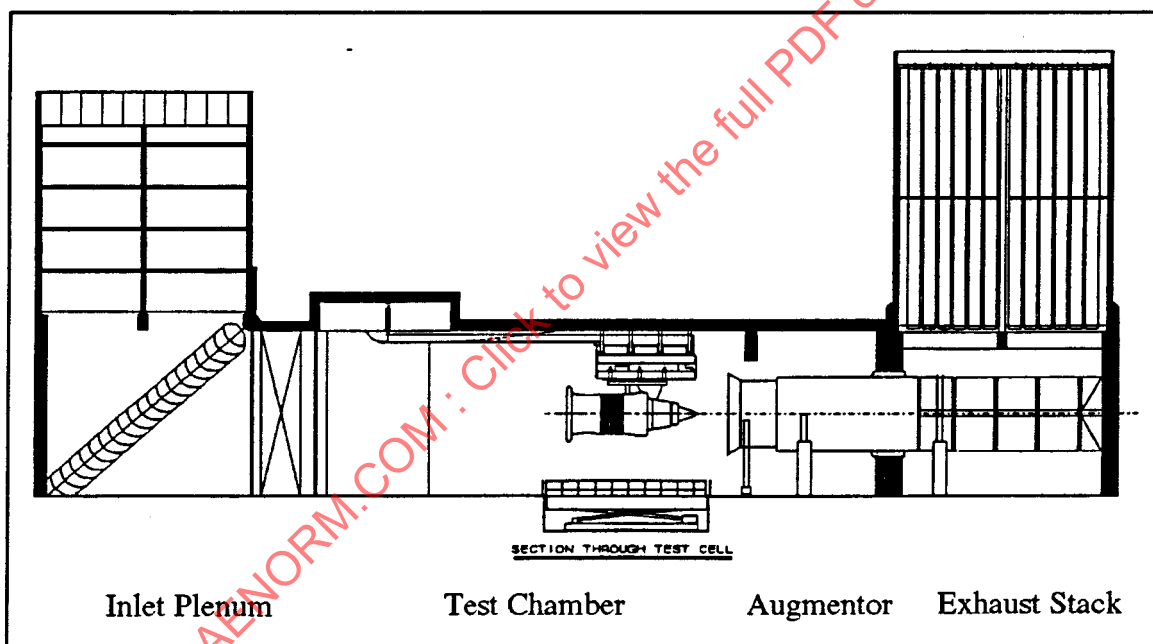
FIGURE 4 - General Design Concepts for an Engine Test Cell for a Large, High-Bypass Turbofan Engine
