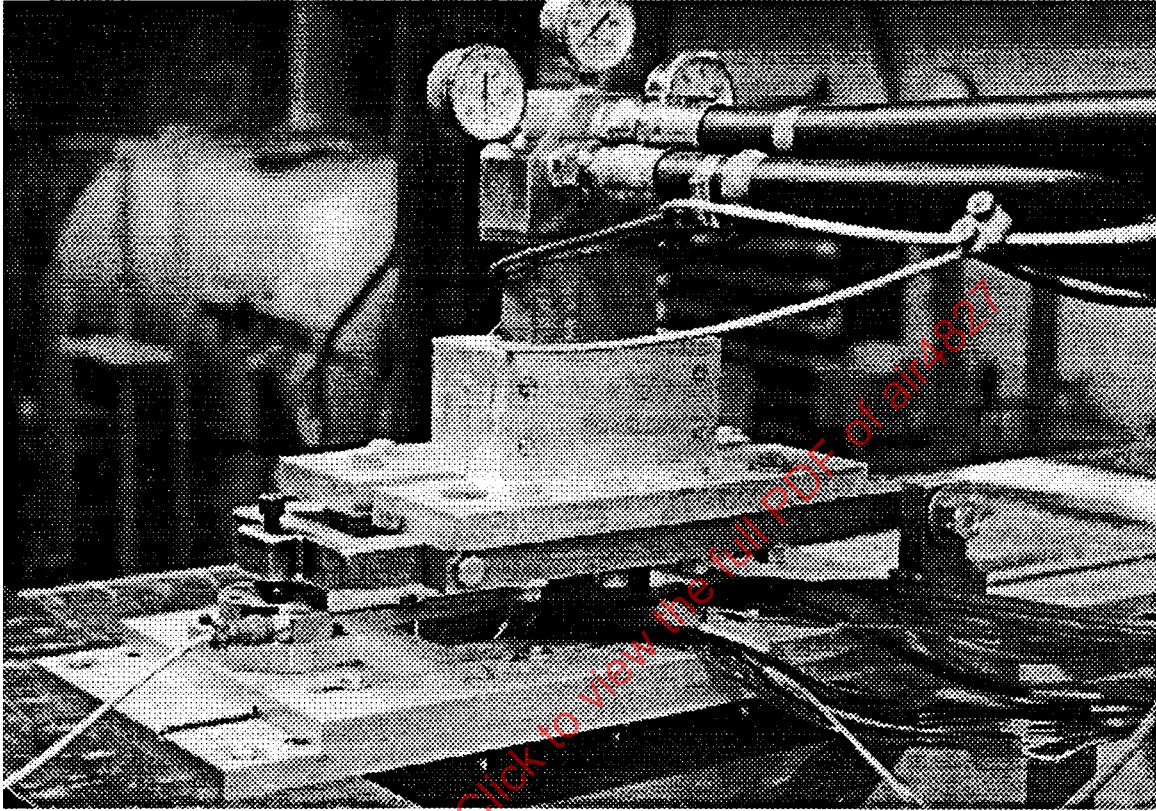
FIGURE 7 - Photograph of a Typical Installation of the Ejector Drive Air Supply Strut for the Engine Simulator and the Thrust Measuring System Using a Conventional Load Cell for the Force Measurement
