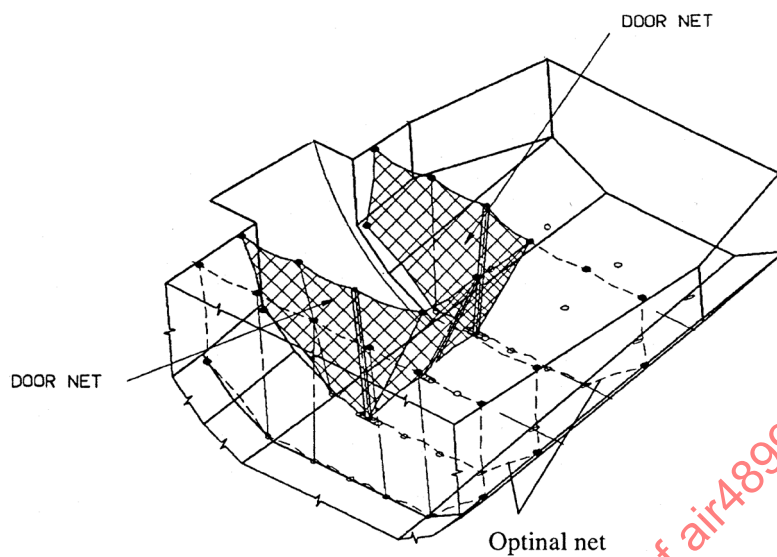
Tapered Cargo Compartment Design Example
