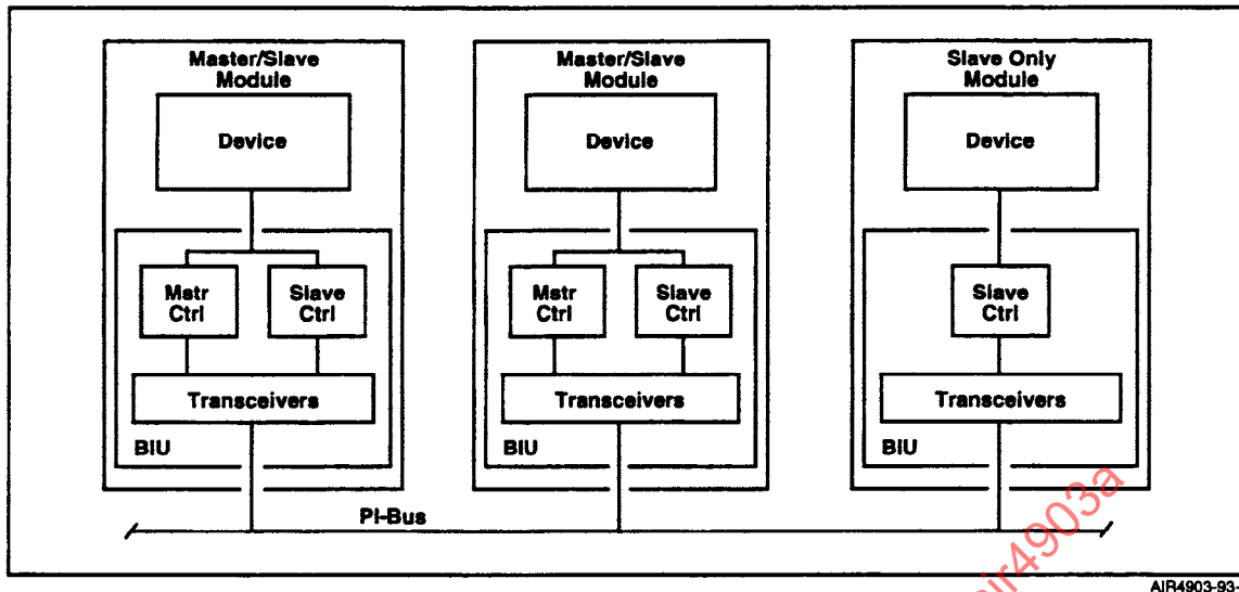
FIGURE 2 - High Level View of Pi-Bus
