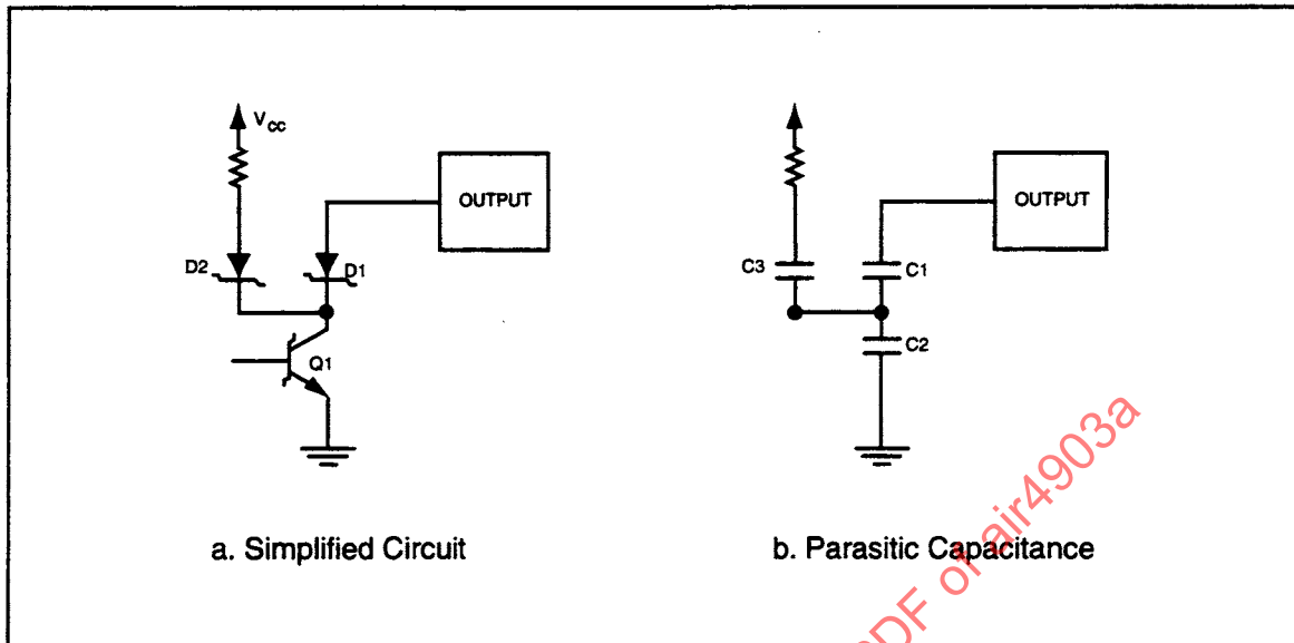
FIGURE 15 - Pi-Bus Driver Output
