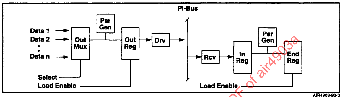
FIGURE 8 - Data and Control Flow for a Pi-Bus
