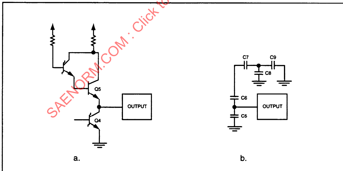
FIGURE 16 - Capacitance Loading
