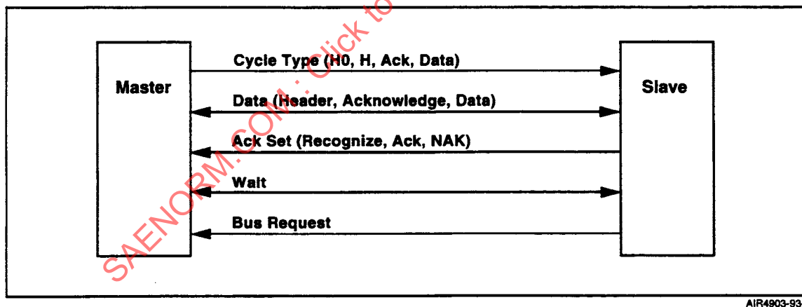
FIGURE 7 - Buses Used for Pi-Bus Messages
