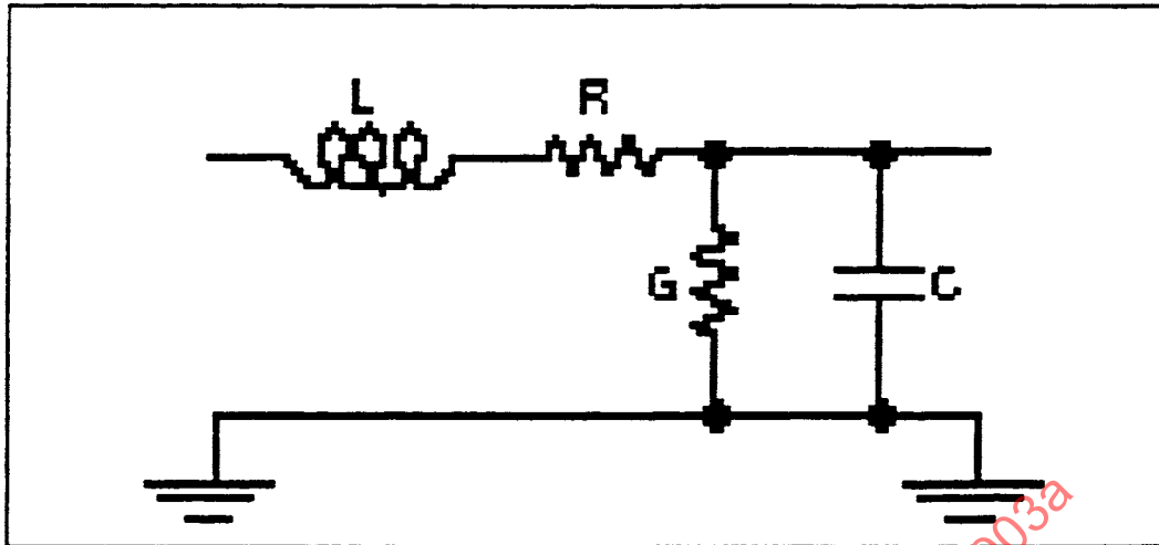
FIGURE 13 Simple Transmission Line Model
