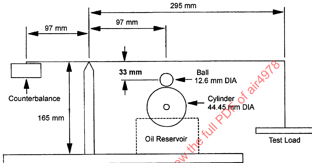
FIGURE B1 - Rolls-Royce Tribology Evaluator
