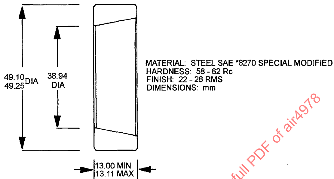
FIGURE B2 - RRTE Test Cylinder
