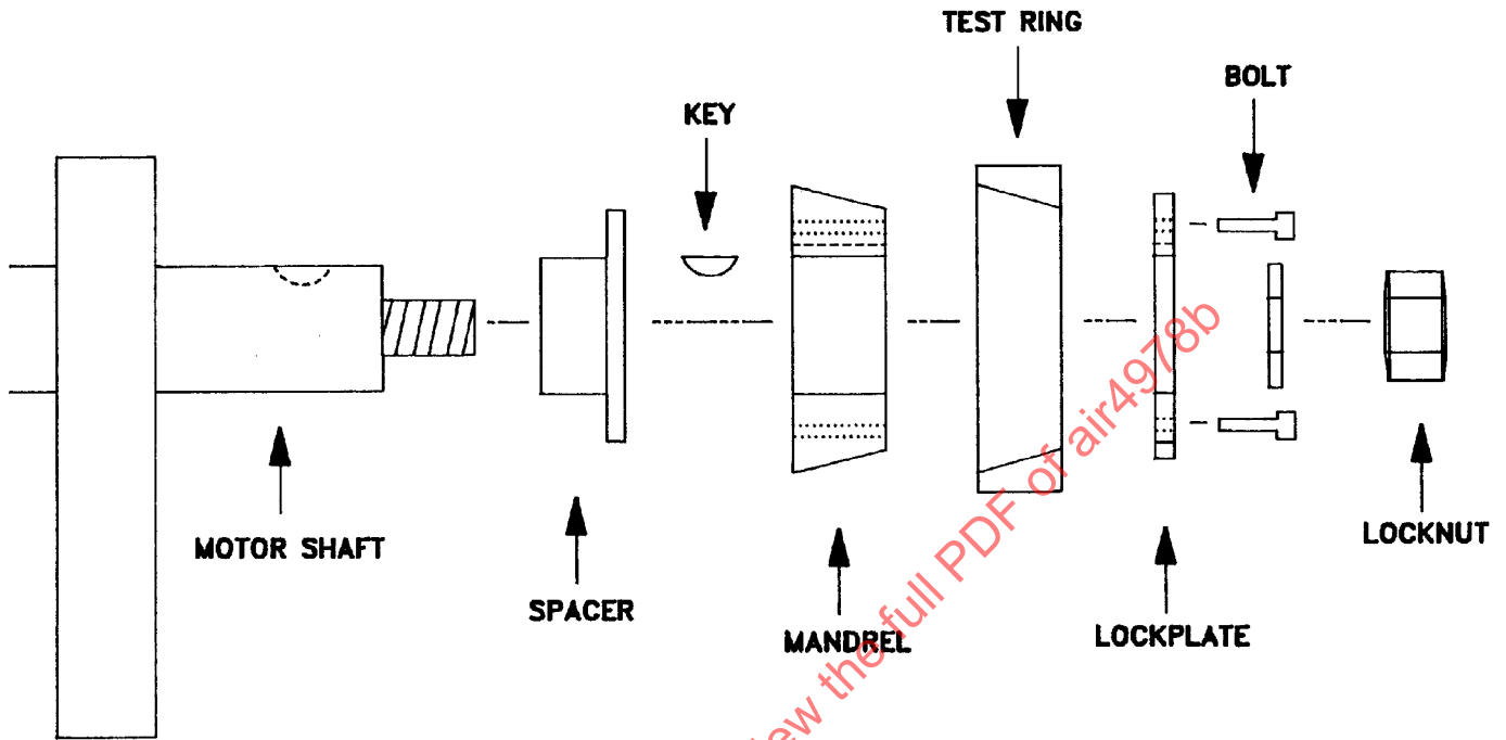
FIGURE B5 - Test Ring and Mandrel Assembly
