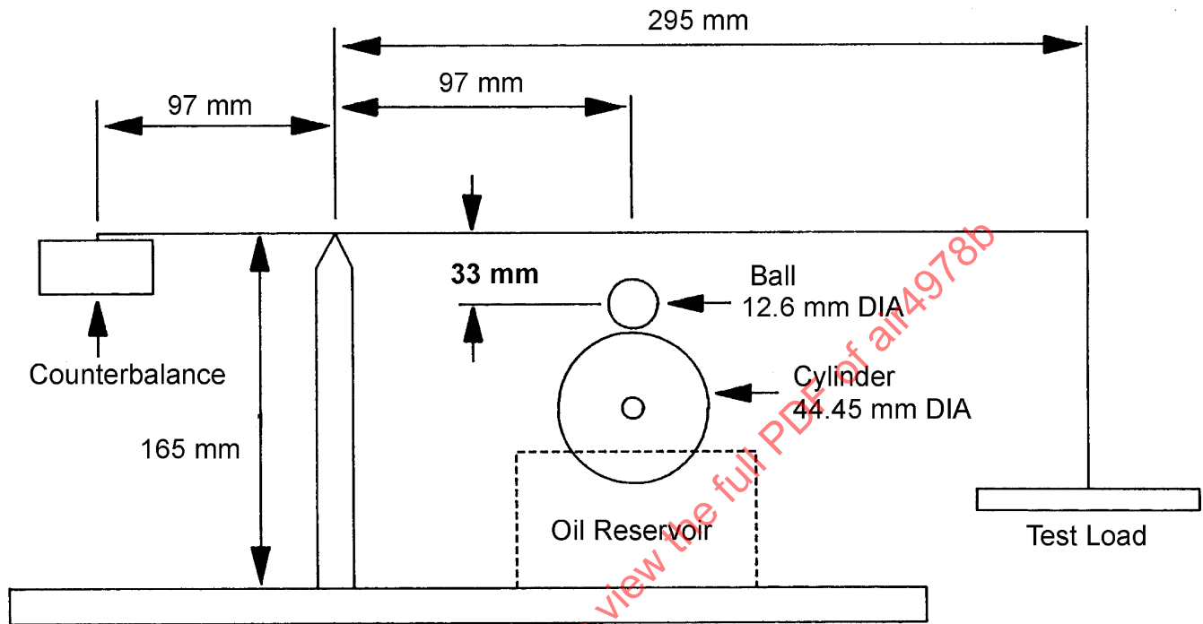
FIGURE B1 Rolls-Royce Tribology Evaluator
