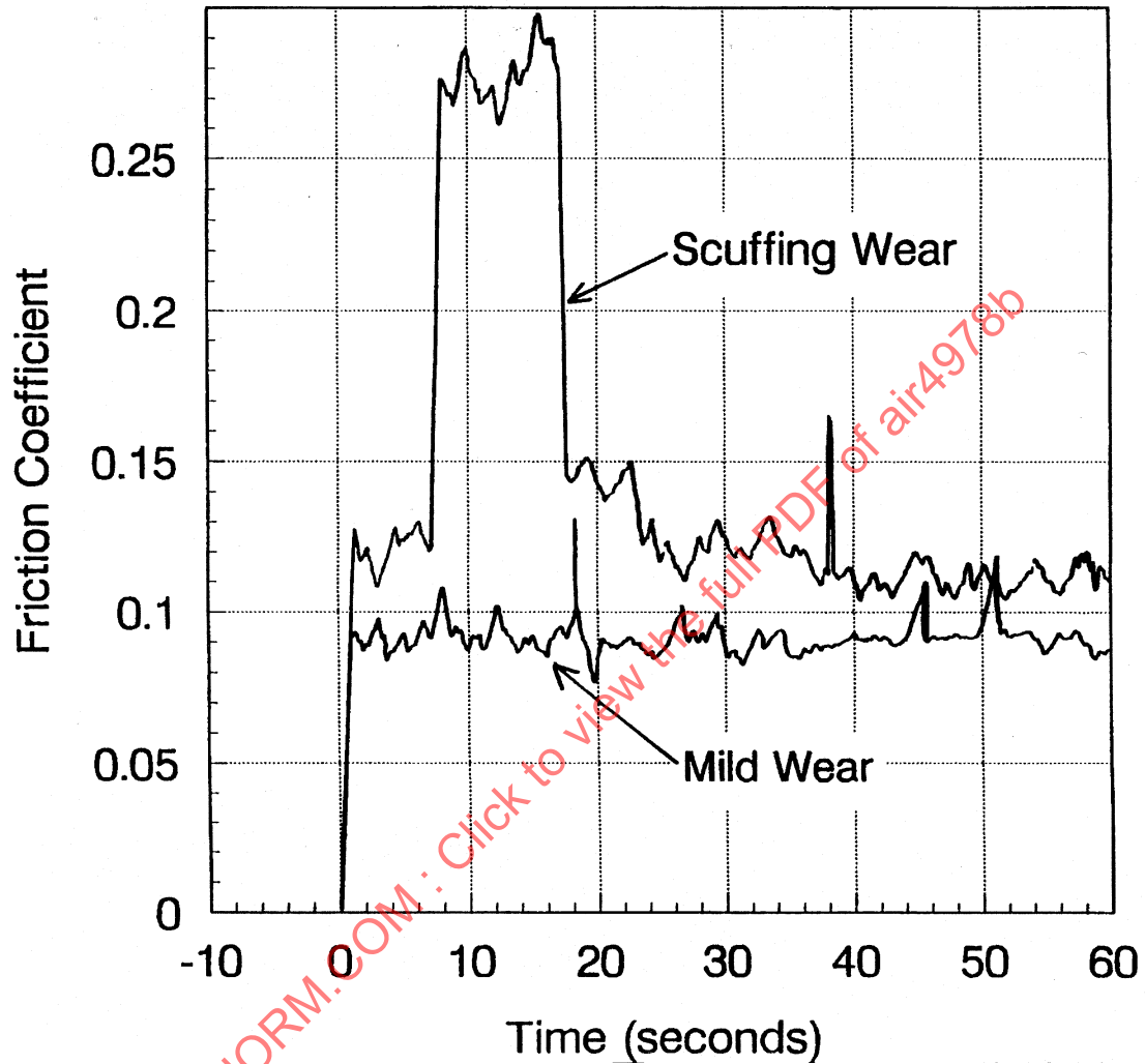
FIGURE C4 - Typical Friction Coefficients Obtained During Load Wear Tests, Calculated from Friction Trace Recording
