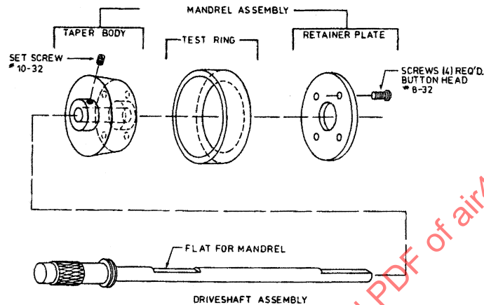
FIGURE C3 - Ring and Mandrel Assembly (Cylinder)
