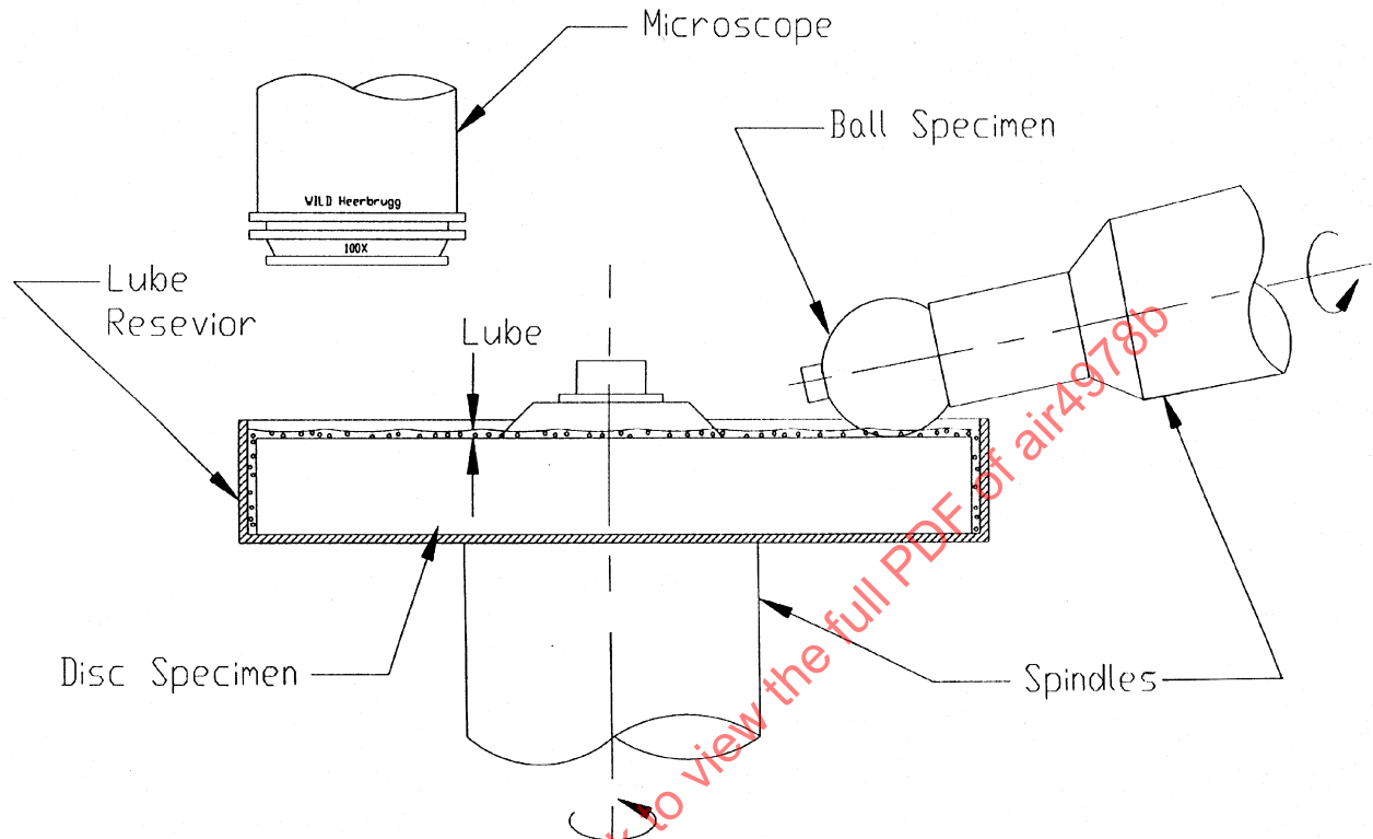
FIGURE D1 - WAM3 Test Specimens for Economical Load Screening Test
