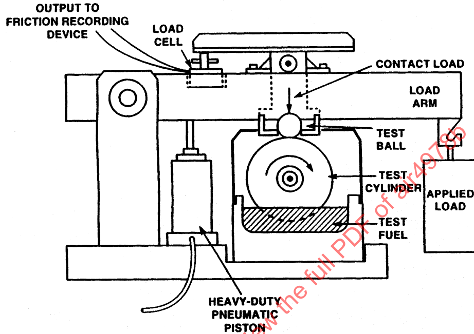
FIGURE C2 - Schematic Diagram of the Gear Oil Scuff Test (GOST) Apparatus, Not Including Instrumentation
