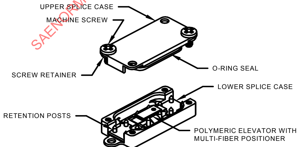
FIGURE 63 - Exploded Isometric View of Mechanical Splice Assembly
