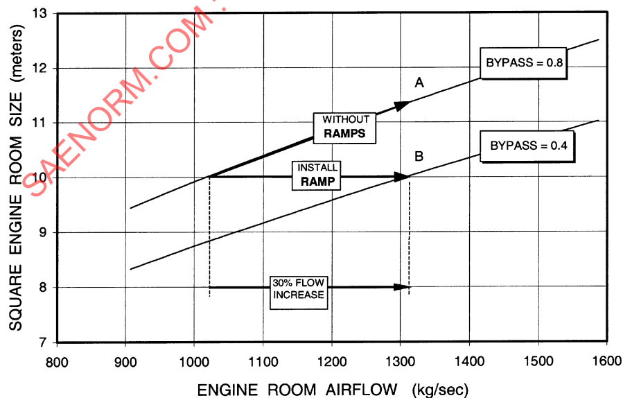
FIGURE 3 - Engine Airflow Versus Test Cell Size V_{FC} = 15.24 \text{ m/s (50 ft/s)}
