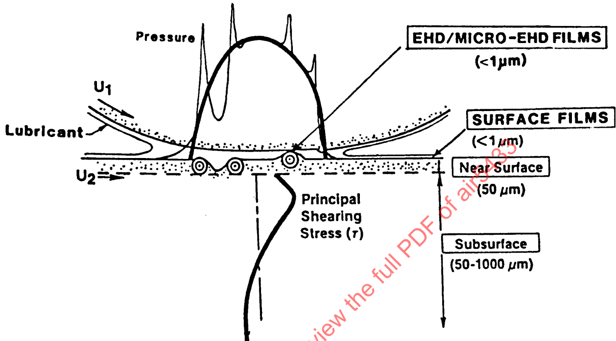
FIGURE 1 - Structural Elements of a Lubricated Contact
