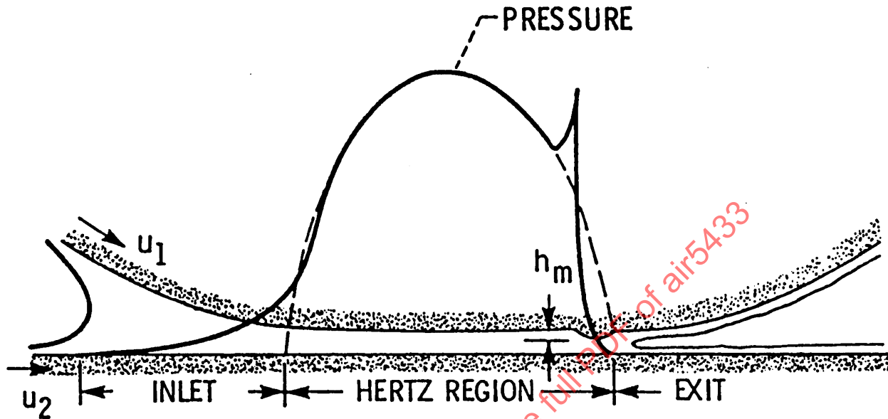
FIGURE 2 - EHD Lubrication
