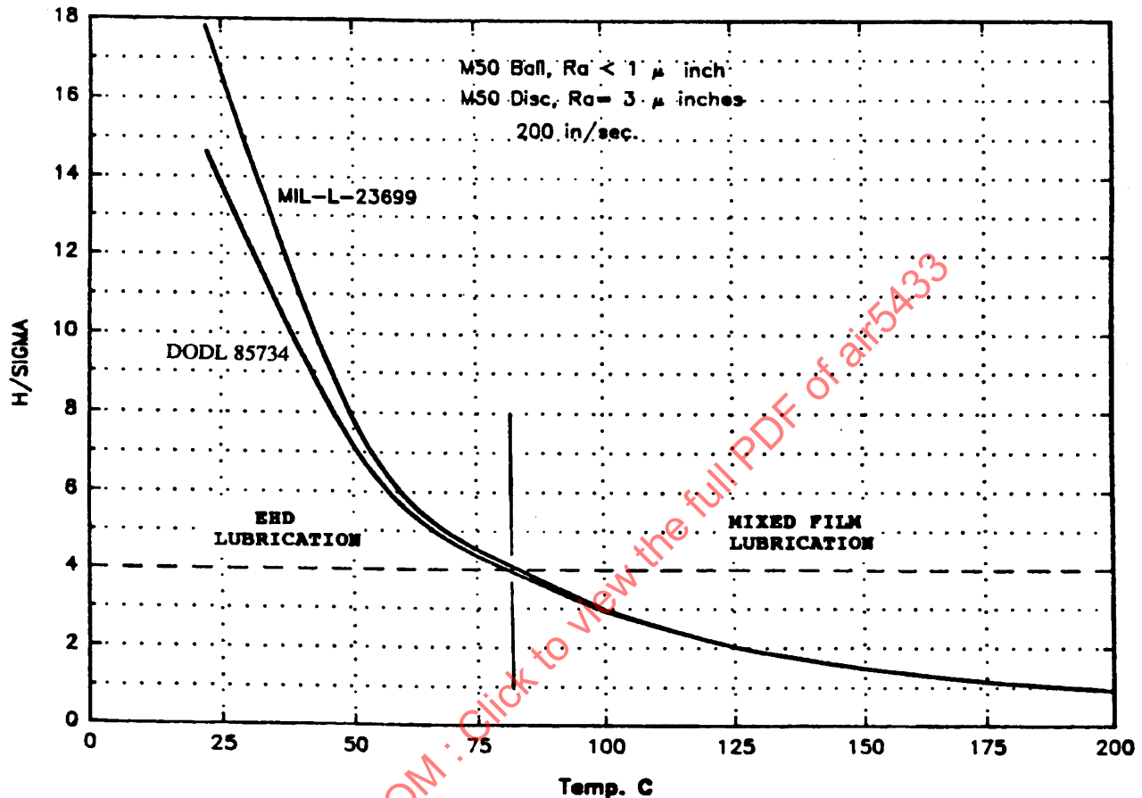
FIGURE 6 - Film Thickness to Surface Roughness Ratio Versus Temperature
