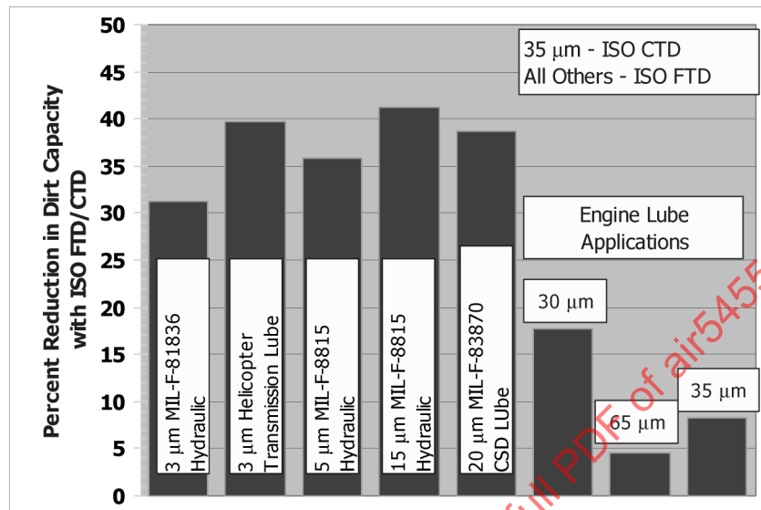
FIGURE 9 - Percent Reduction in 'Slug Load' Dirt Capacity With ISO FTD/CTD Contaminant, Compared to ACFTD/ACCTD Contaminant
