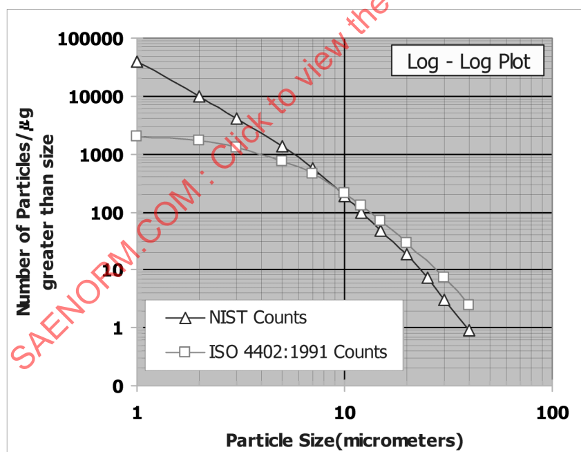
FIGURE 3 - Particle Size Versus Number Distribution of ISO MTD - ISO 4402 Versus NIST
