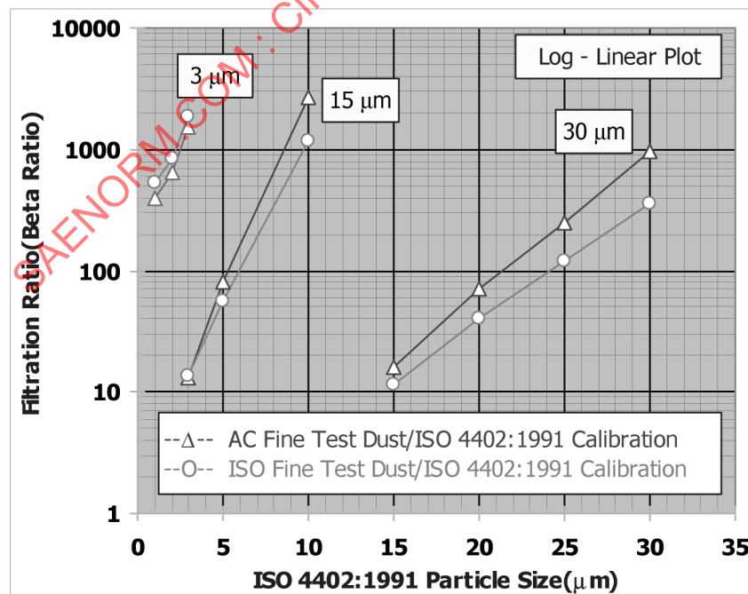
FIGURE 5 - Comparison of Multipass Beta Ratios - ACFTD Versus ISO FTD
