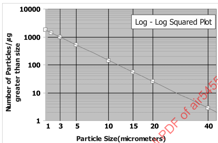
FIGURE 1 - AC Fine Test Dust Size Distribution Based on Longest Chord Dimension
