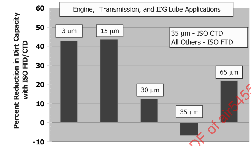
FIGURE 10 - Percent Reduction in Continuous Ingression Dirt Capacity With ISO FTD/CTD Contaminant, Compared to ACFTD/ACCTD Contaminant
