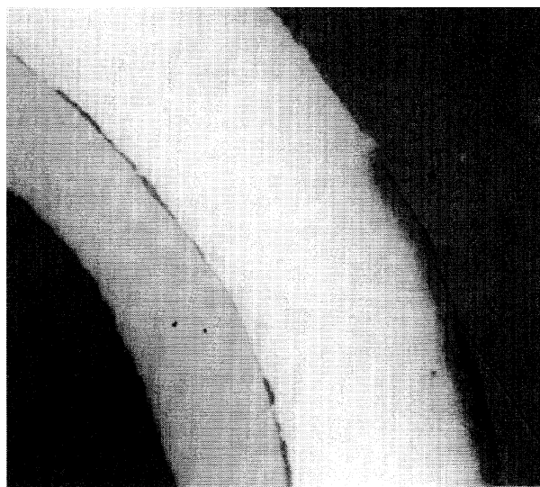
FIGURE 3 - Optical Micrograph of Cross-Sectioned XL-ETFE Wire Marked With Frequency Tripled Nd-YAG Solid State UV Laser
