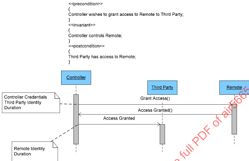
FIGURE 8 - SCENARIO GRANT ACCESS
