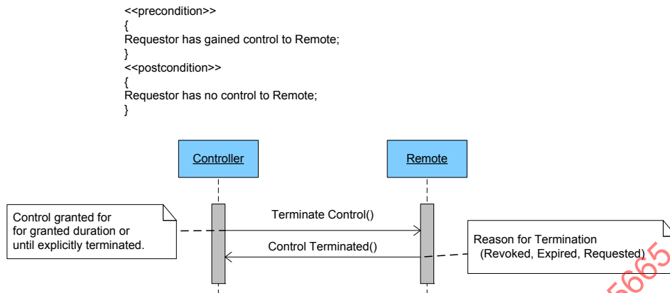
FIGURE 12 - SCENARIO TERMINATE CONTROL
