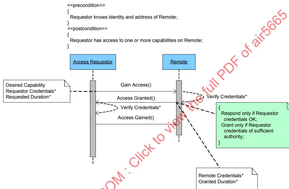
FIGURE 7 - SCENARIO GAIN ACCESS
