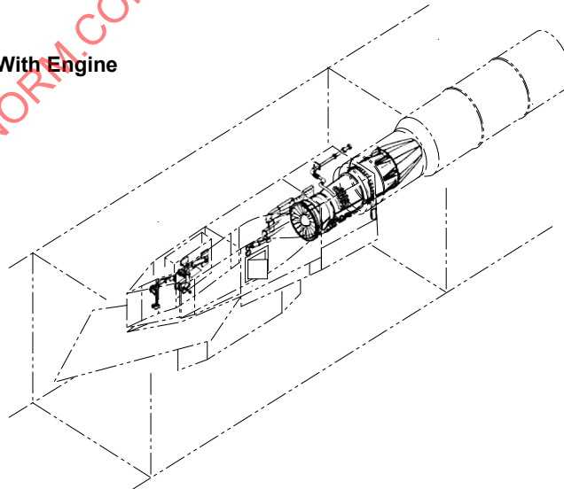
FIGURE 27 - DETAILS OF B-1A INLET WIND TUNNEL MODELS
