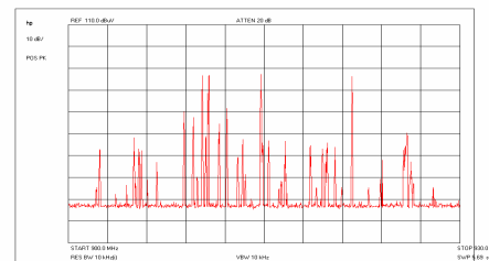
FIGURE 12B - HORIZONTAL POLARITY
