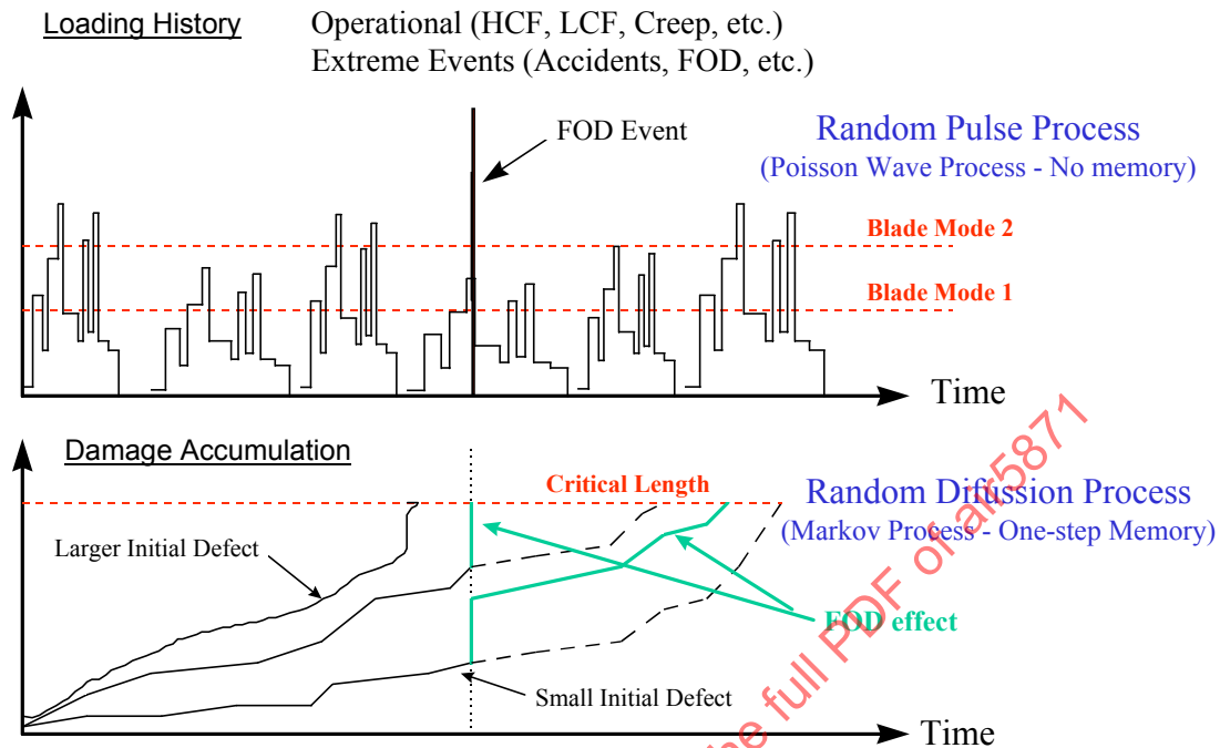
FIGURE 6 - MISSION ENVIRONMENT AND DAMAGE ACCUMULATION PROCESS
