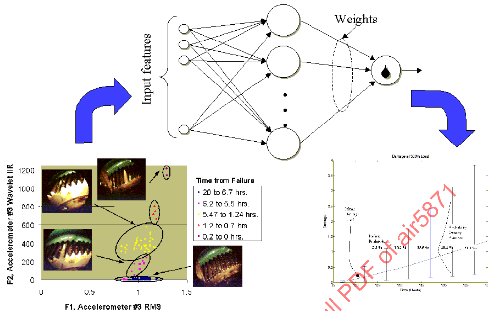
FIGURE 3 - FEATURE/AI-BASED PROGNOSTICS
