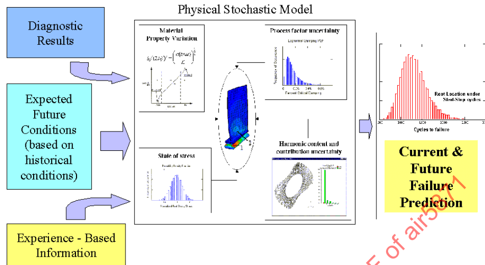
FIGURE 5 - PHYSICS-BASED PROGNOSTICS
