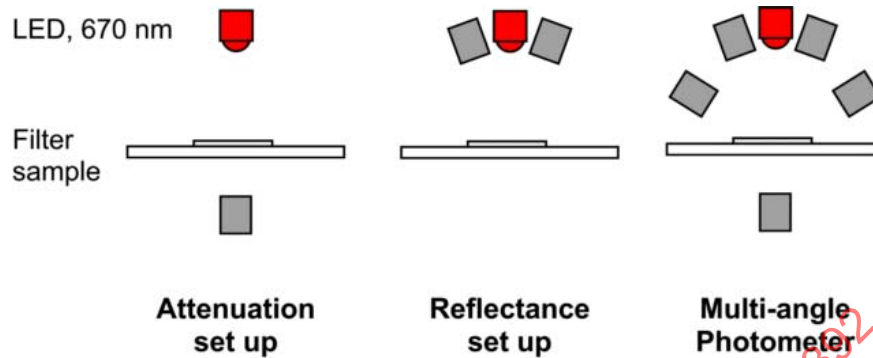
FIGURE 4 - Schematic Set Up for Attenuation and Reflectivity Measurements Compared to the Multi-angle Absorption Photometer (MAAP) Set Up (Reference 30)
