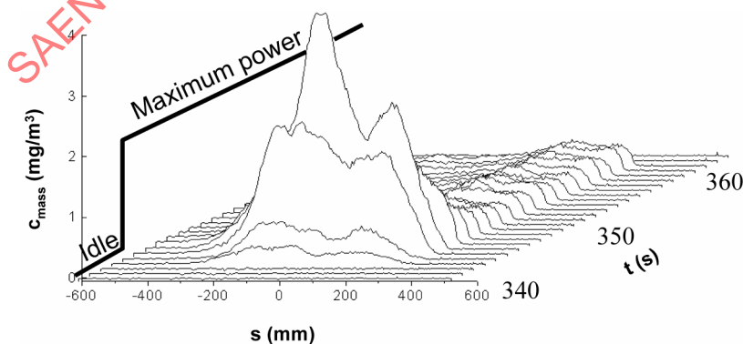
FIGURE 9 - Particle Mass Profiles in an Engine Exhaust During a Transition in Throttle Setting from Idle to Maximum Power
