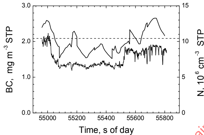
FIGURE 5 - Carbon mass concentration measured with the Multi-Angle Absorption Photometer (solid line) and with the Smoke Number method (dashed line) in an aircraft engine combustor exhaust; the lower full line indicates the number concentration of combustion particles (Reference 33)
