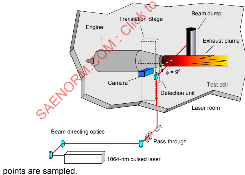
FIGURE 7 - LII System Mounted in an Engine Test Cell for Measuring Particle Mass Concentration in Exhausts
