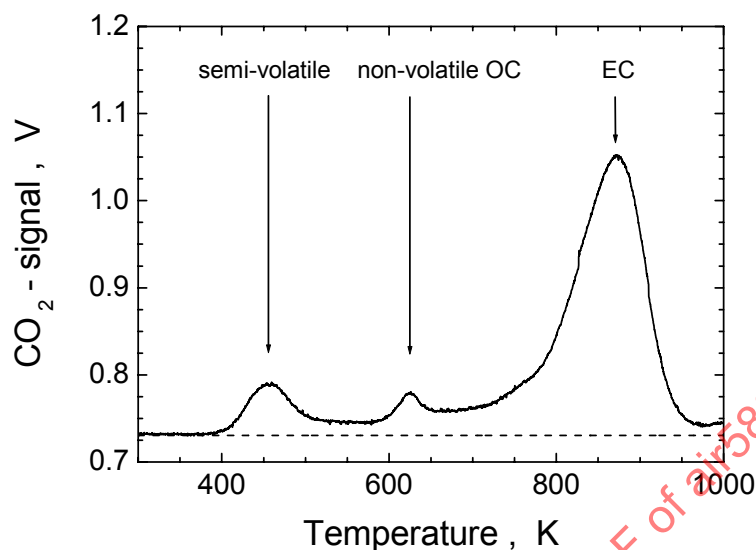
FIGURE 1 - Evolving \text{CO}_2 as a function of the sample heating temperature for a combustor particulate matter sample; semi-volatile OC oxidizes at 450 K, nonvolatile OC at 600 K, and elemental carbon above 700 K (Reference 34)
